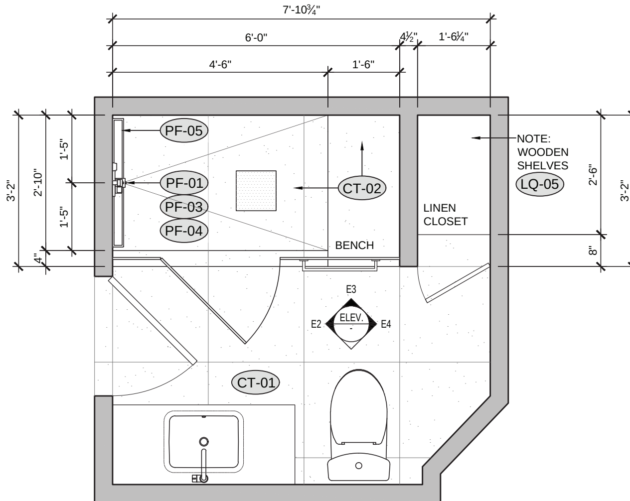
P1 | DETAIL PLAN 1/2" = 1'-0"
