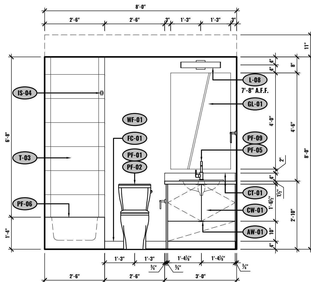
D ELEVATION - BATHROOM UNIT #604 1/2"=1'-0"
