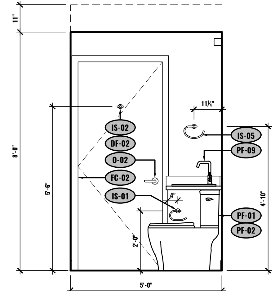
I ELEVATION - BATHROOM UNIT #2-503 1/2"=1'-0"
