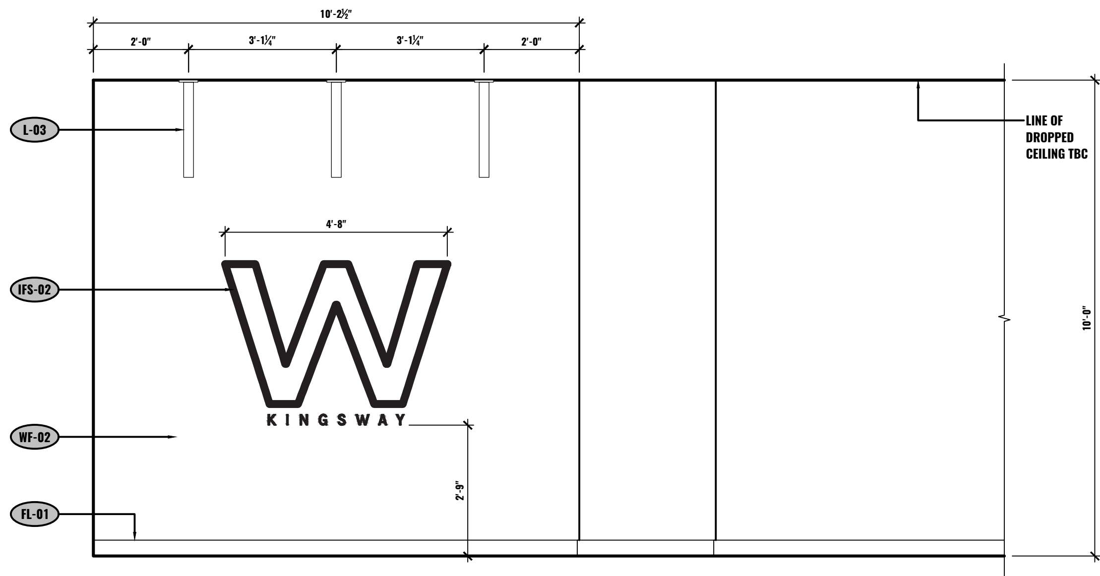
A ELEVATION - ELEVATOR LOBBY LEVEL 1 1/2"=1'-0"
