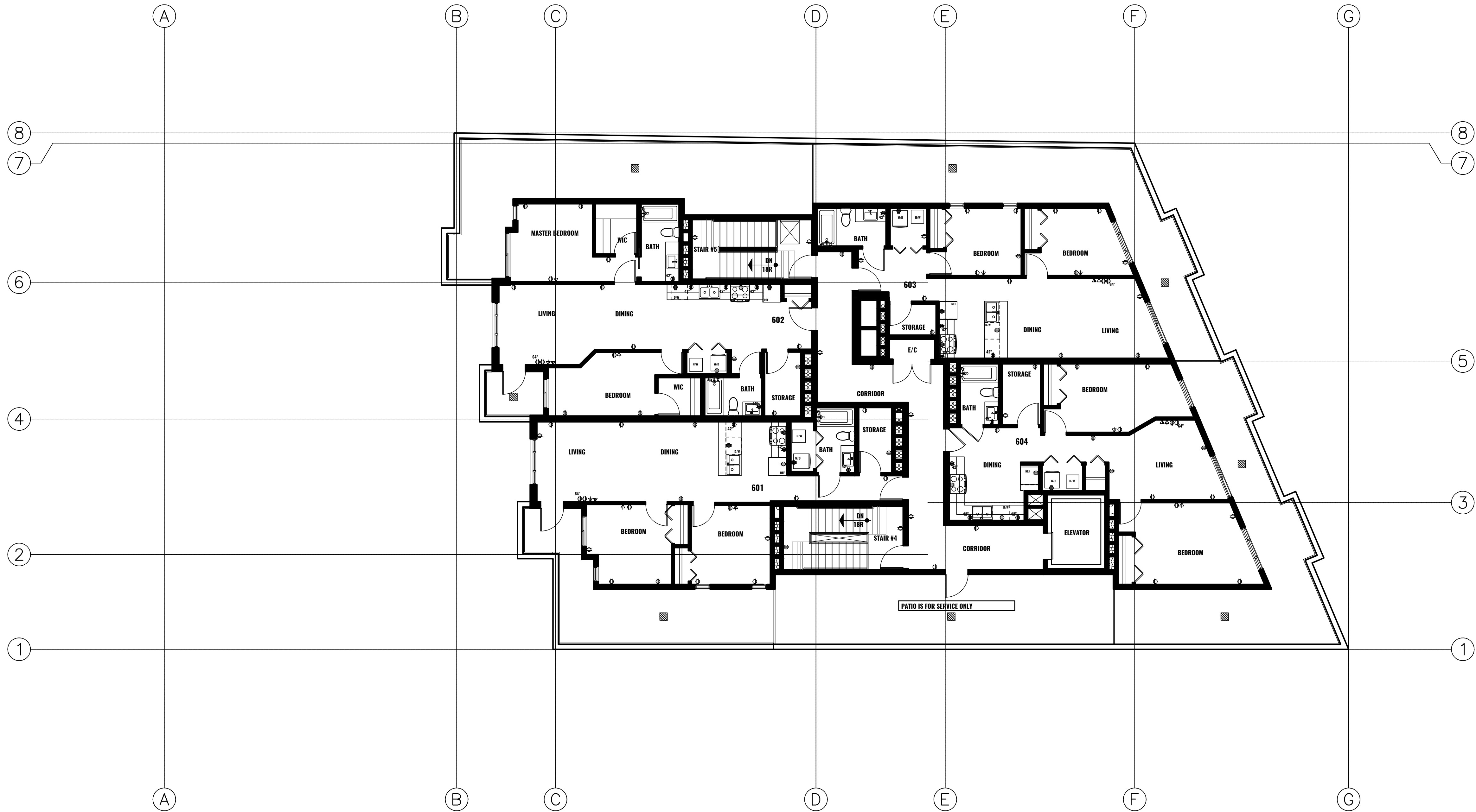
3 ELECTRICAL PLAN LEVEL 6 1/8"=1'-0"
