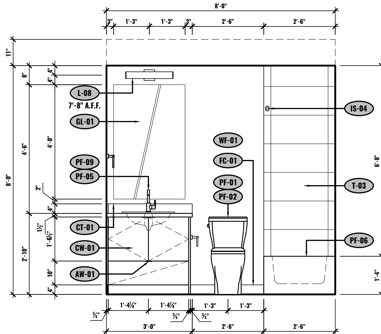
F ELEVATION - BATHROOM UNIT #2-503 1/2"=1'-0"
