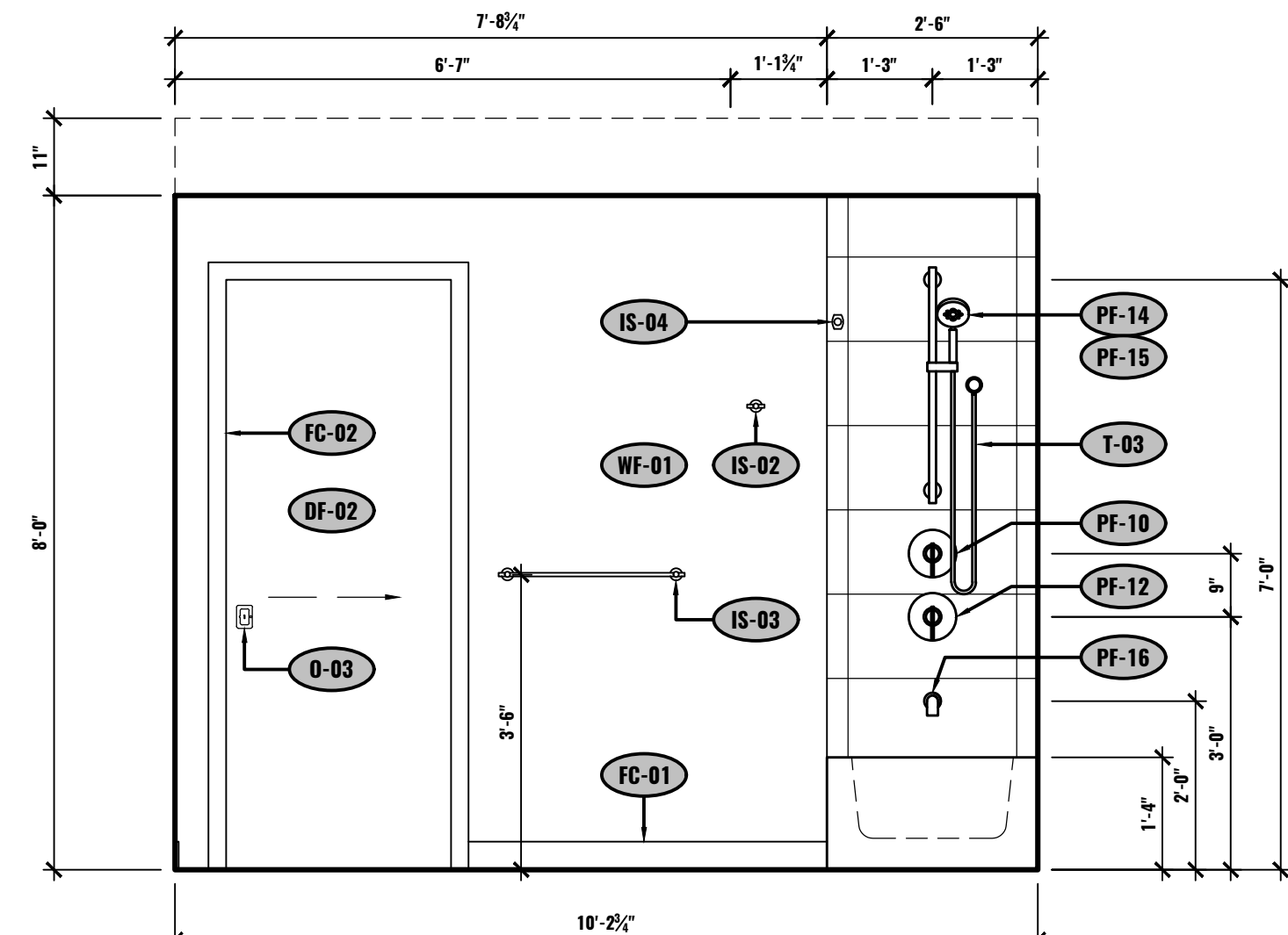
M ELEVATION - BATHROOM UNIT #602 1/2"=1'-0"
