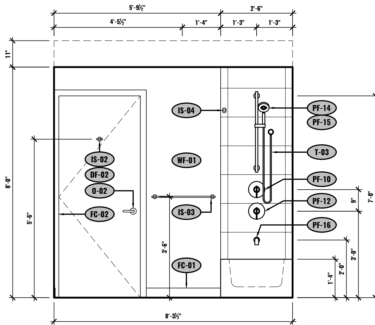
C ELEVATION - BATHROOM UNIT #2-506 1/2"=1'-0"
