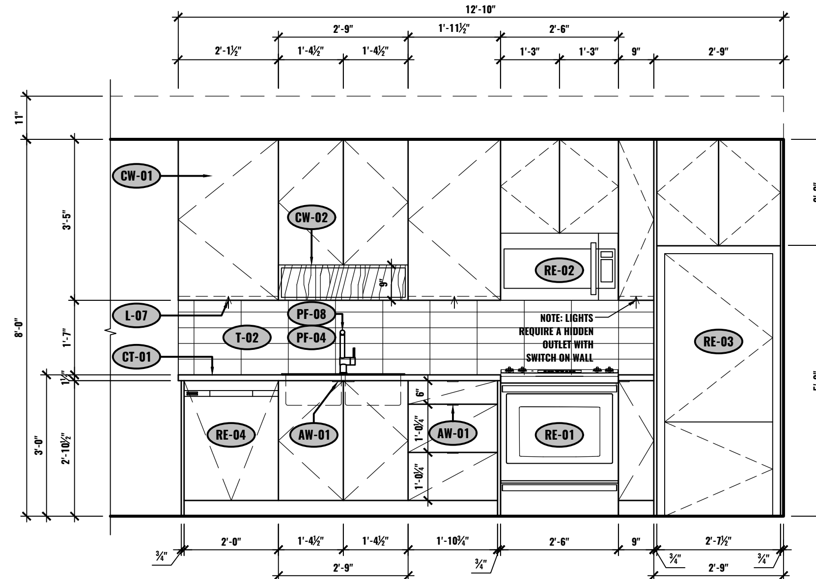
G ELEVATION - KITCHEN UNIT #2-502 1/2"=1'-0"
