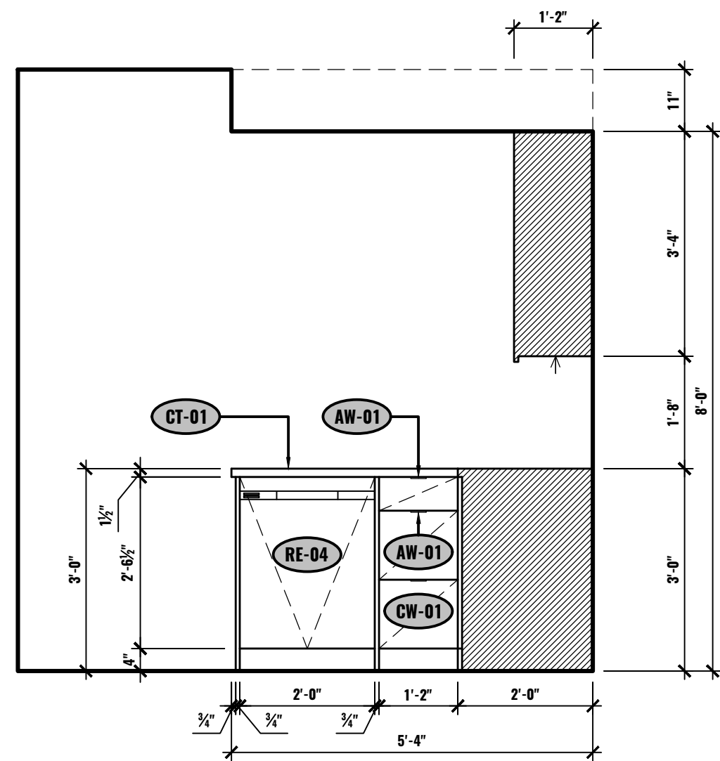
E ELEVATION - KITCHEN UNIT #2-504 1/2"=1'-0"
