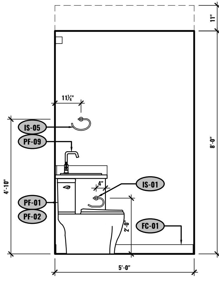
K ELEVATION - BATHROOM UNIT #2-507 1/2"=1'-0"
