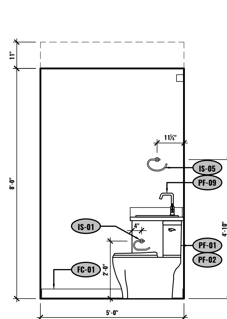
D ELEVATION - BATHROOM UNIT #2-505 1/2"=1'-0"
