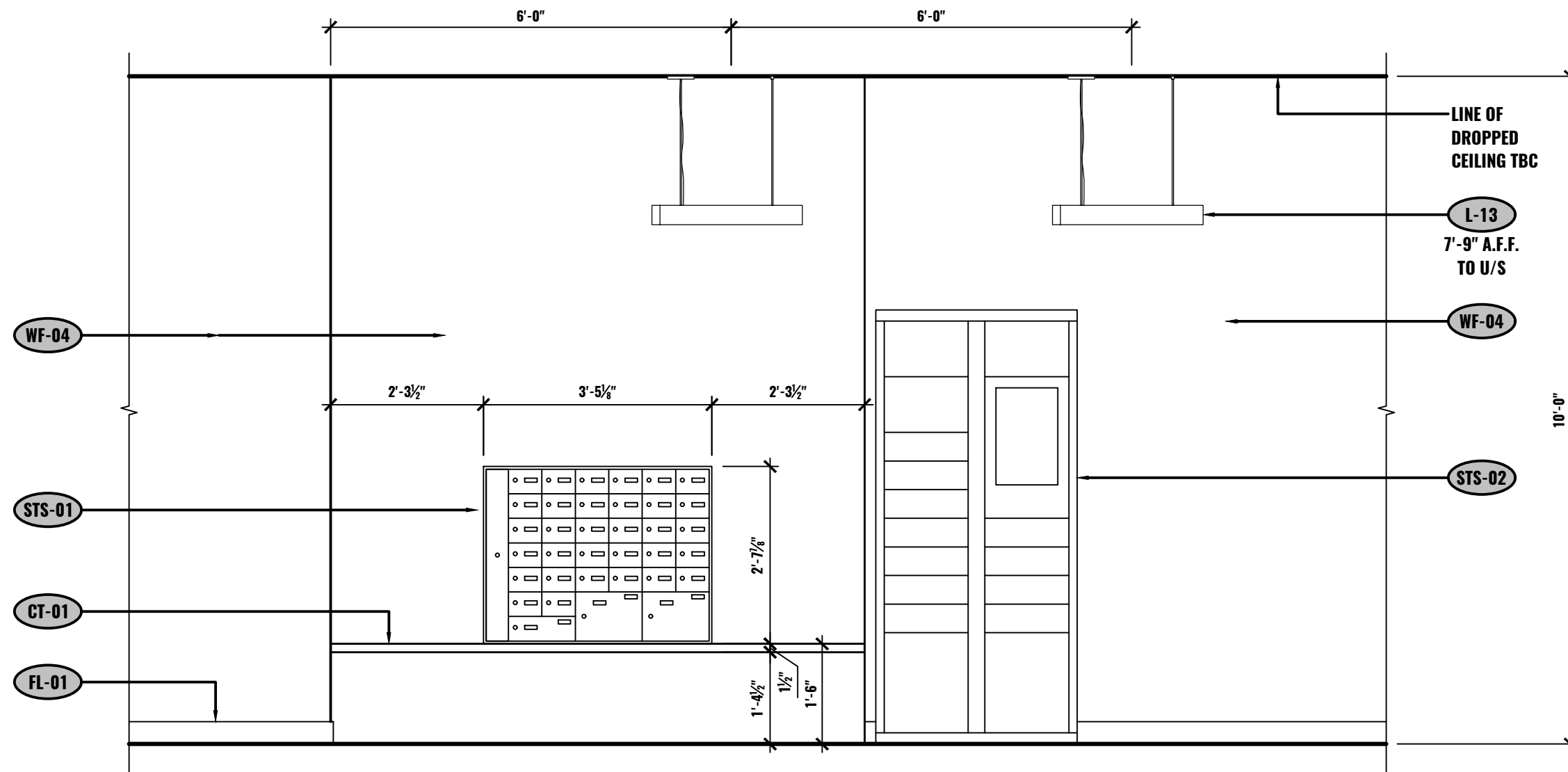
B ELEVATION - ELEVATOR LOBBY LEVEL 1 1/2"=1'-0"
