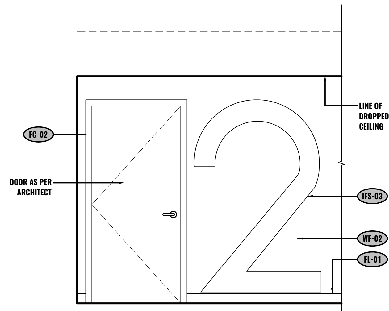
E ELEVATION - CORRIDOR STAIRWELL DOORS ALL LEVELS 1/2"=1'-0"
