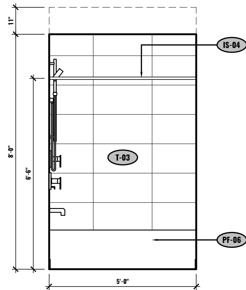
F ELEVATION - BATHROOM UNIT #601 1/2"=1'-0"
