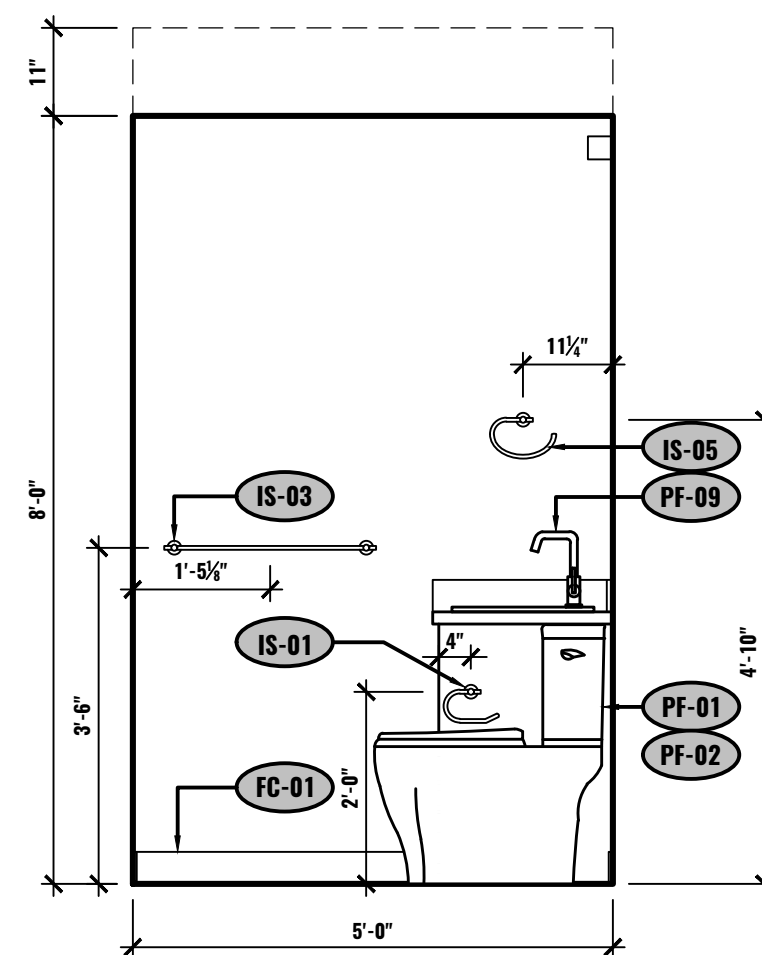
K ELEVATION - BATHROOM UNIT #2-502 1/2"=1'-0"
