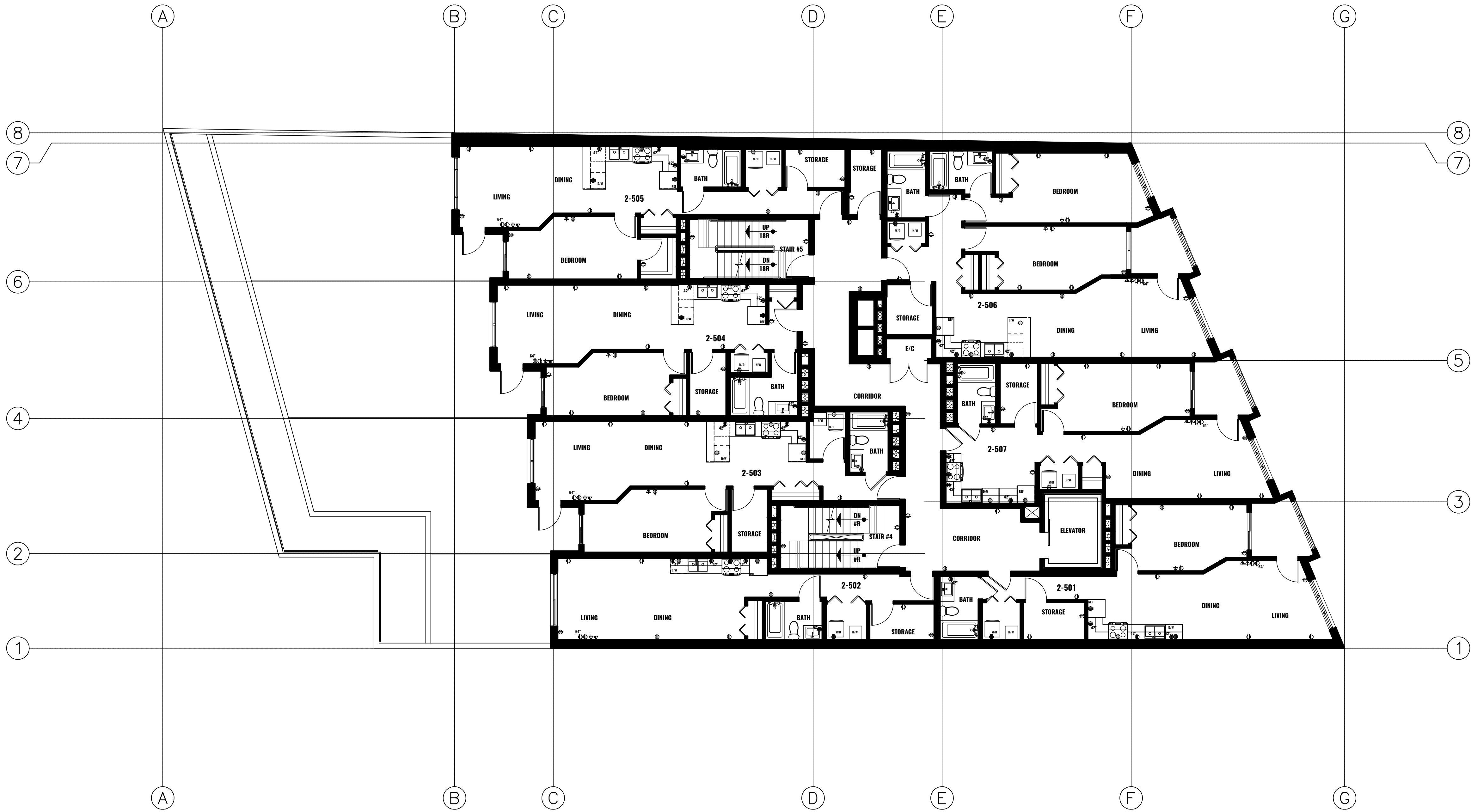
2 ELECTRICAL PLAN LEVELS 2-5 1/8"=1'-0"
