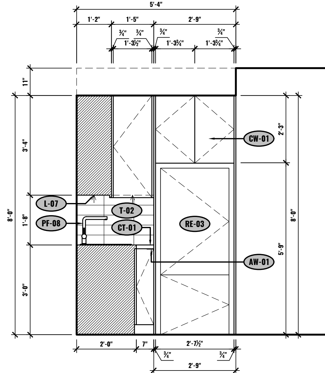
C ELEVATION - KITCHEN UNIT #2-504 1/2"=1'-0"
