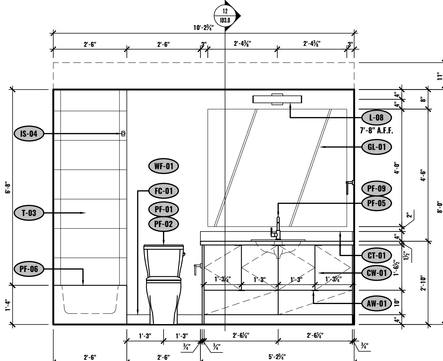
K ELEVATION - BATHROOM UNIT #602 1/2"=1'-0"
