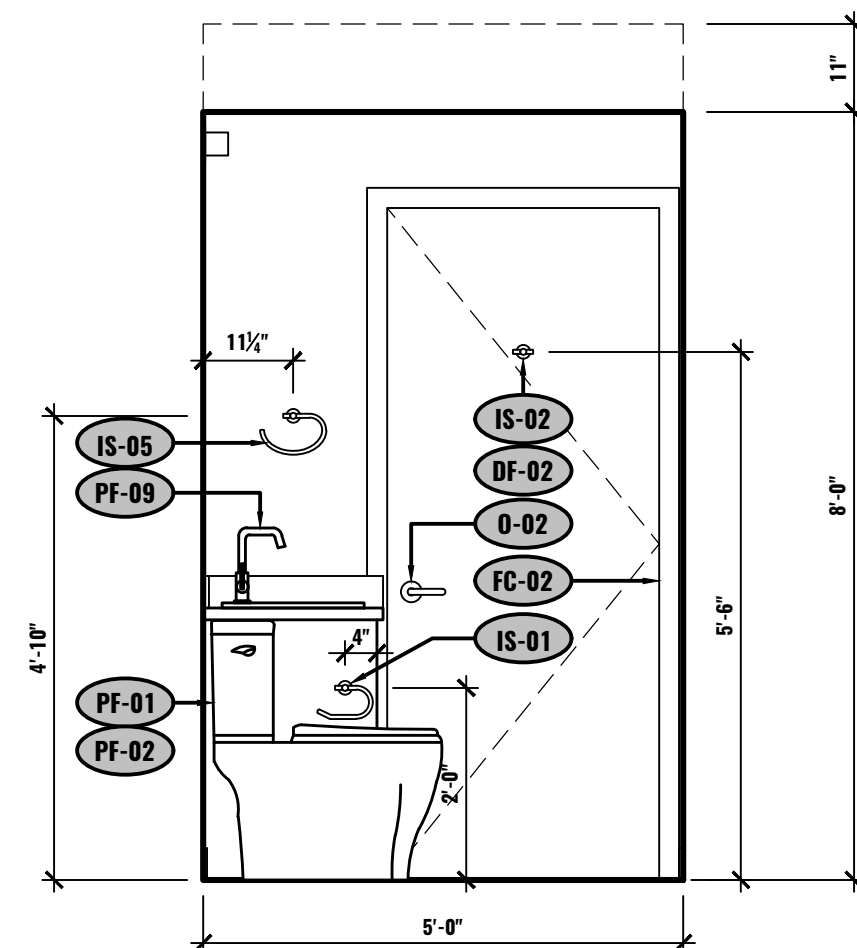
H ELEVATION - BATHROOM UNIT #601 1/2"=1'-0"
