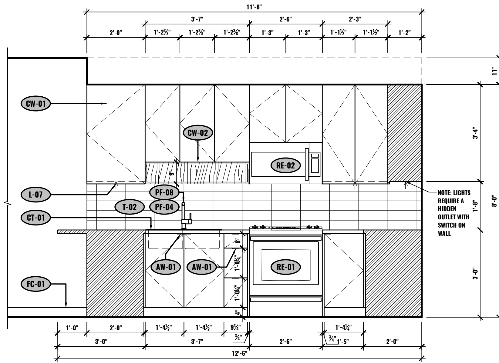
F ELEVATION - KITCHEN UNIT #2-505 1/2"=1'-0"
