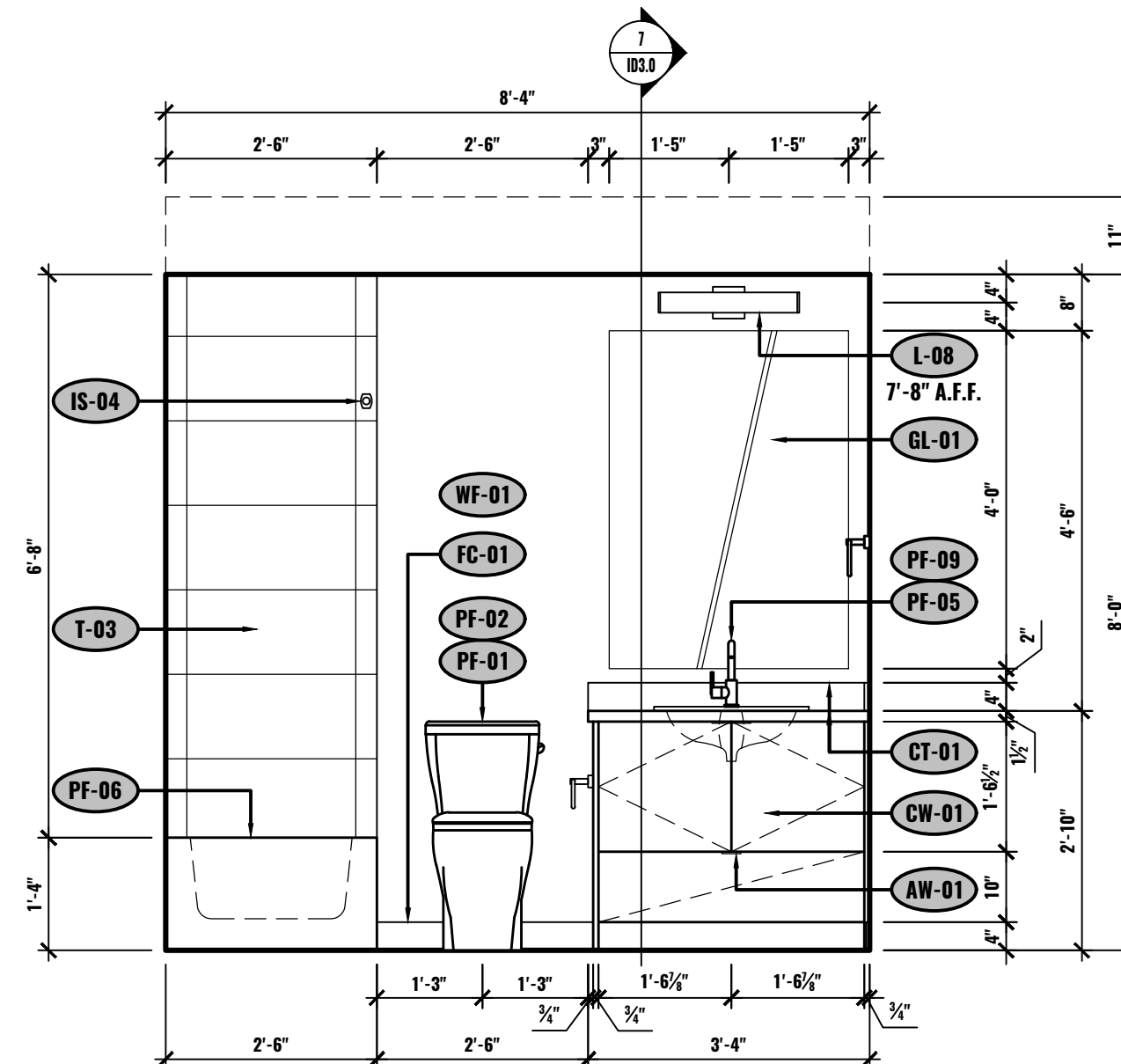
C ELEVATION - BATHROOM UNIT #2-501 1/2"=1'-0"
