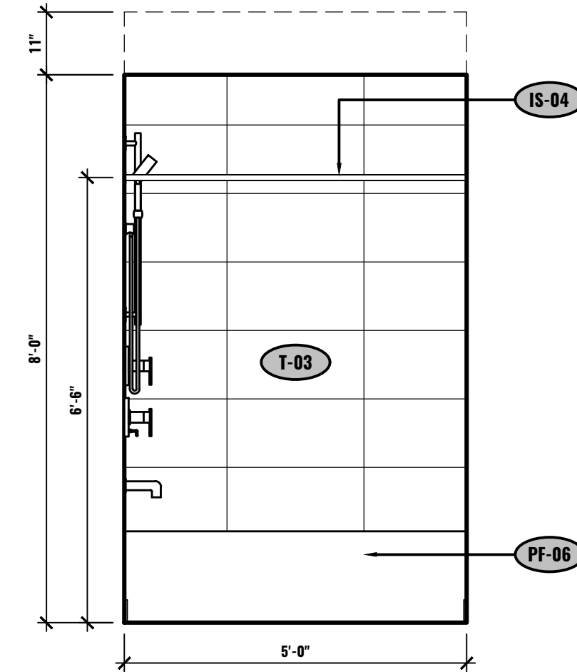
D ELEVATION - BATHROOM UNIT #2-501 1/2"=1'-0"
