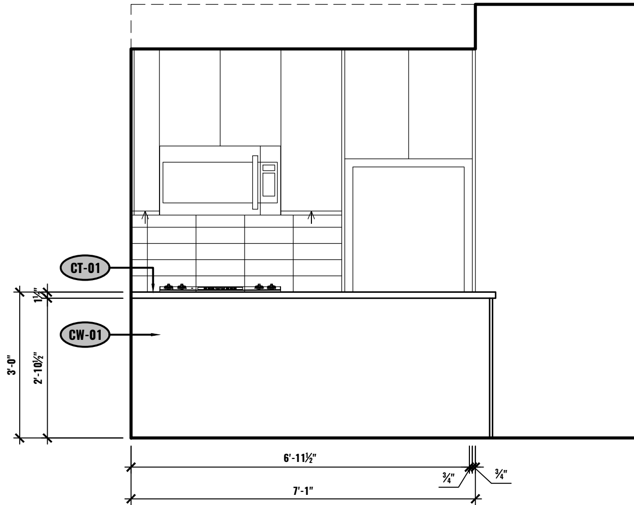
B ELEVATION - KITCHEN UNIT #601 1/2"=1'-0"
