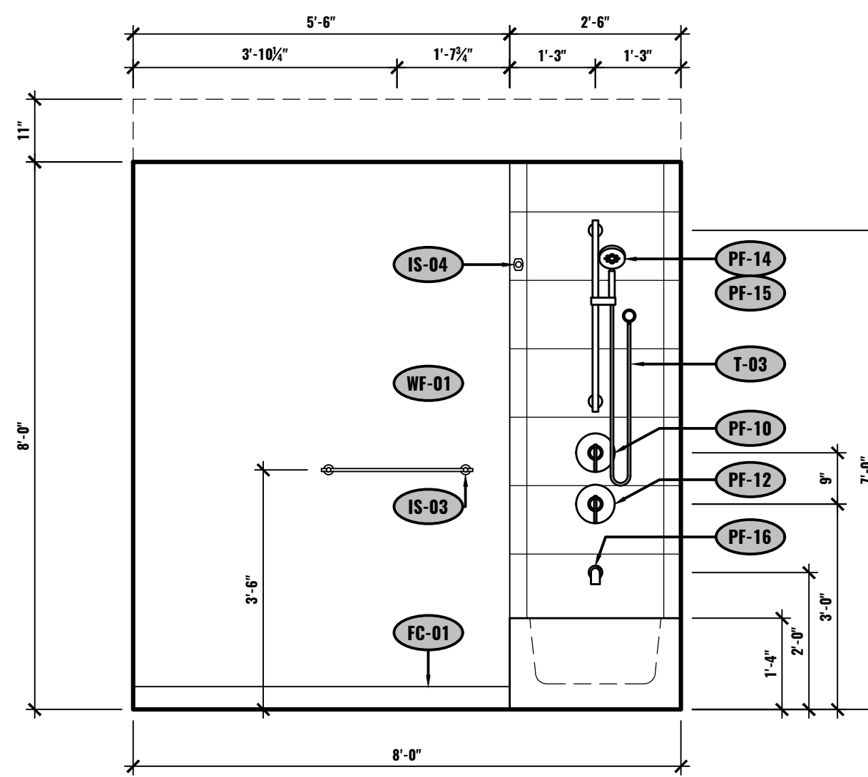
F ELEVATION - BATHROOM UNIT #604 1/2"=1'-0"
