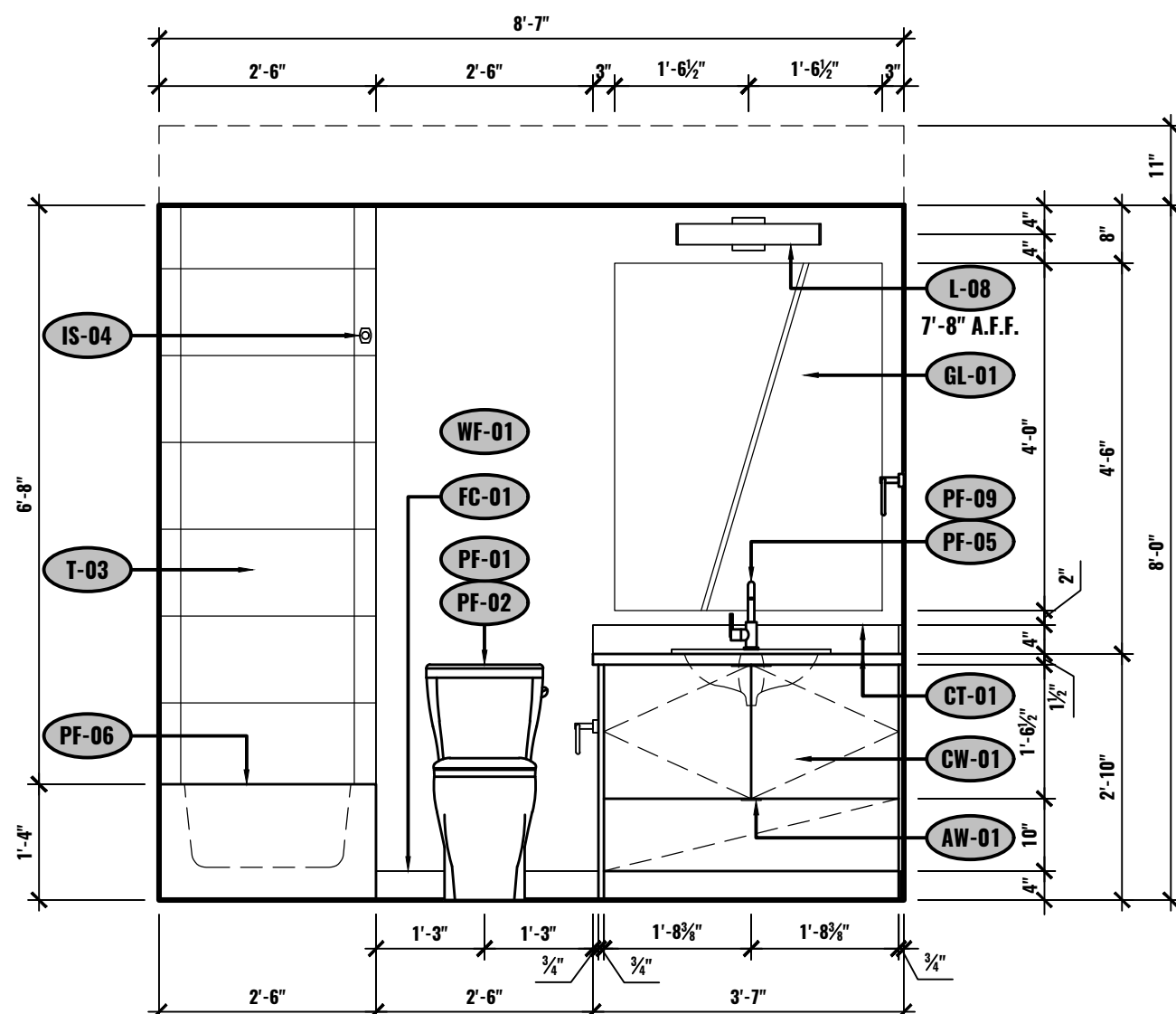
E ELEVATION - BATHROOM UNIT #601 1/2"=1'-0"
