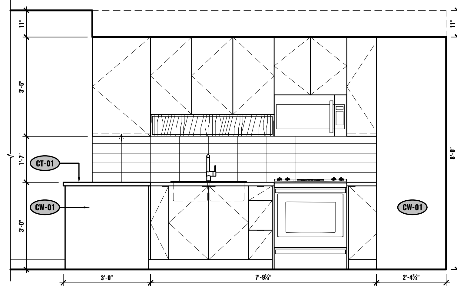
B ELEVATION - KITCHEN UNIT #2-503 1/2"=1'-0"
