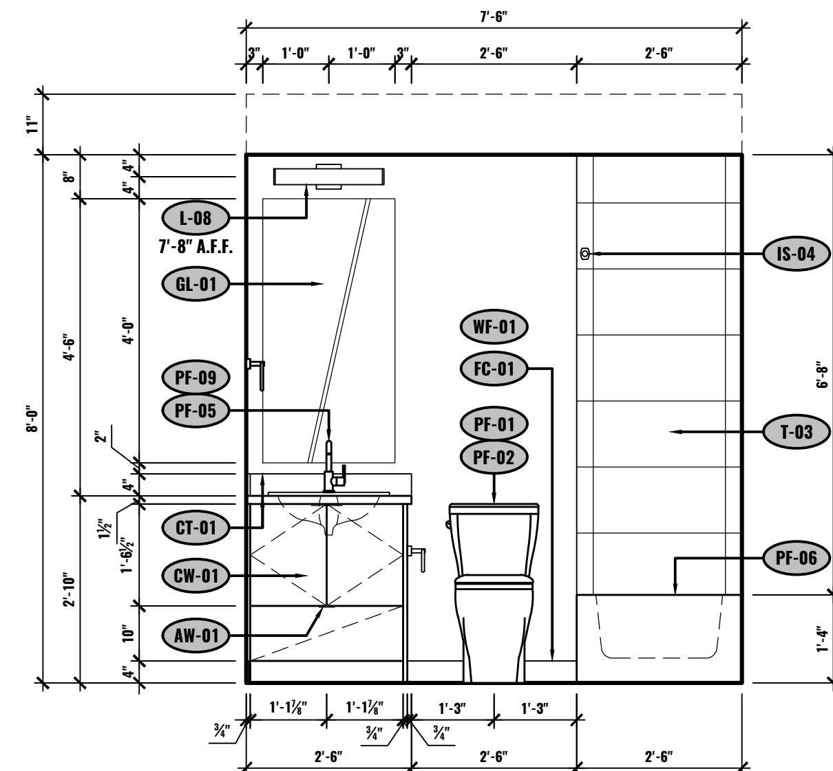
H ELEVATION - BATHROOM UNIT #2-502 1/2"=1'-0"
