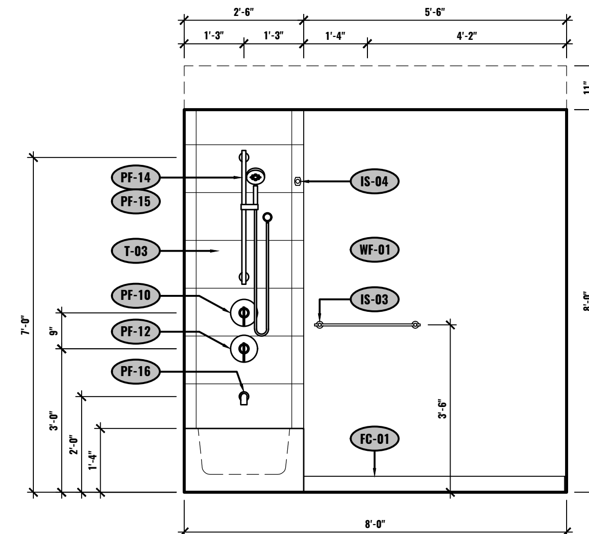
H ELEVATION - BATHROOM UNIT #2-503 1/2"=1'-0"
