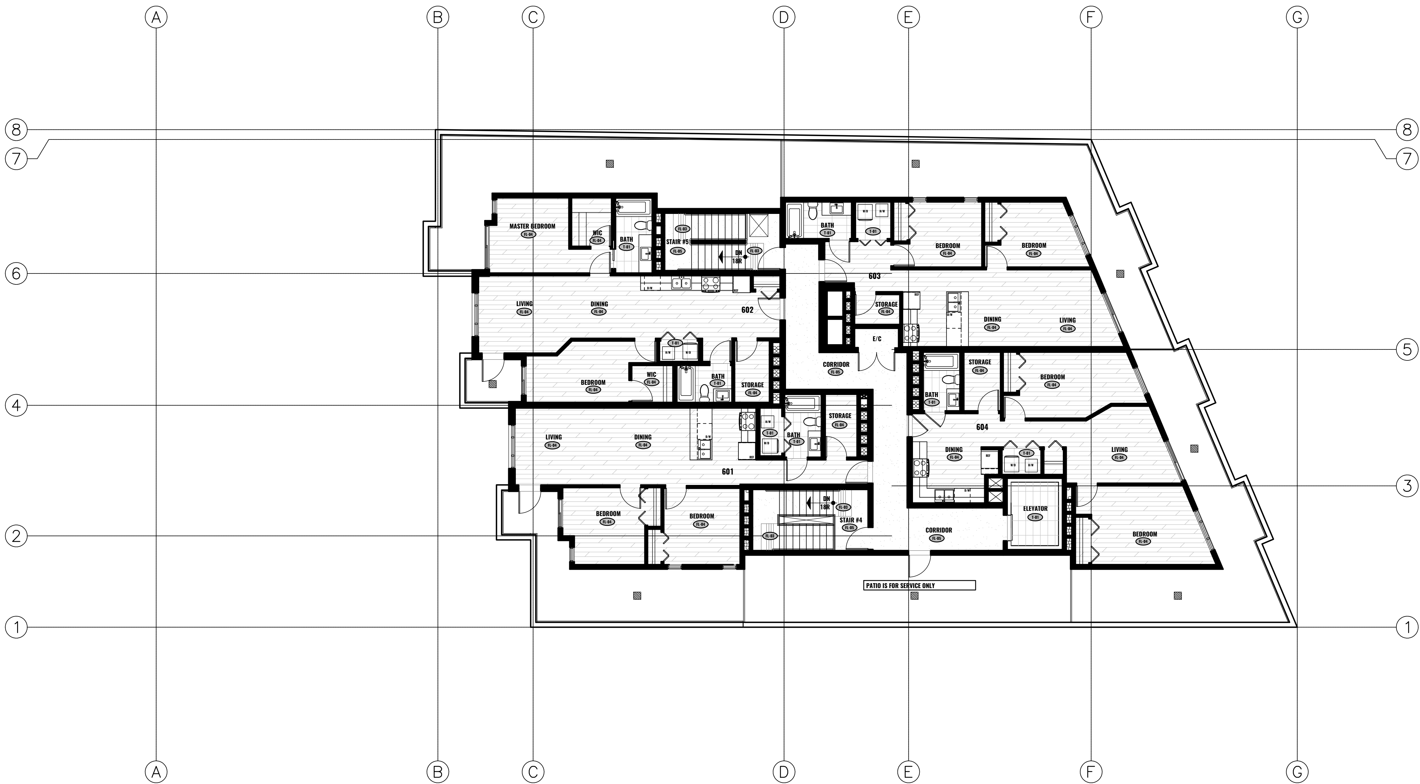
3 FINISHES PLAN LEVEL 6 1/8"=1'-0"
