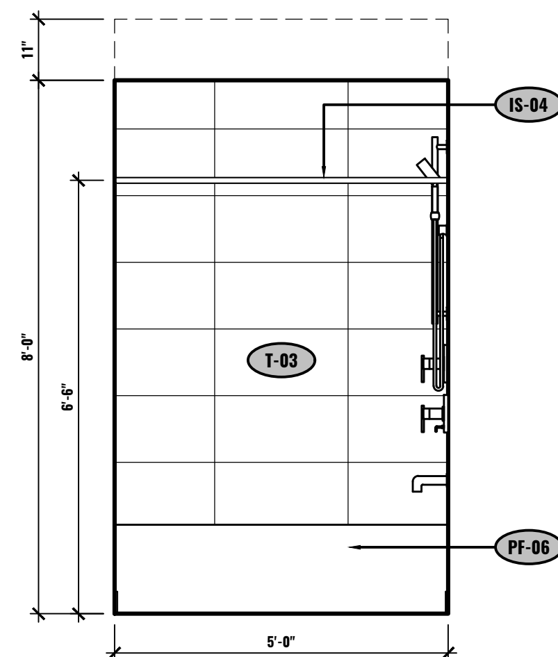
L ELEVATION - BATHROOM UNIT #2-506 1/2"=1'-0"
