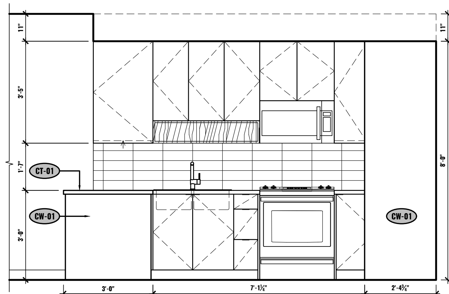
F ELEVATION - KITCHEN UNIT #2-506 1/2"=1'-0"
