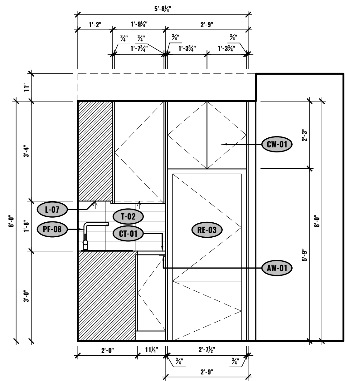
H ELEVATION - KITCHEN UNIT #2-505 1/2"=1'-0"
