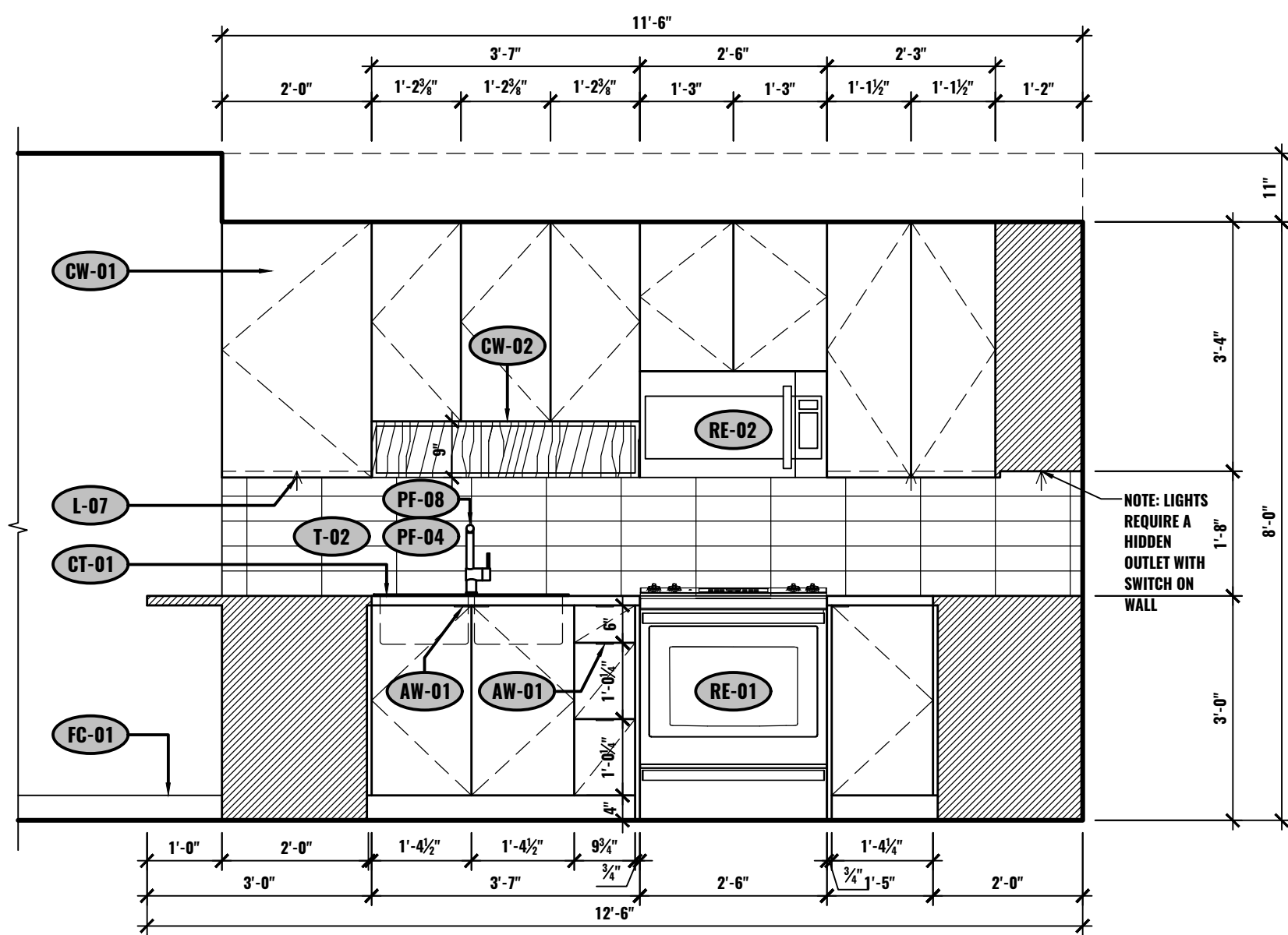
A ELEVATION - KITCHEN UNIT #2-504 1/2"=1'-0"
