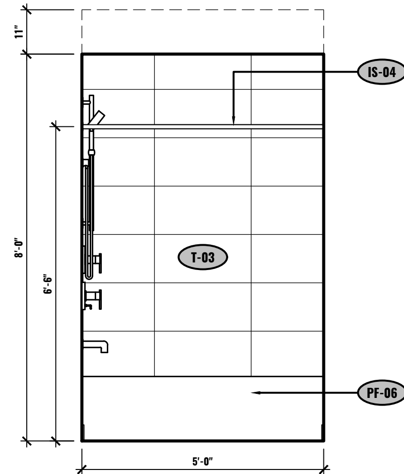
L ELEVATION - BATHROOM UNIT #603 1/2"=1'-0"
