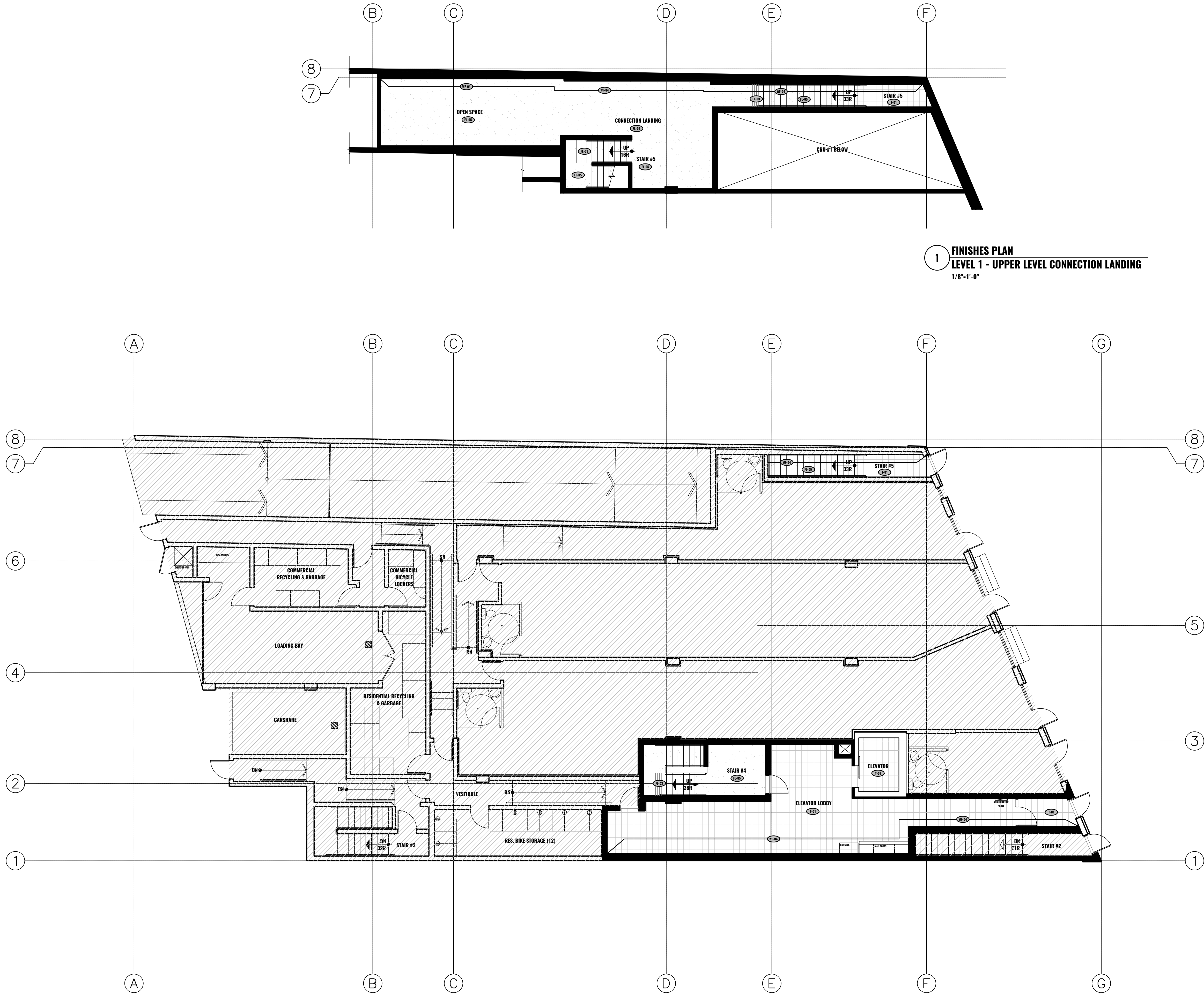
1 FINISHES PLAN LEVEL 1 1/8"=1'-0"
