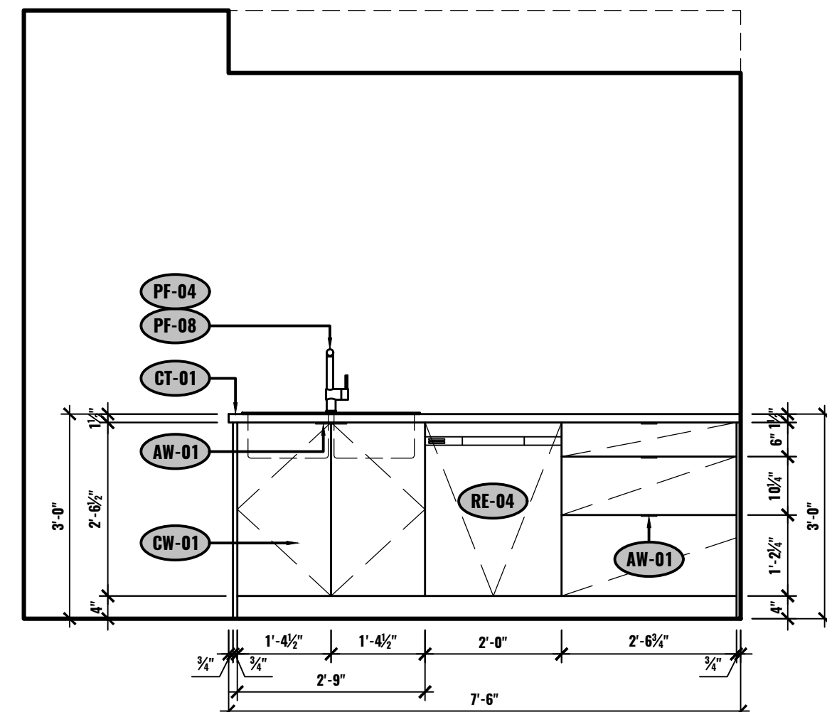
H ELEVATION - KITCHEN UNIT #603 1/2"=1'-0"
