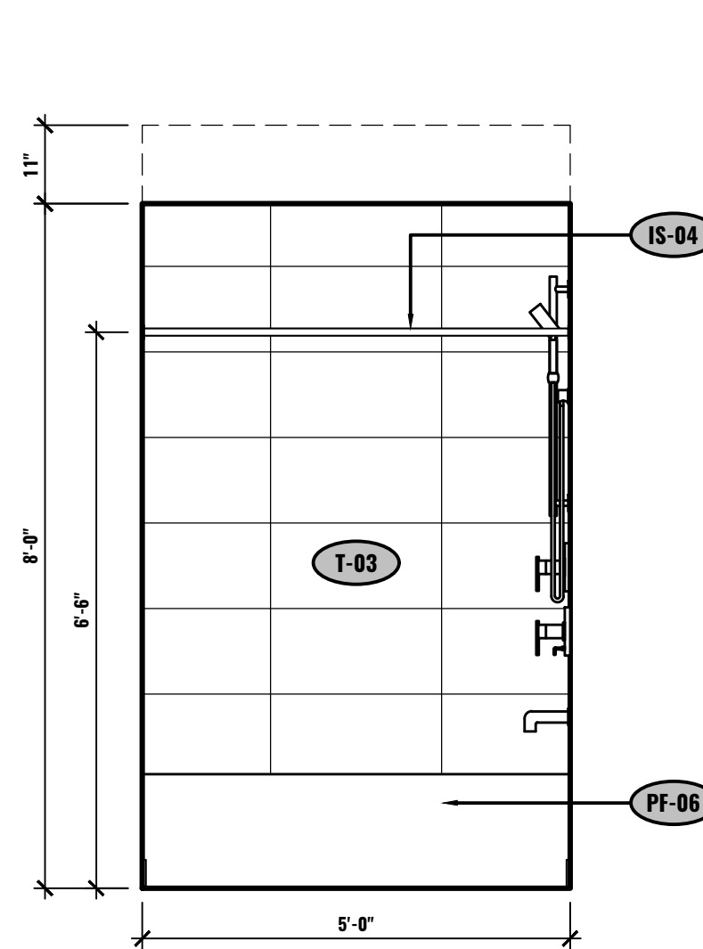
B ELEVATION - BATHROOM UNIT #2-505 1/2"=1'-0"
