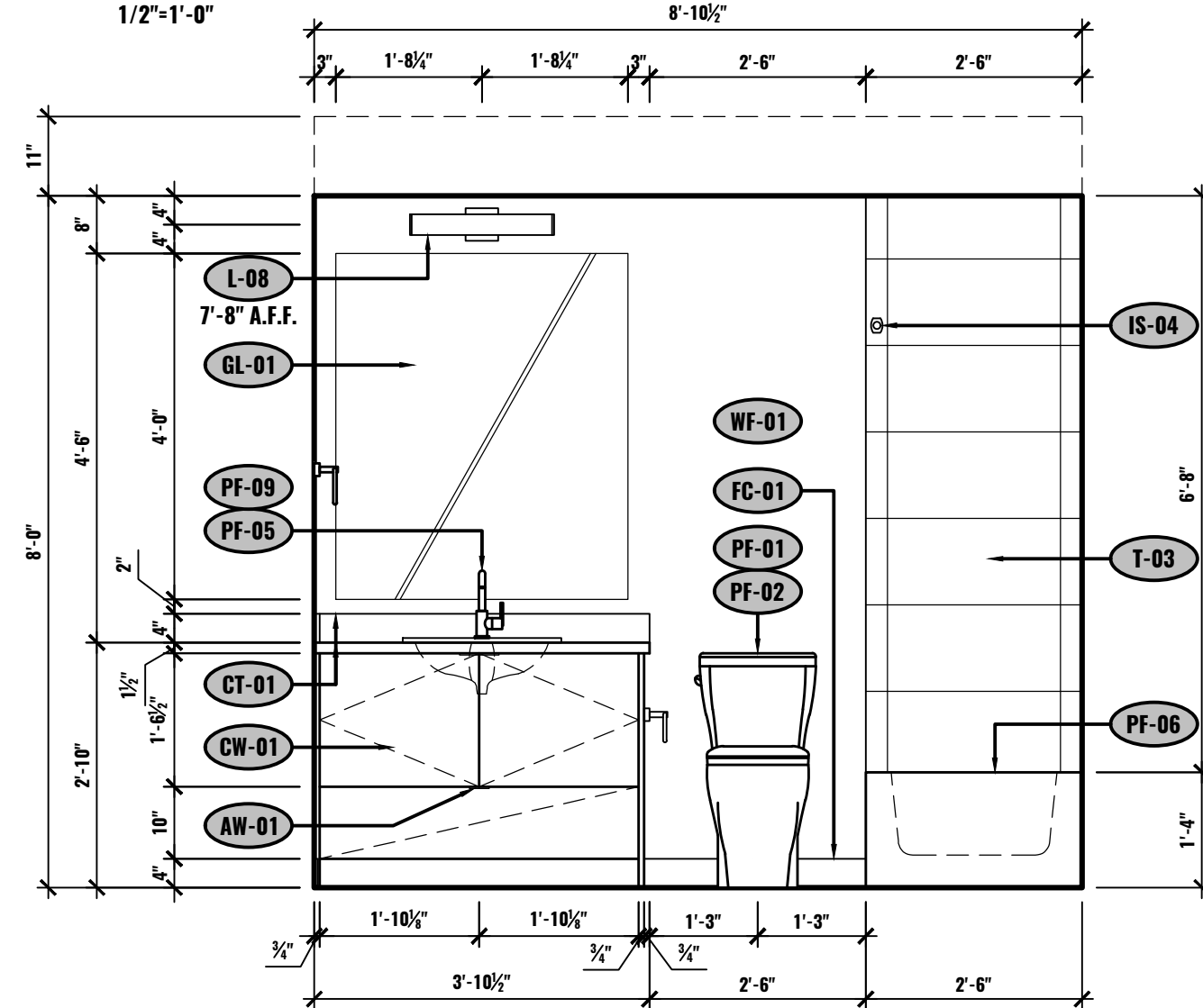
K ELEVATION - BATHROOM UNIT #2-504 1/2"=1'-0"
