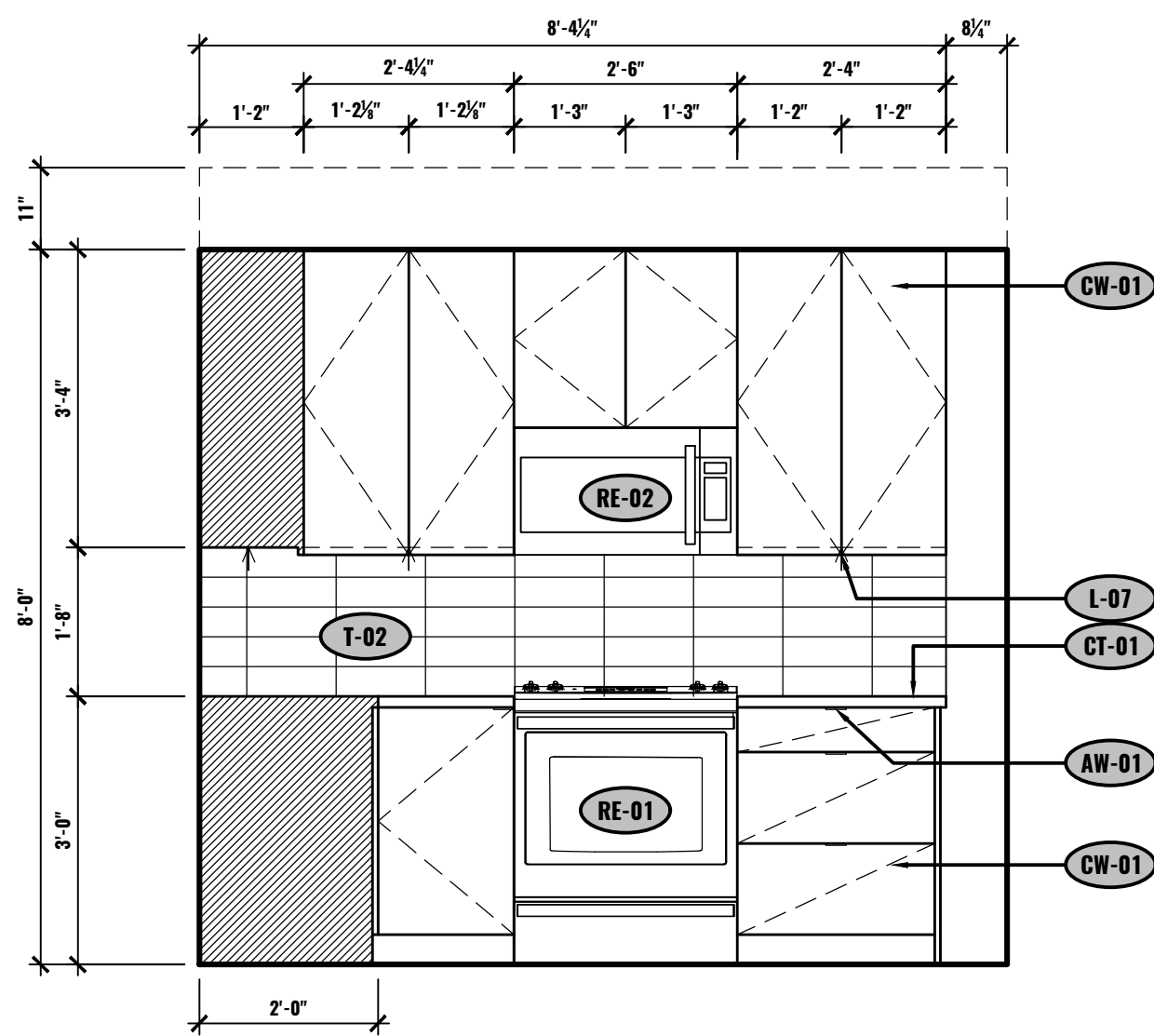
A ELEVATION - KITCHEN UNIT #604 1/2"=1'-0"
