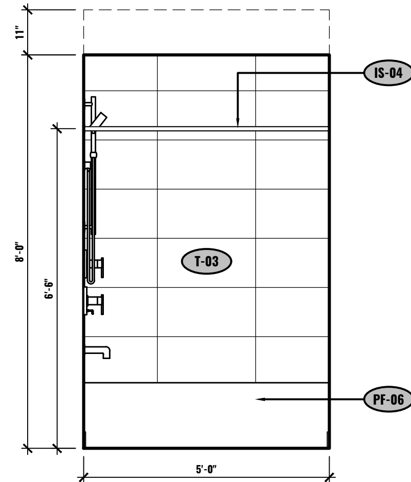
E ELEVATION - BATHROOM UNIT #604 1/2"=1'-0"
