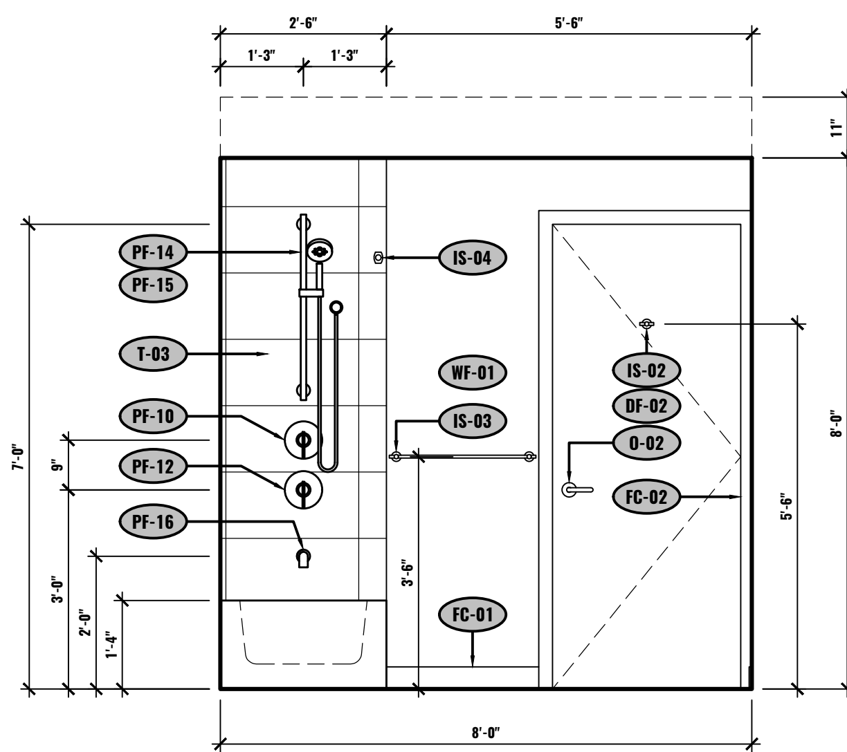
C ELEVATION - BATHROOM UNIT #2-505 1/2"=1'-0"
