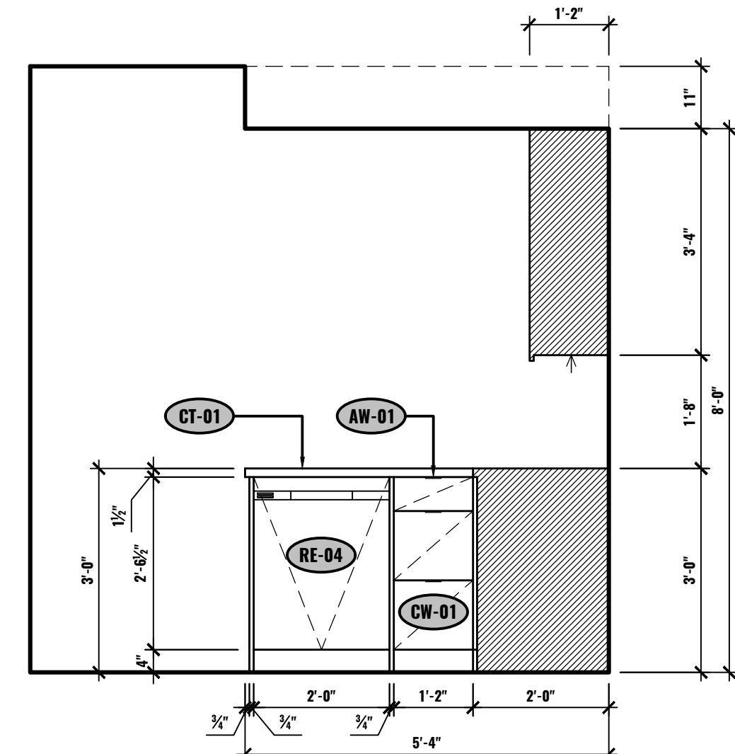
J ELEVATION - KITCHEN UNIT #2-506 1/2"=1'-0"
