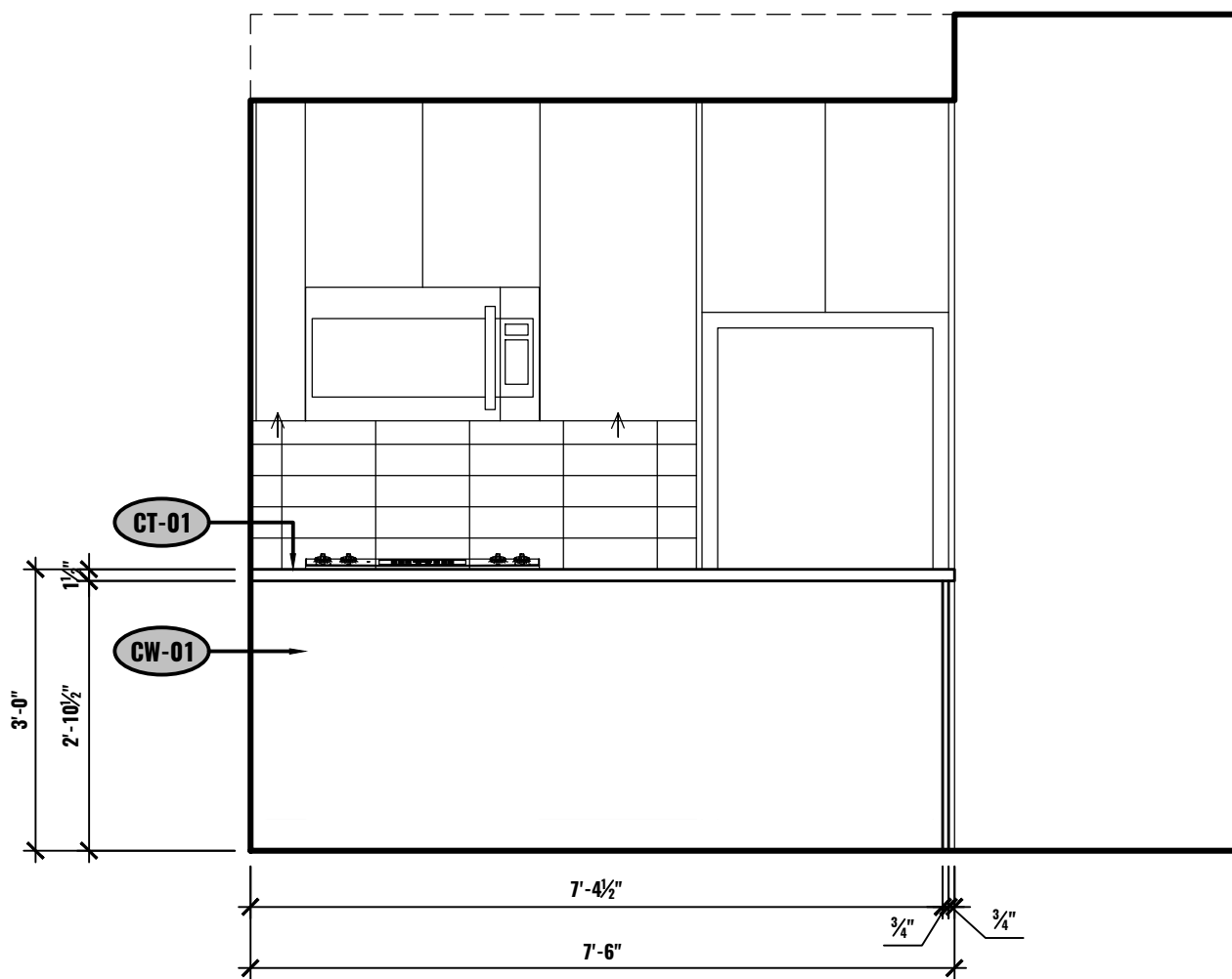
G ELEVATION - KITCHEN UNIT #603 1/2"=1'-0"
