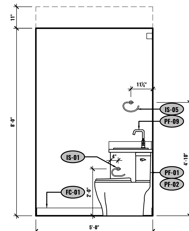
N ELEVATION - BATHROOM UNIT #2-506 1/2"=1'-0"
