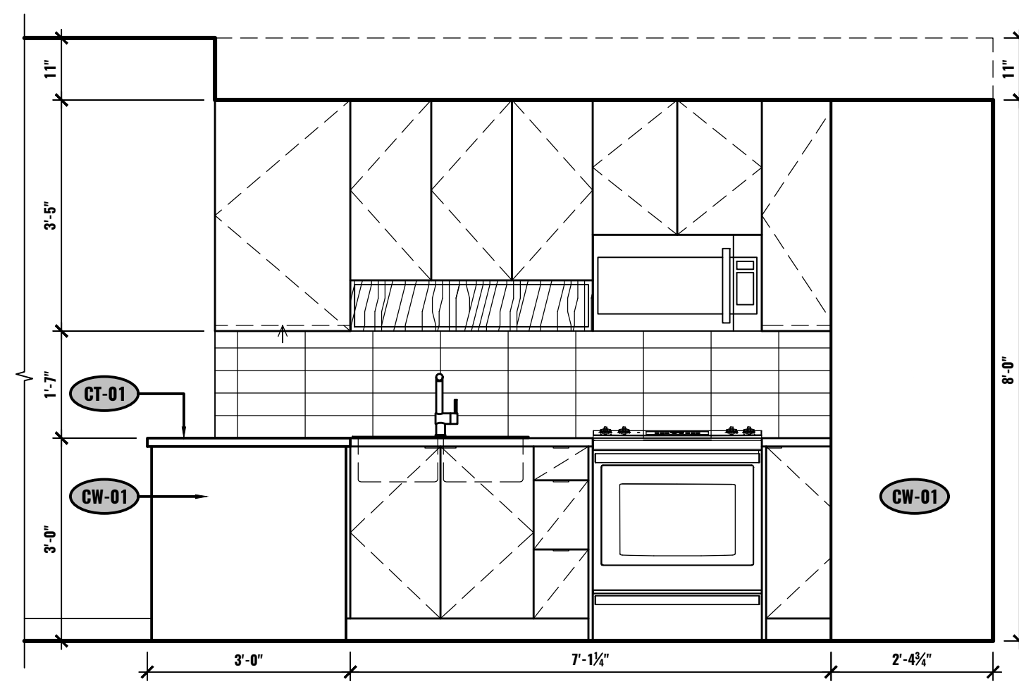
G ELEVATION - KITCHEN UNIT #2-505 1/2"=1'-0"
