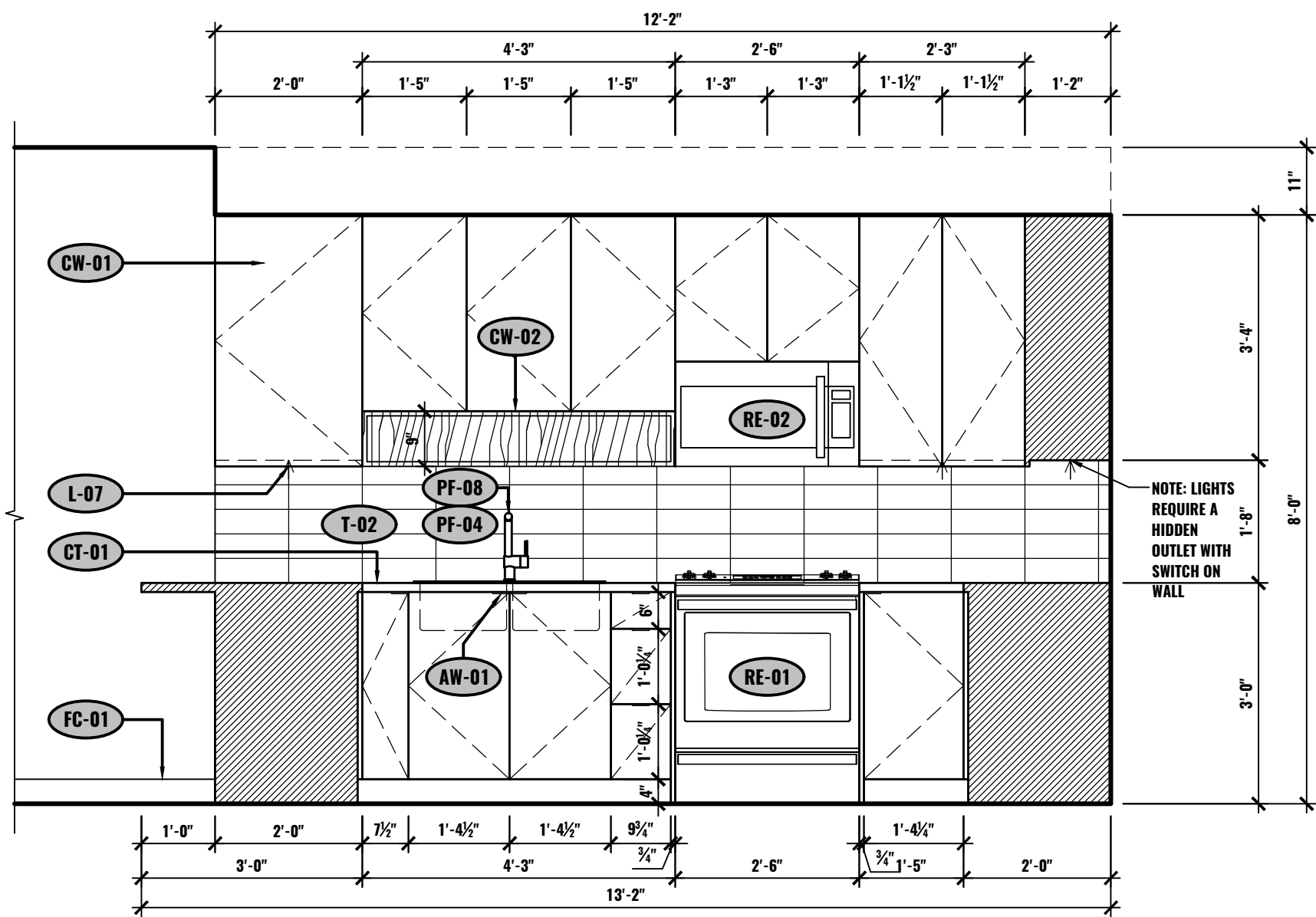
A ELEVATION - KITCHEN UNIT #2-503 1/2"=1'-0"
