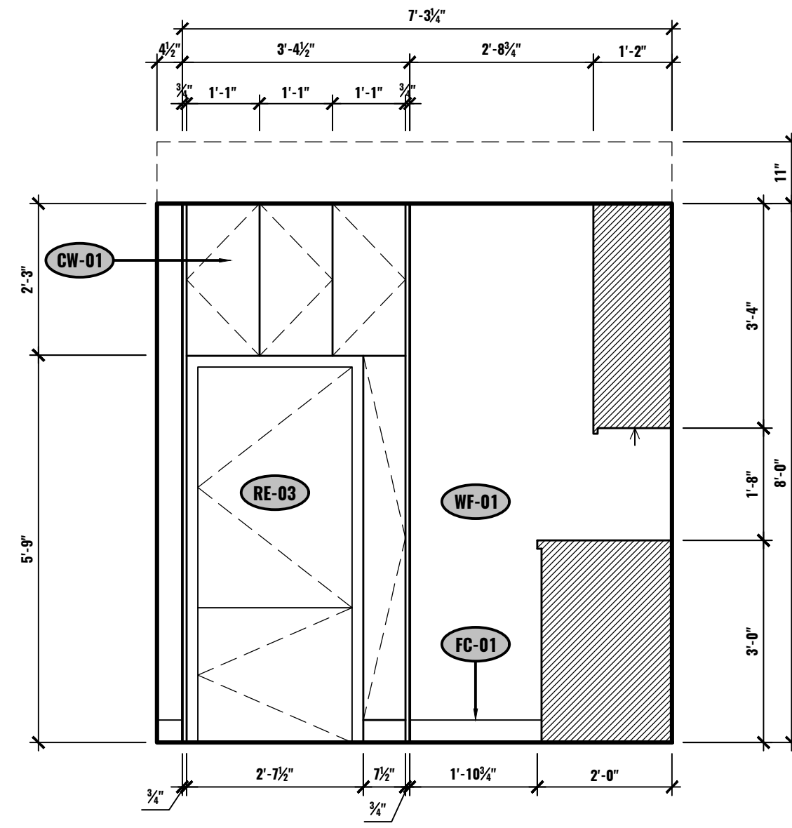
C ELEVATION - KITCHEN UNIT #604 1/2"=1'-0"
