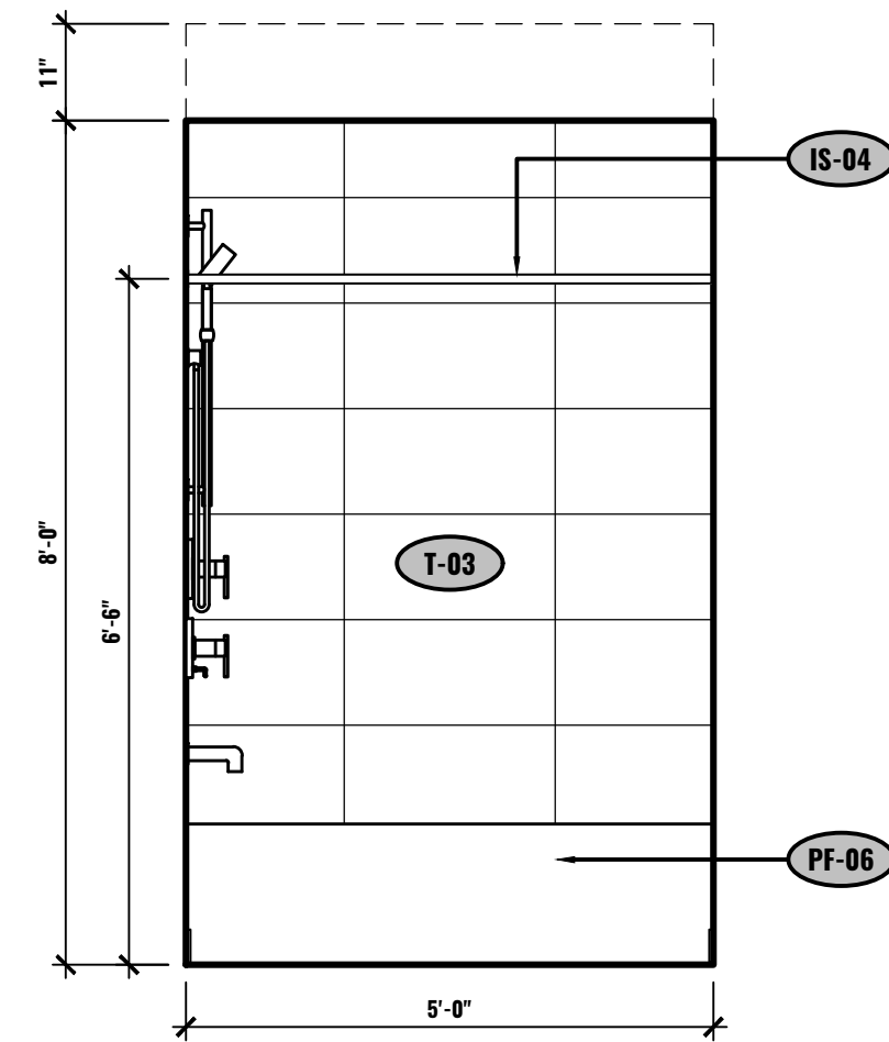
H ELEVATION - BATHROOM UNIT #2-507 1/2"=1'-0"
