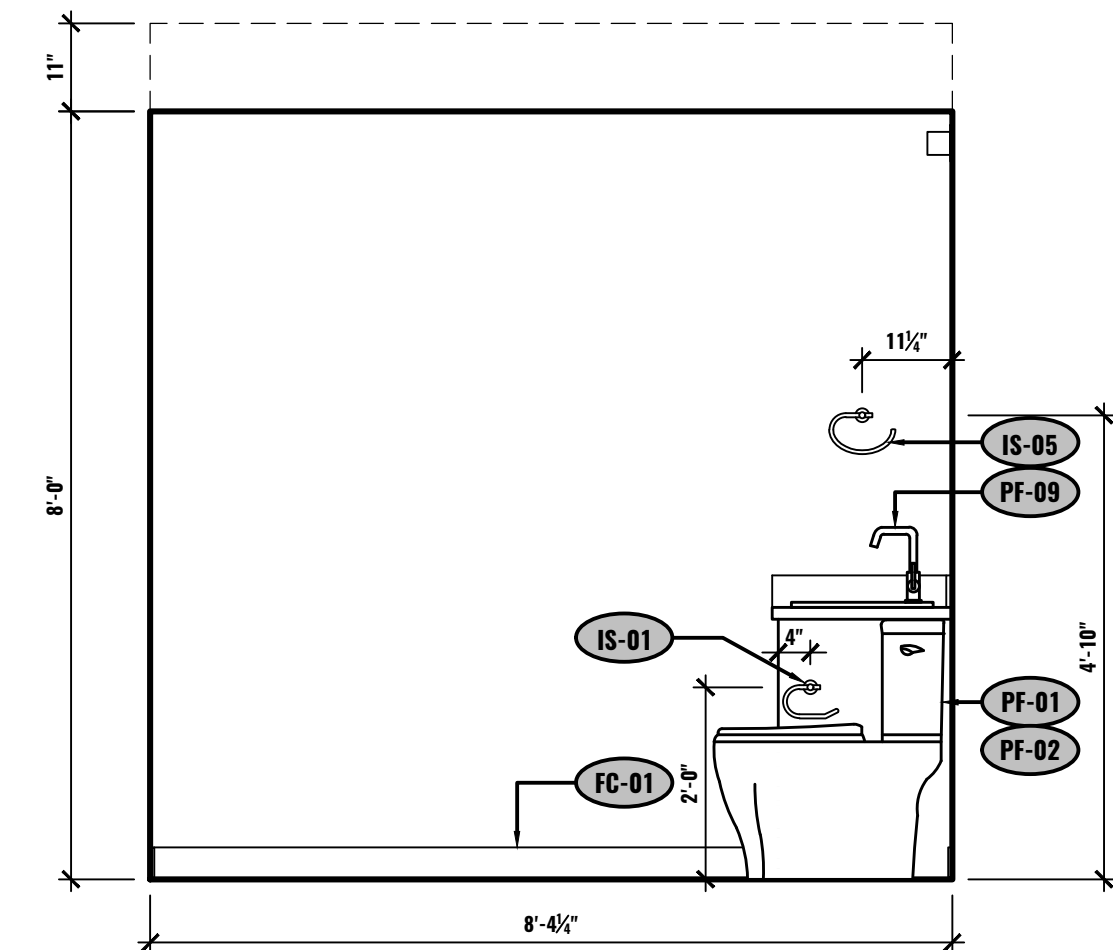
N ELEVATION - BATHROOM UNIT #2-504 1/2"=1'-0"
