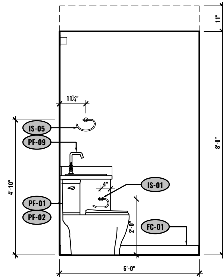
F ELEVATION - BATHROOM UNIT #2-501 1/2"=1'-0"
