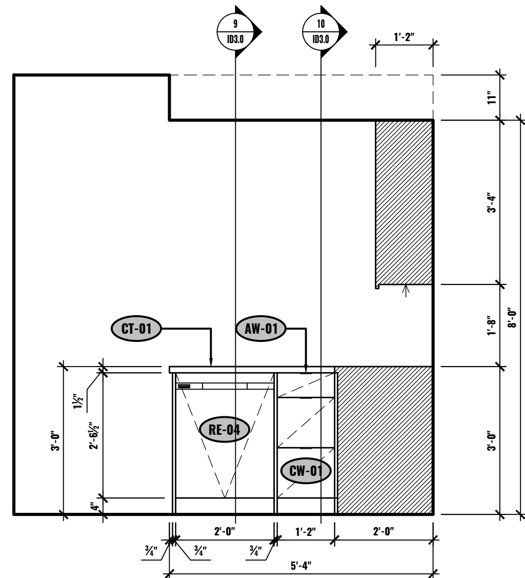
E ELEVATION - KITCHEN UNIT #2-503 1/2"=1'-0"
