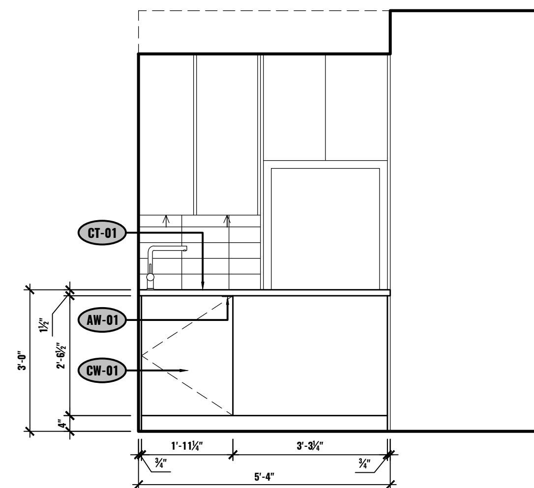
H ELEVATION - KITCHEN UNIT #2-506 1/2"=1'-0"
