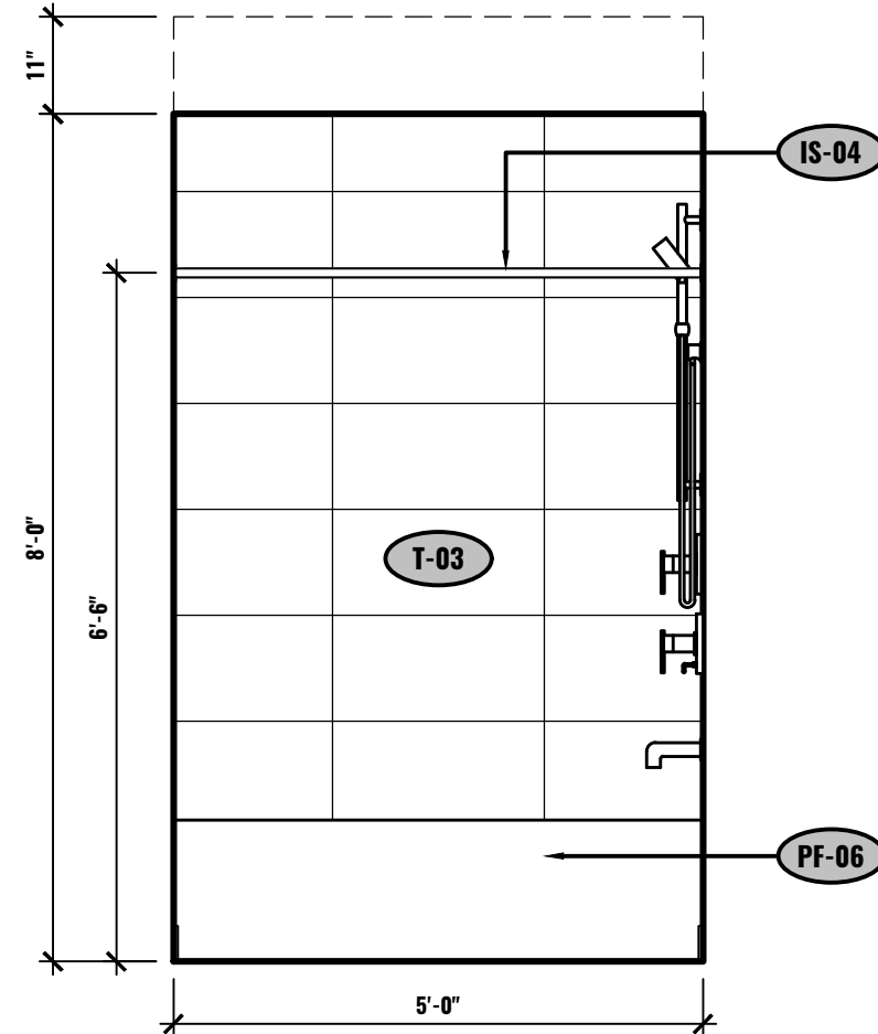
G ELEVATION - BATHROOM UNIT #2-503 1/2"=1'-0"
