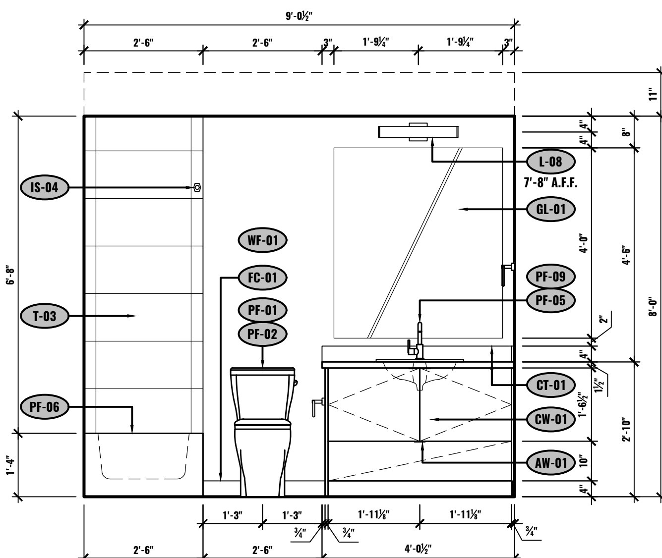
K ELEVATION - BATHROOM UNIT #603 1/2"=1'-0"
