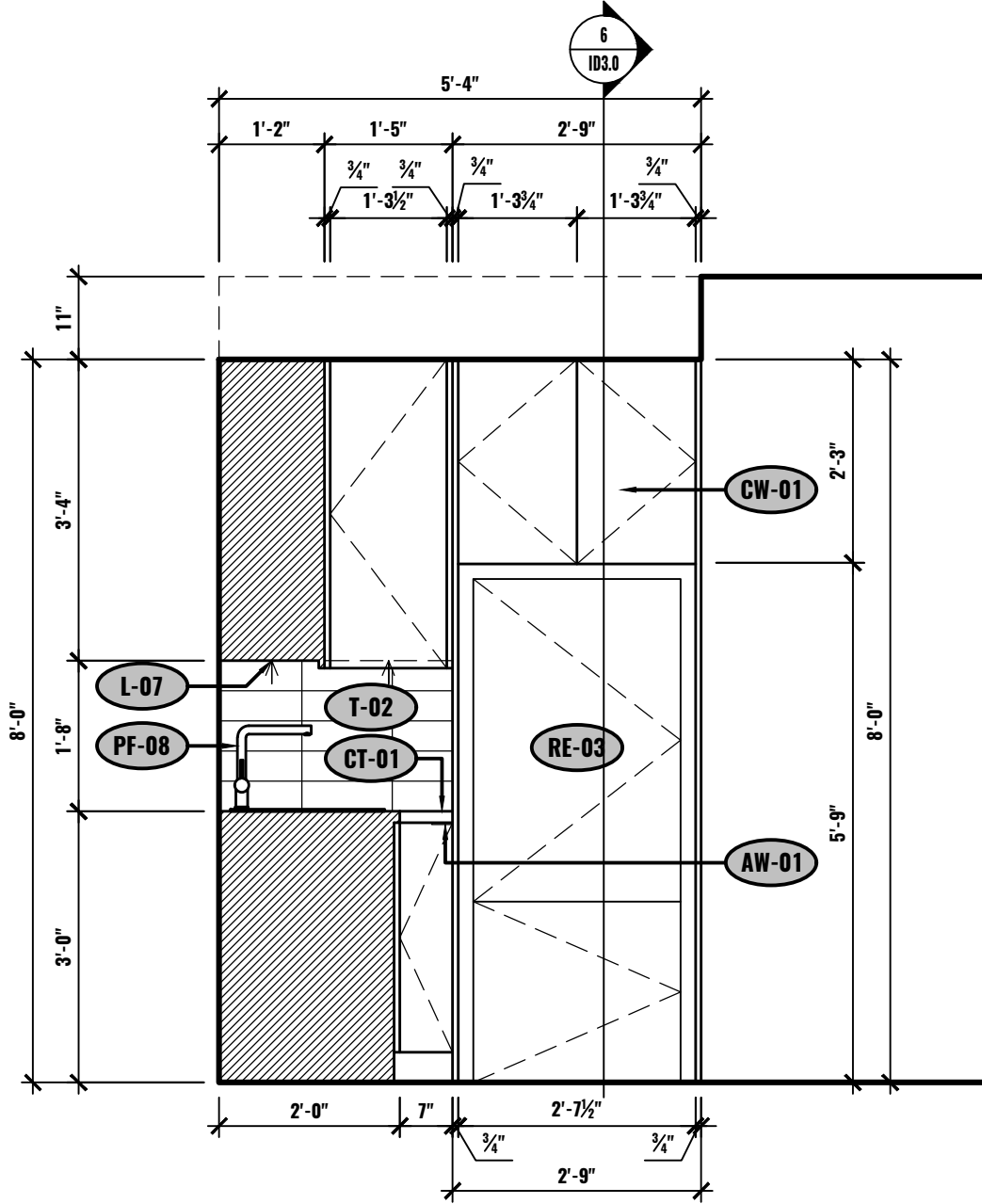
B ELEVATION - KITCHEN UNIT #2-501 1/2"=1'-0"
