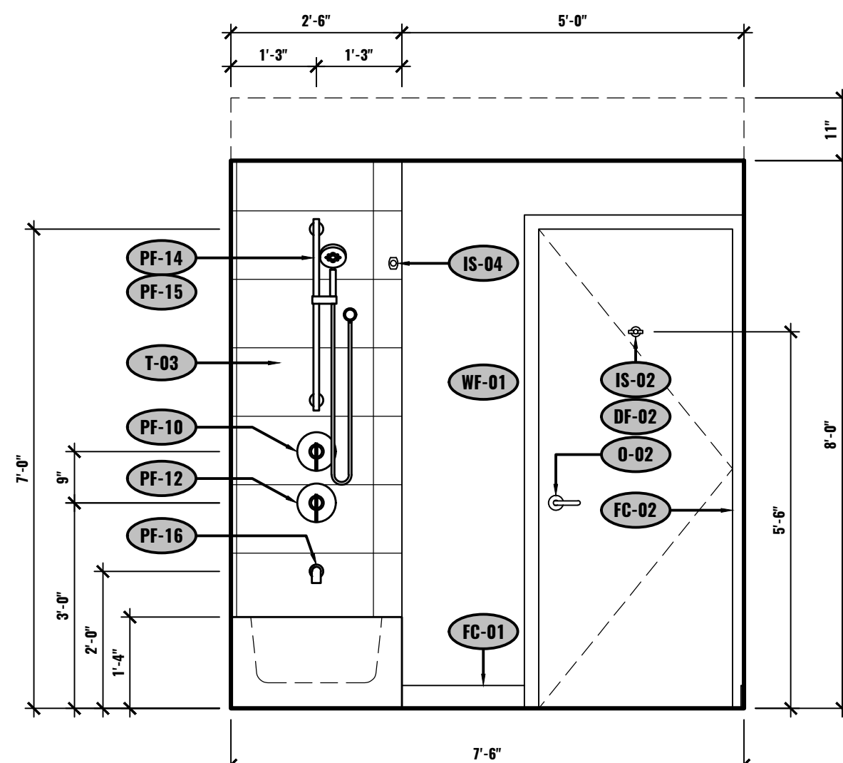
D ELEVATION - BATHROOM UNIT #602 1/2"=1'-0"
