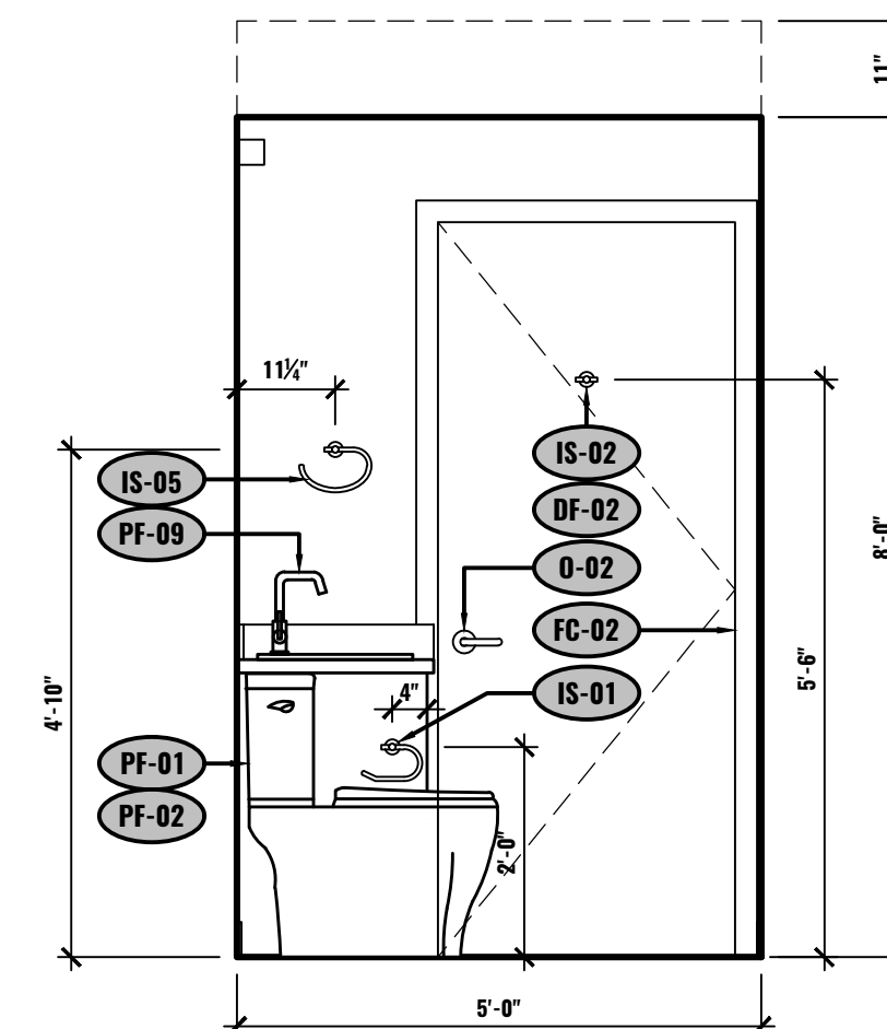
G ELEVATION - BATHROOM UNIT #604 1/2"=1'-0"
