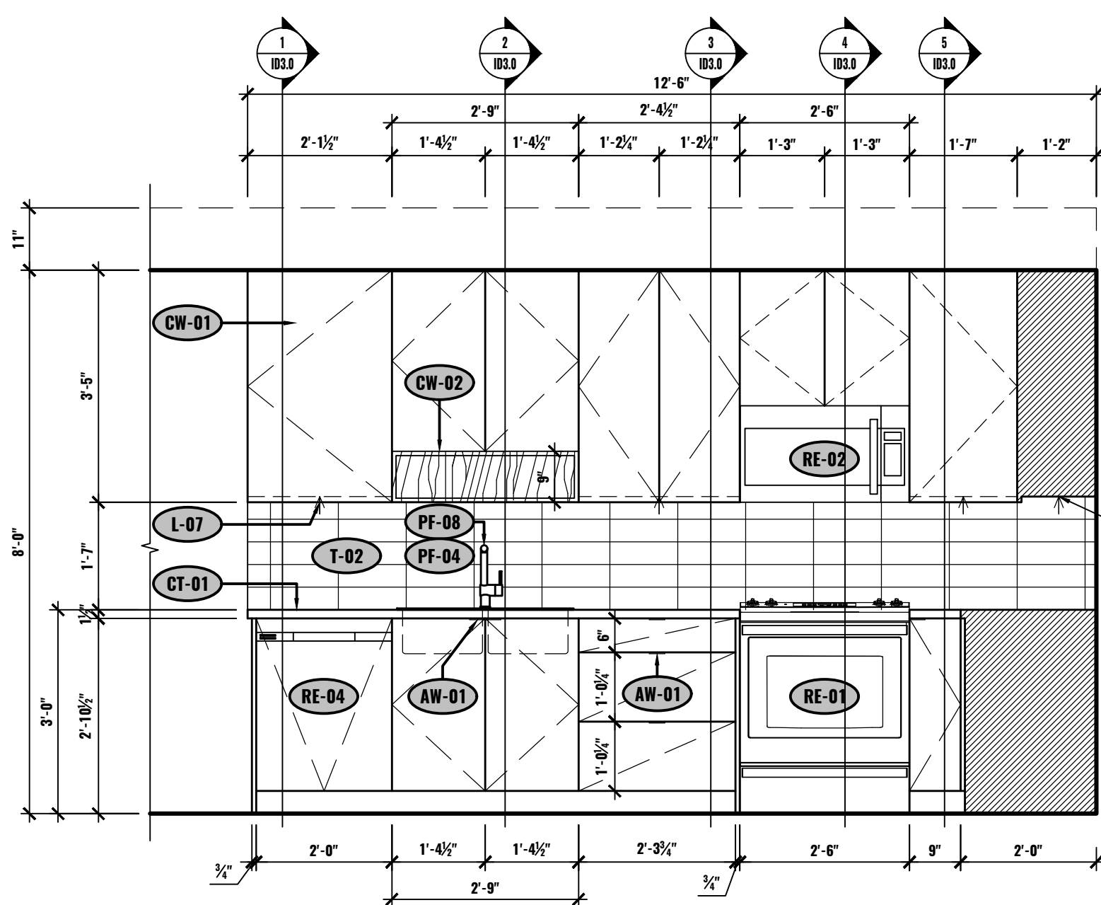
A ELEVATION - KITCHEN UNIT #2-501 1/2"=1'-0"
