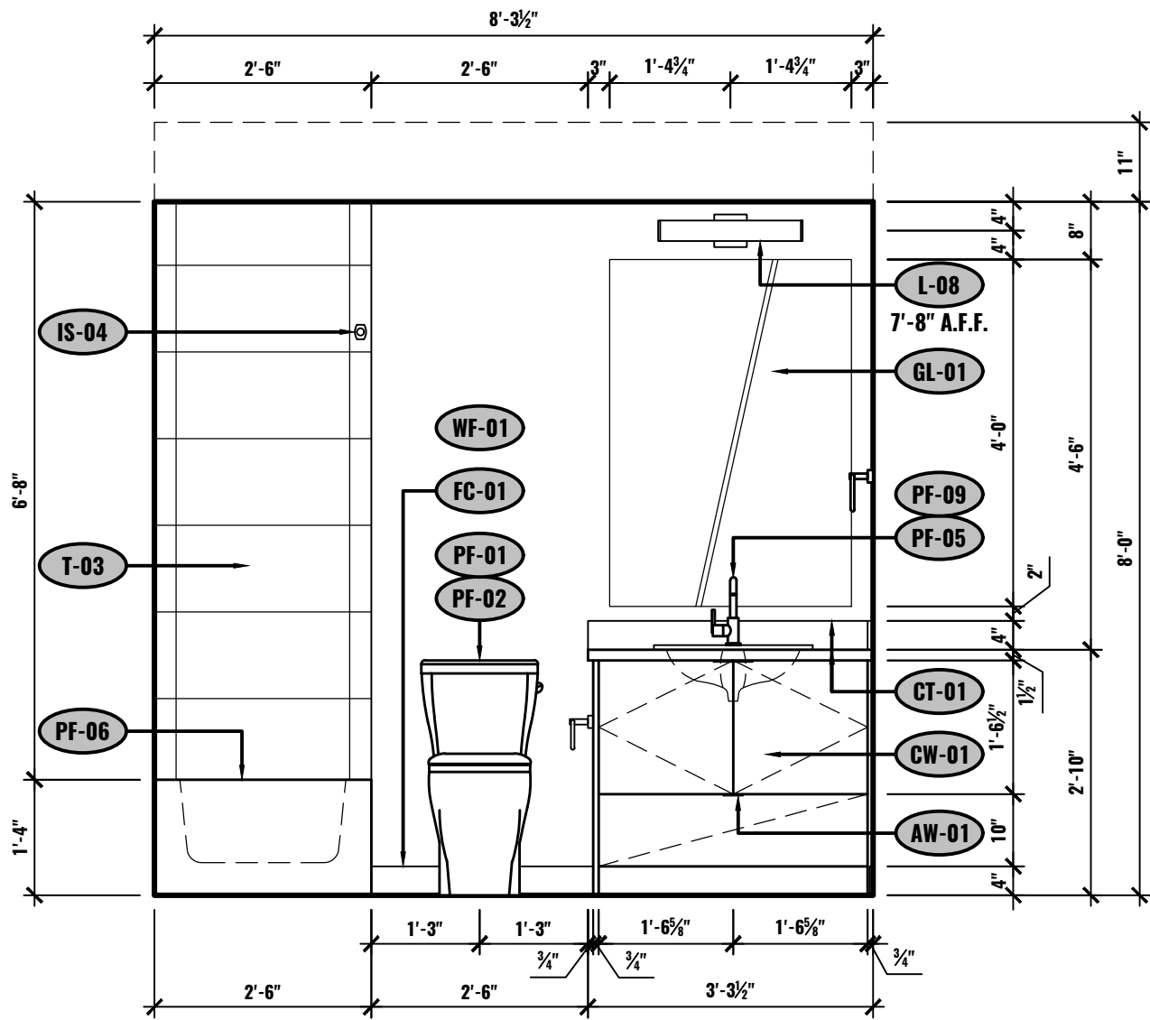
A ELEVATION - BATHROOM UNIT #2-506 1/2"=1'-0"
