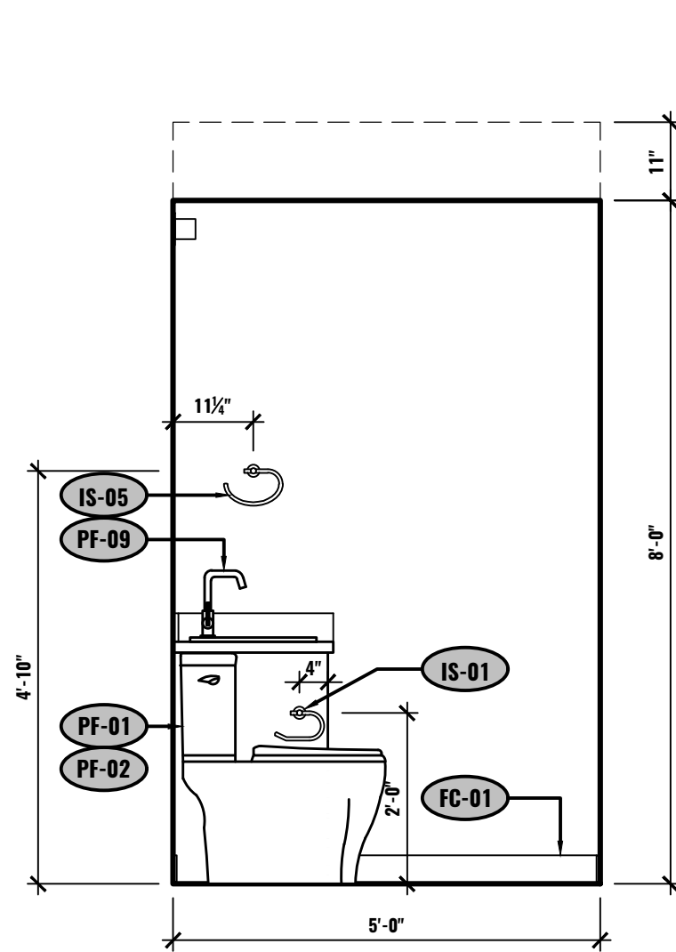
A ELEVATION - BATHROOM UNIT #602 1/2"=1'-0"
