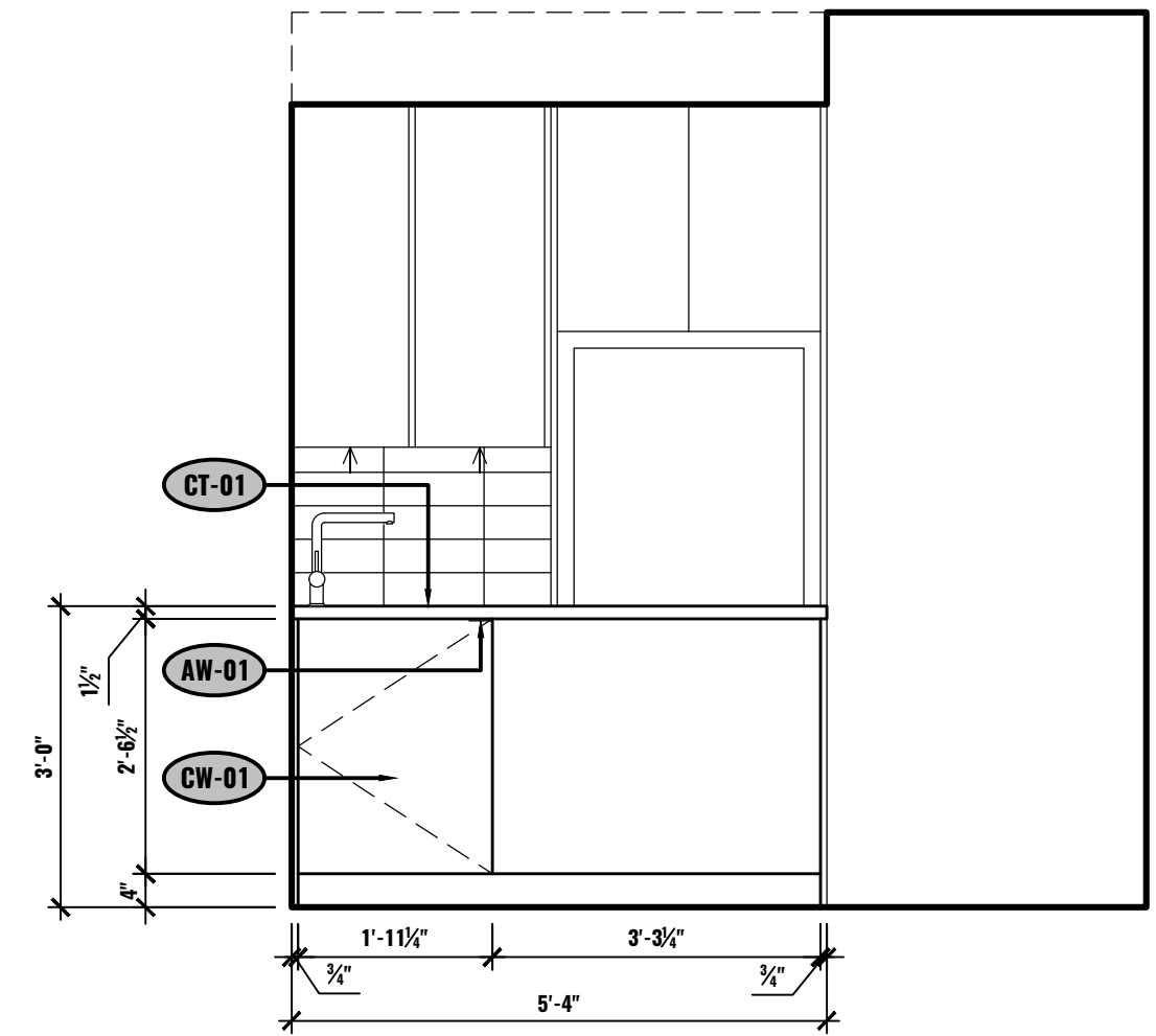
D ELEVATION - KITCHEN UNIT #2-504 1/2"=1'-0"
