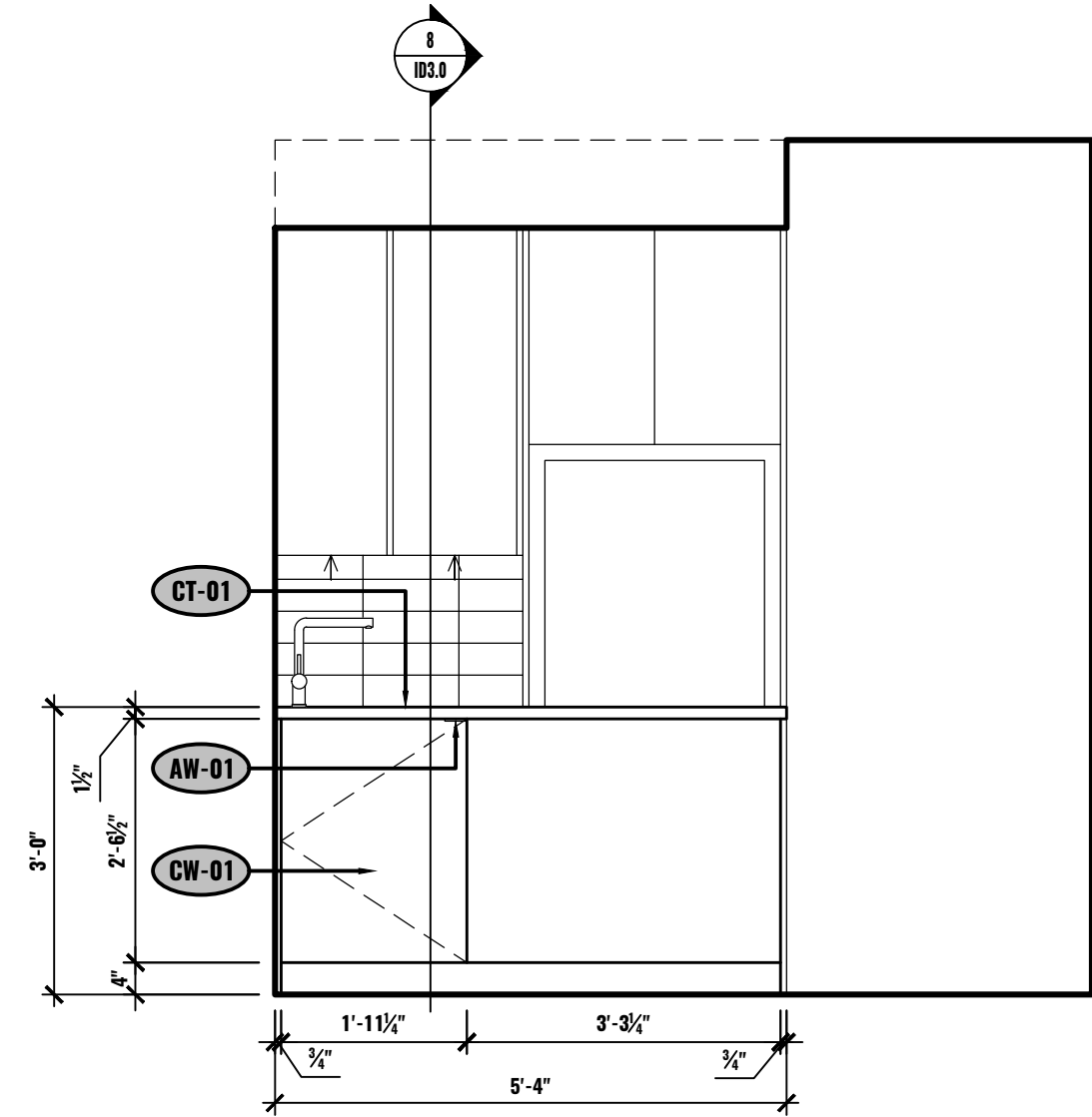
D ELEVATION - KITCHEN UNIT #2-503 1/2"=1'-0"
