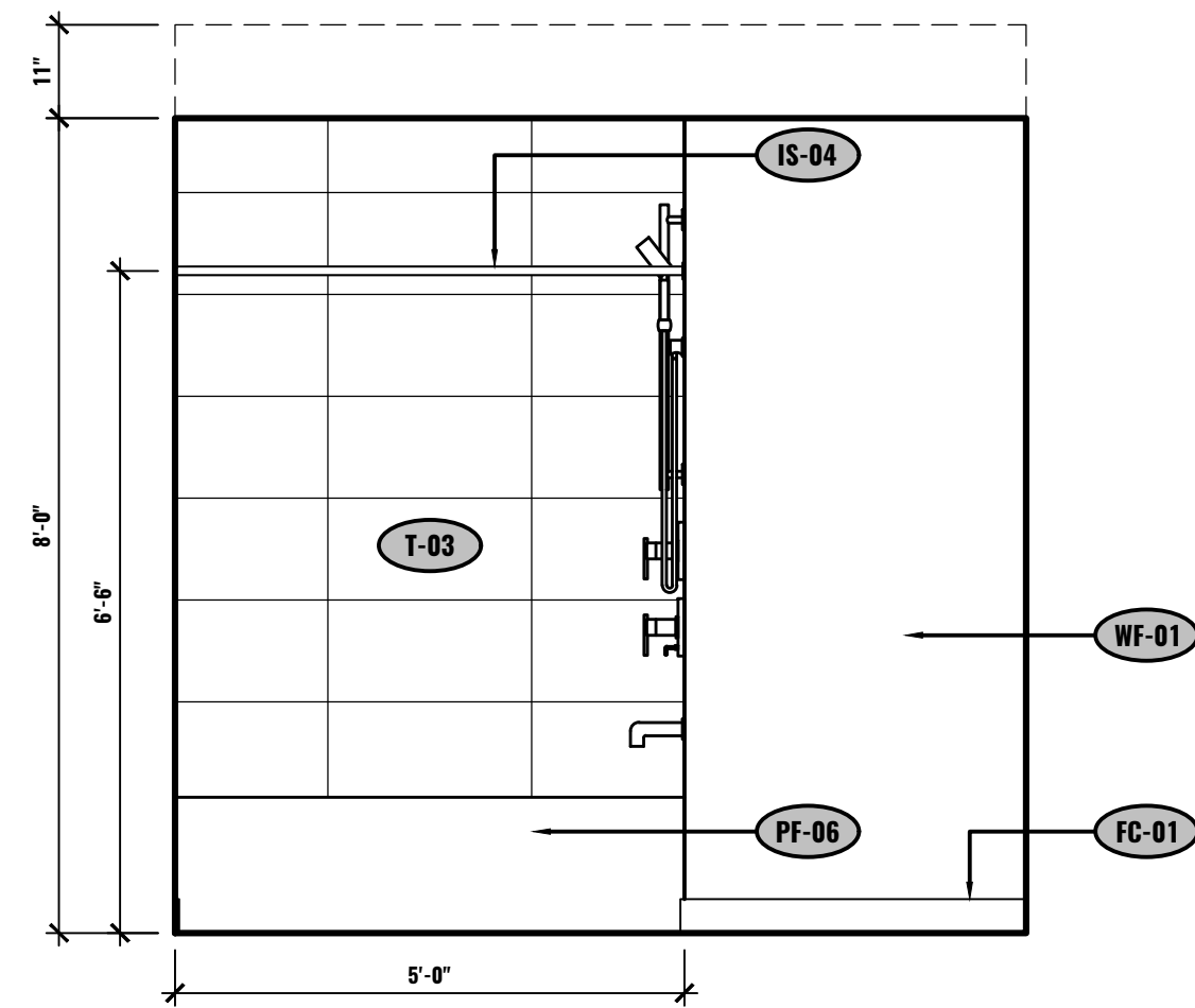
L ELEVATION - BATHROOM UNIT #2-504 1/2"=1'-0"
