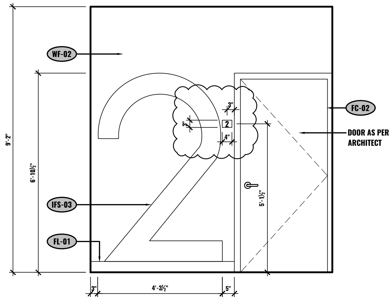
D ELEVATION - STAIRS #4 & STAIRS #5 ALL LEVELS 1/2"=1'-0"
