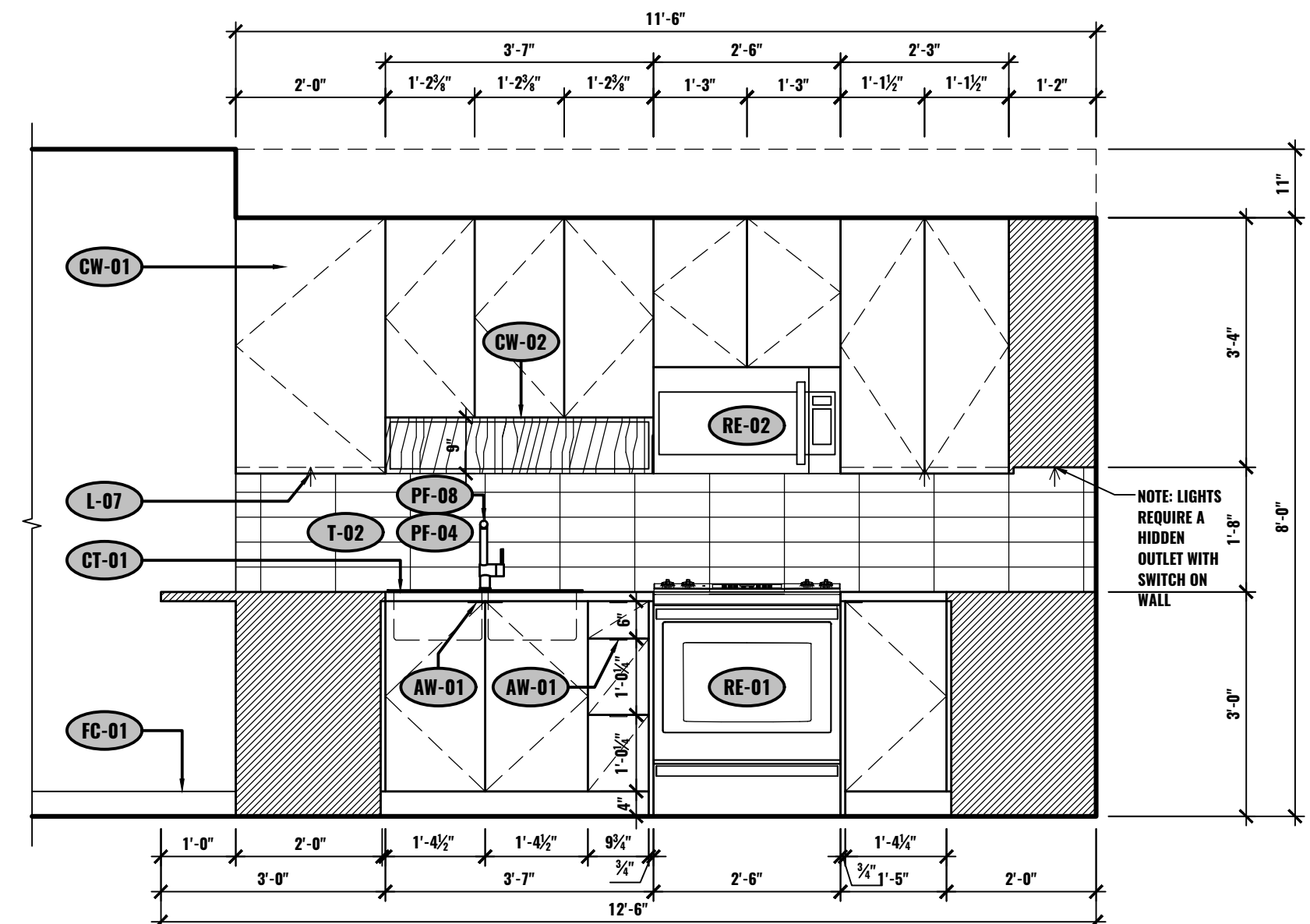
E ELEVATION - KITCHEN UNIT #2-506 1/2"=1'-0"
