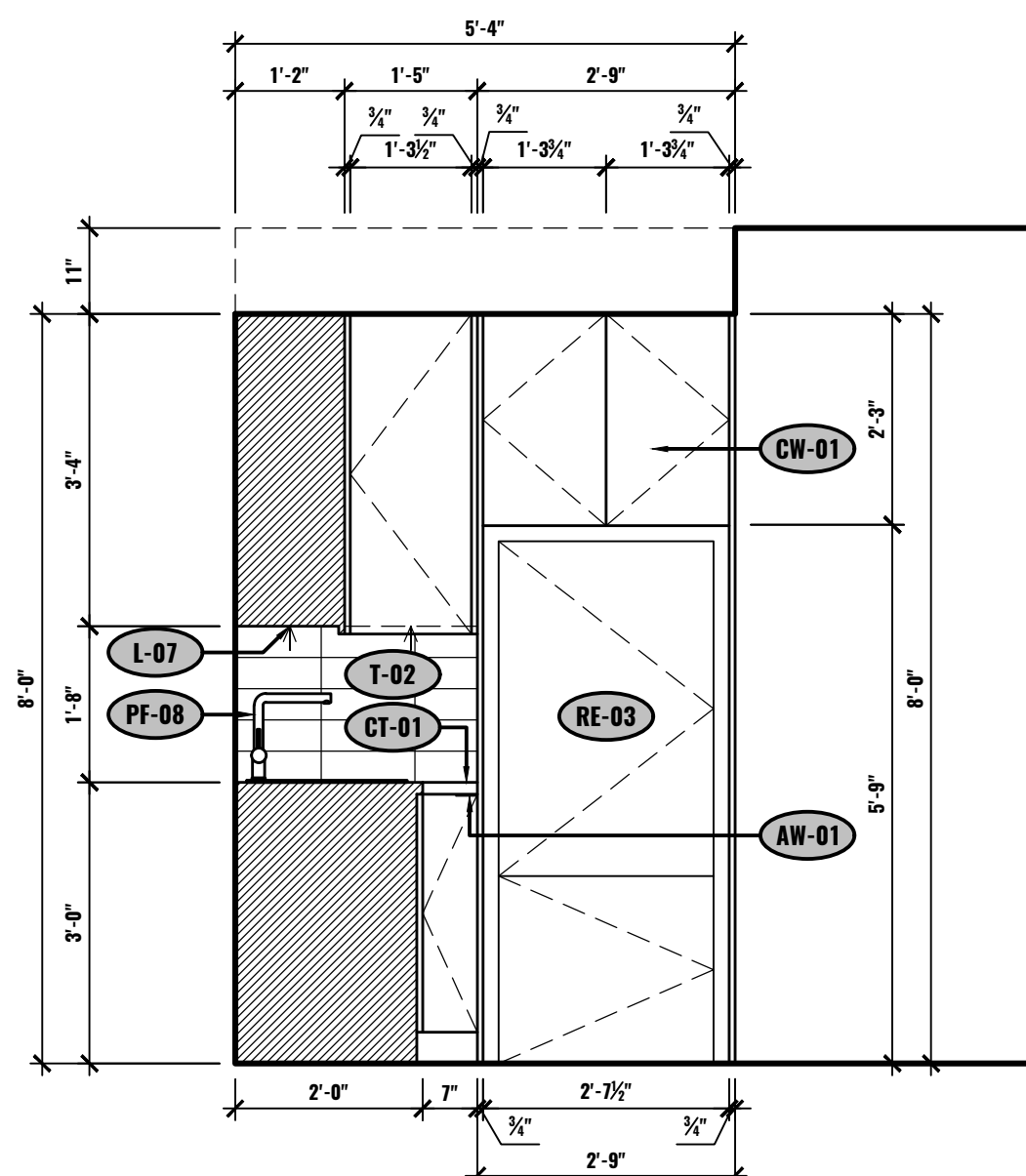
G ELEVATION - KITCHEN UNIT #2-506 1/2"=1'-0"
