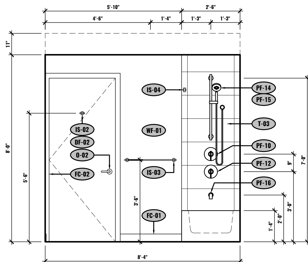
E ELEVATION - BATHROOM UNIT #2-501 1/2"=1'-0"
