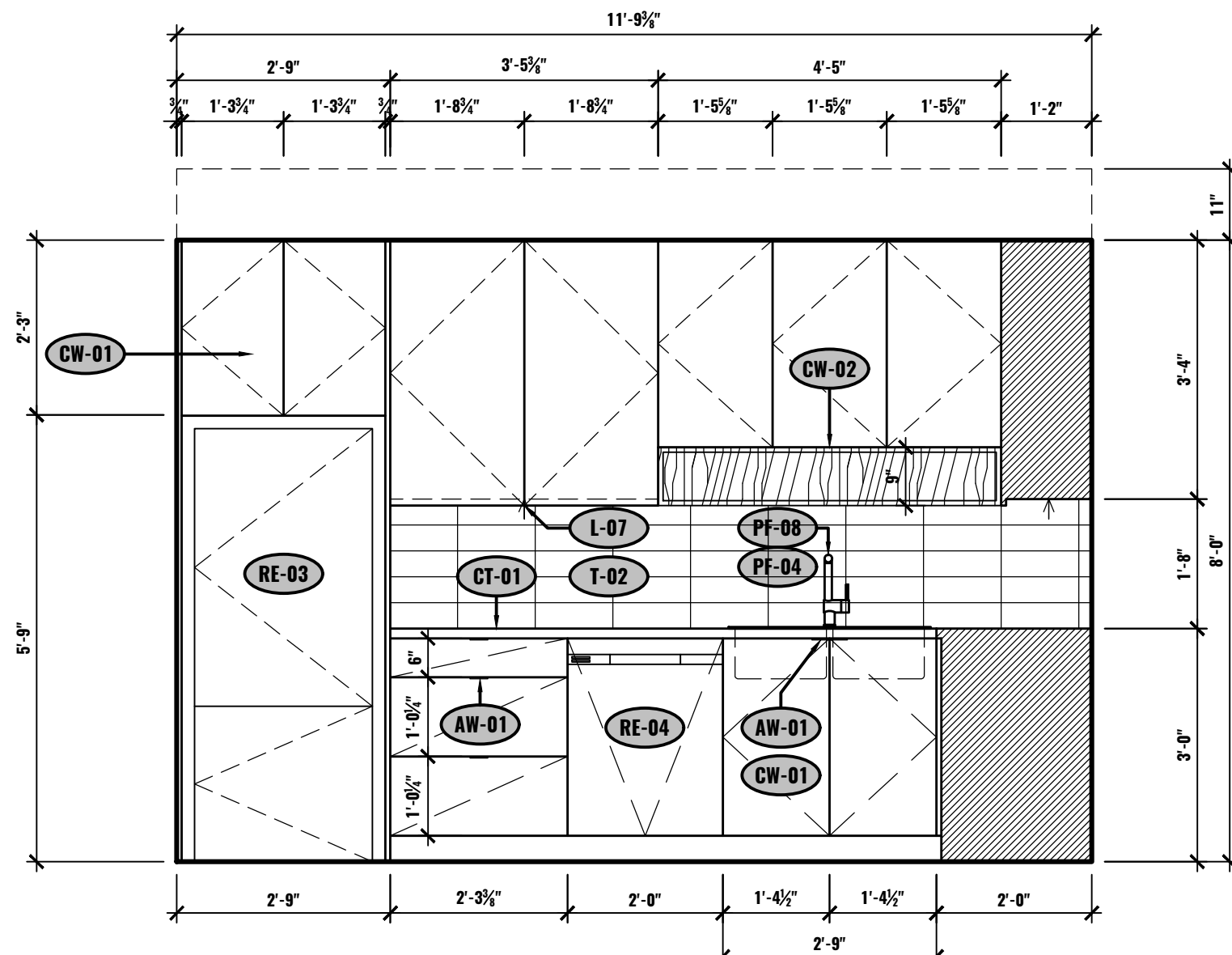
E ELEVATION - KITCHEN UNIT #2-507 1/2"=1'-0"
