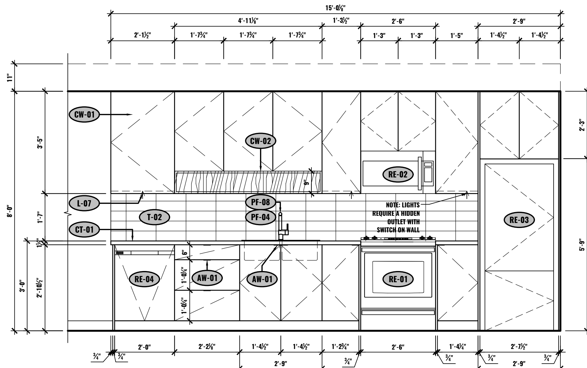
J ELEVATION - KITCHEN UNIT #602 1/2"=1'-0"
