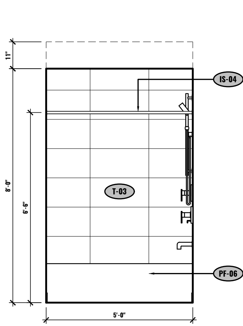
C ELEVATION - BATHROOM UNIT #602 1/2"=1'-0"
