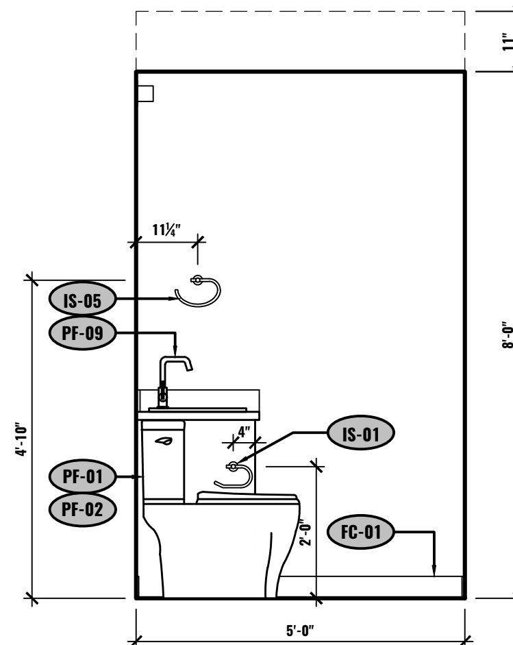
D ELEVATION - BATHROOM UNIT #2-506 1/2"=1'-0"
