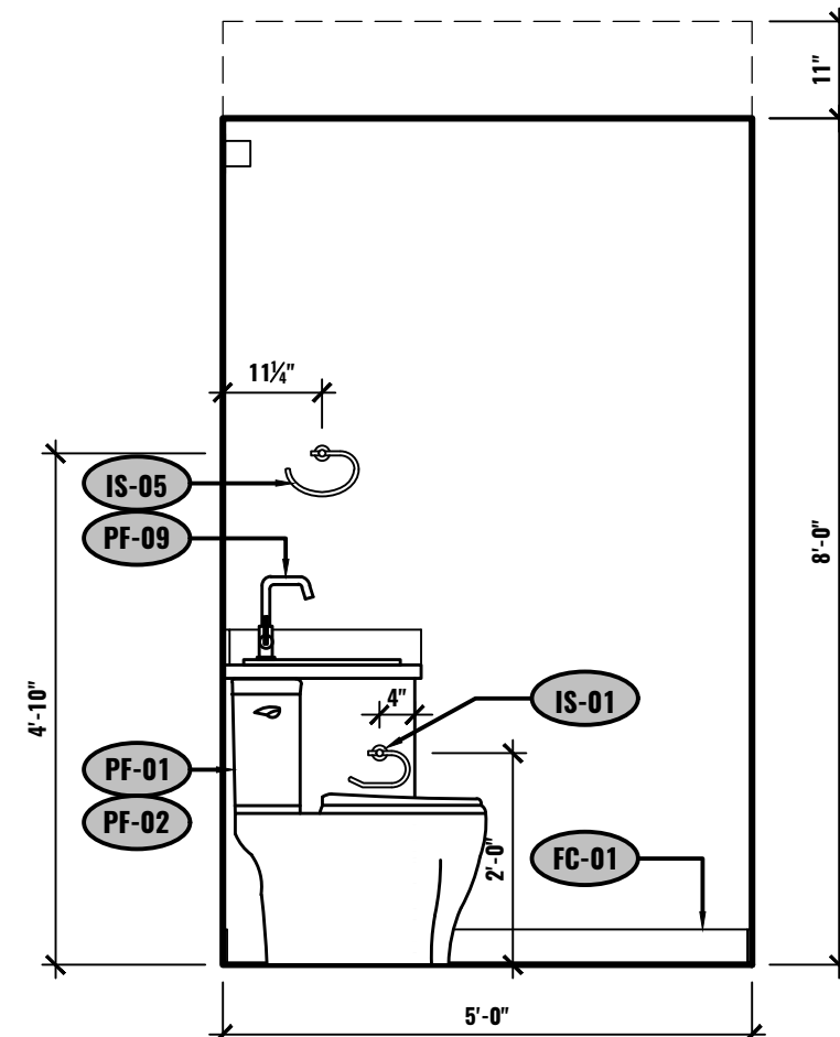
N ELEVATION - BATHROOM UNIT #603 1/2"=1'-0"
