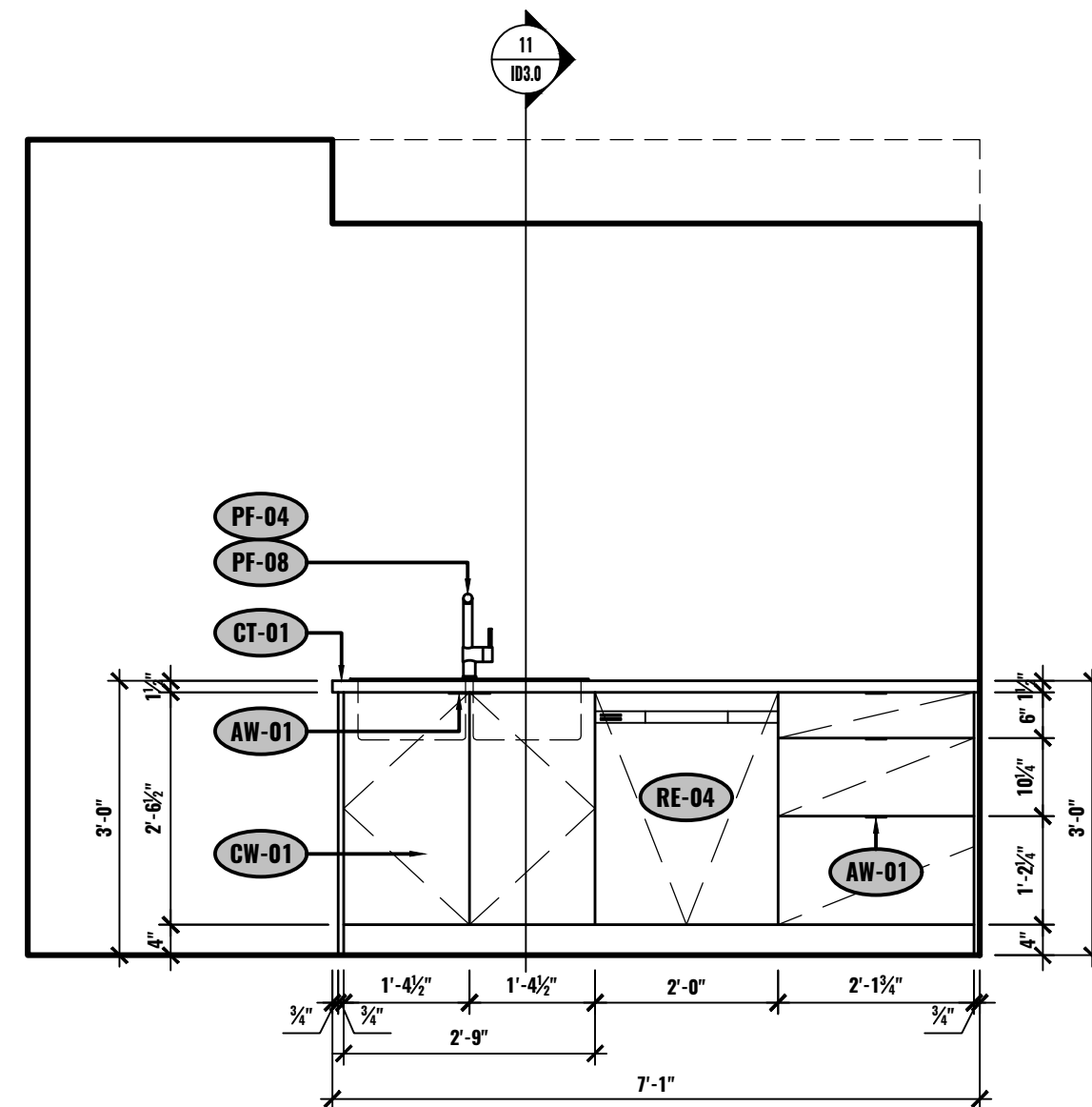
C ELEVATION - KITCHEN UNIT #601 1/2"=1'-0"
