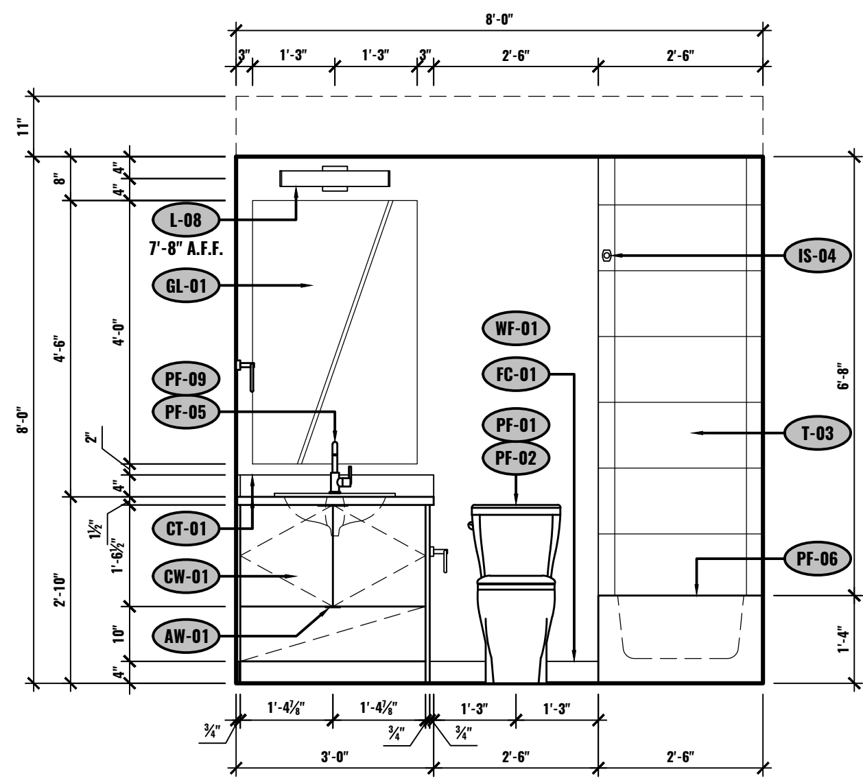
A ELEVATION - BATHROOM UNIT #2-505 1/2"=1'-0"
