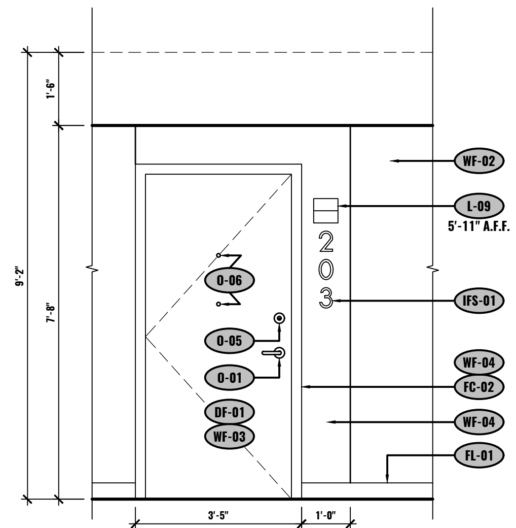
F ELEVATION - SUITE ENTRY ALL LEVELS 1/2"=1'-0"
