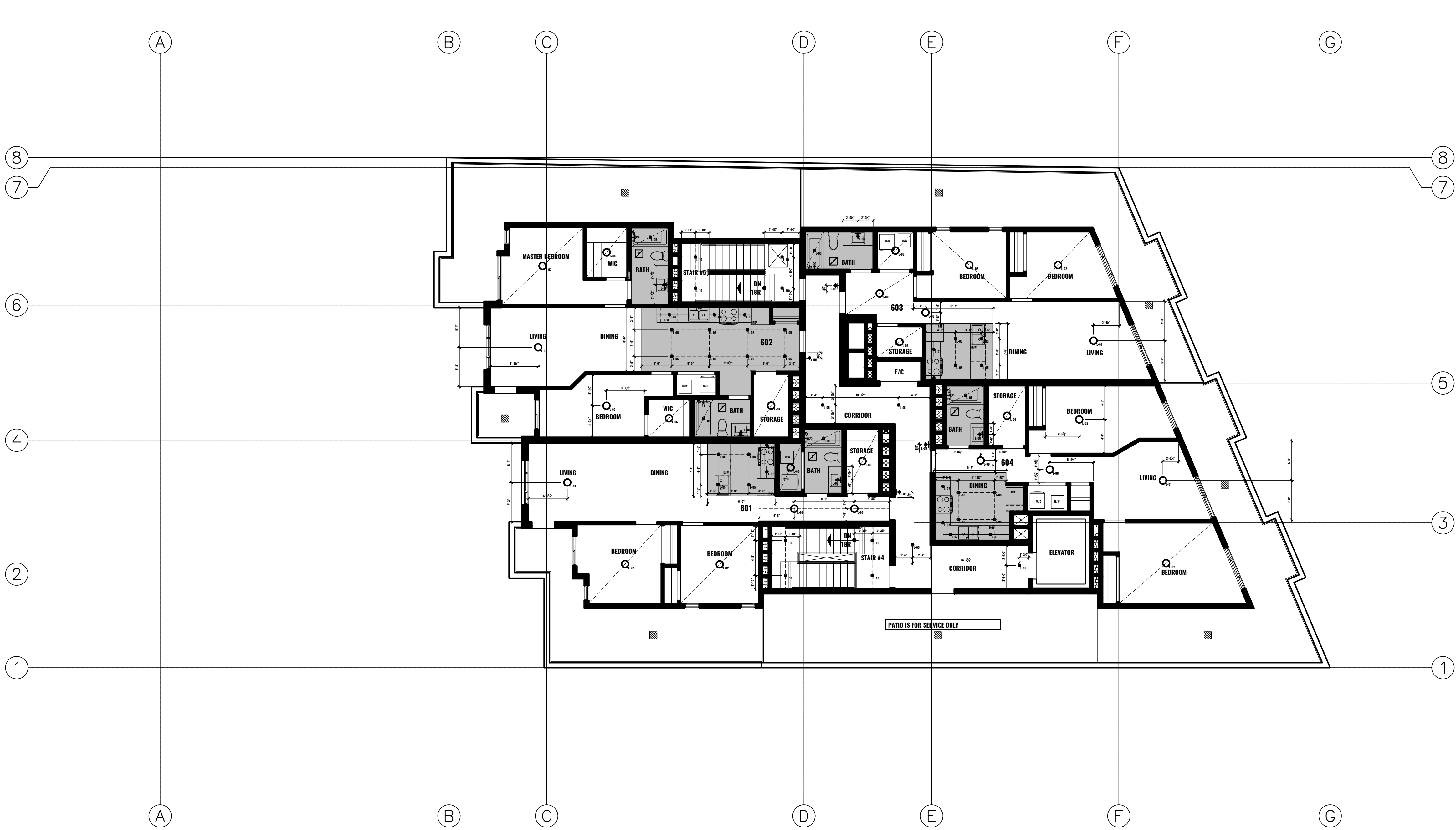
3 REFLECTED CEILING PLAN LEVEL 6 1/8"=1'-0"
