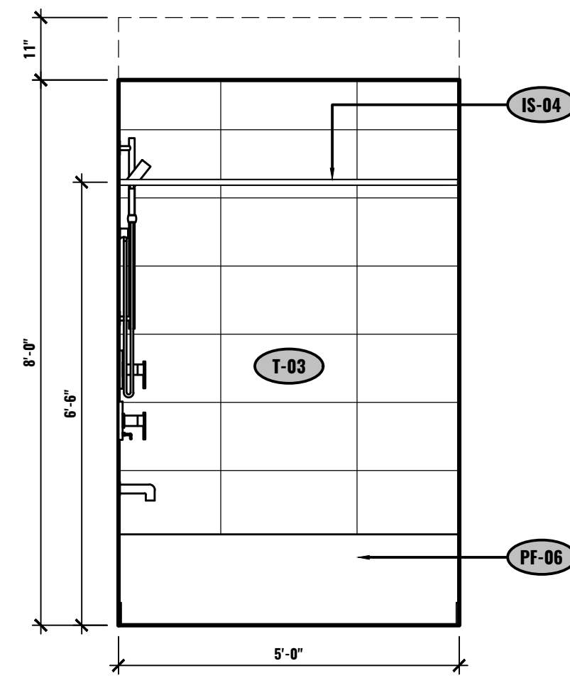
L ELEVATION - BATHROOM UNIT #602 1/2"=1'-0"
