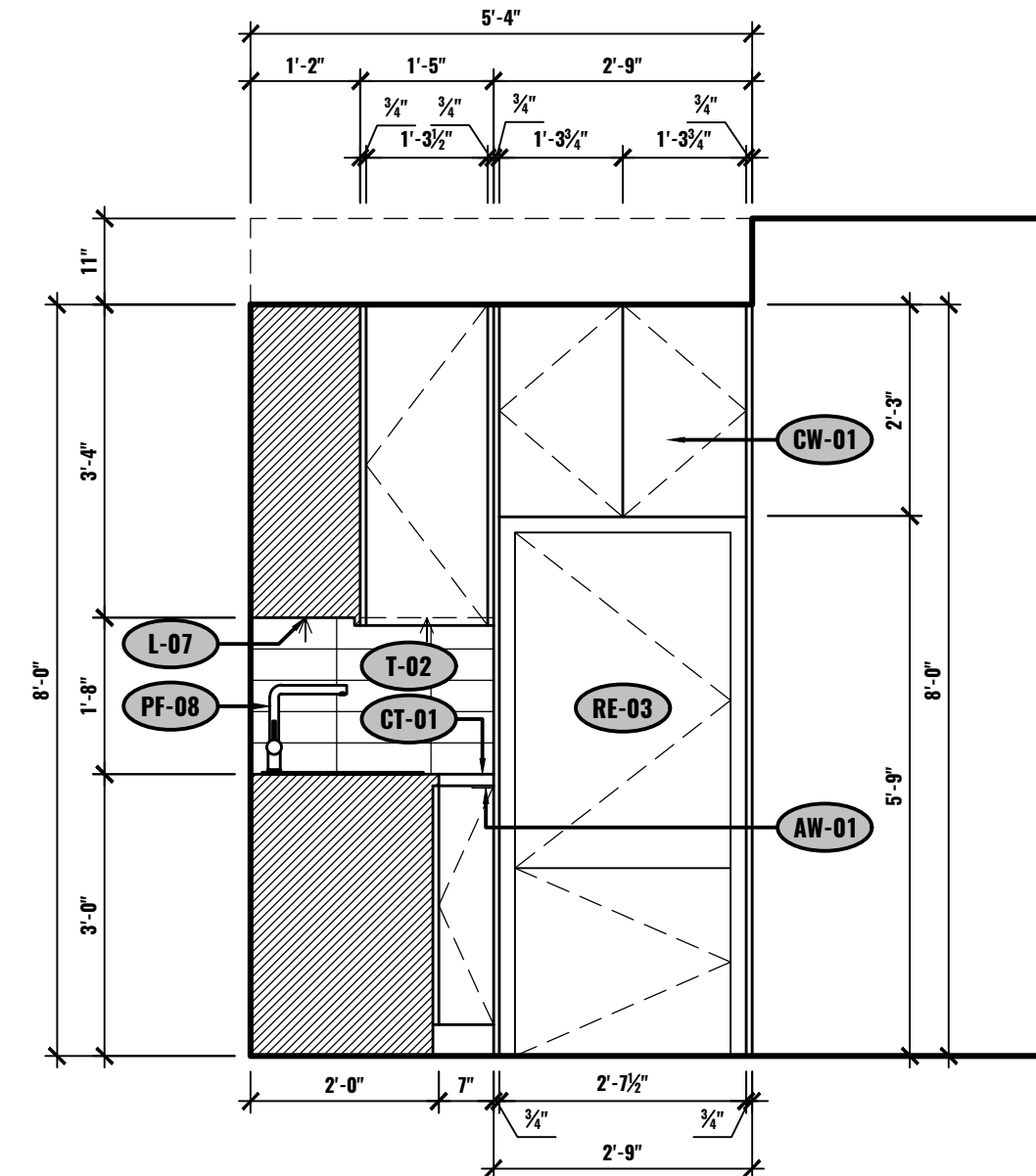
C ELEVATION - KITCHEN UNIT #2-503 1/2"=1'-0"
