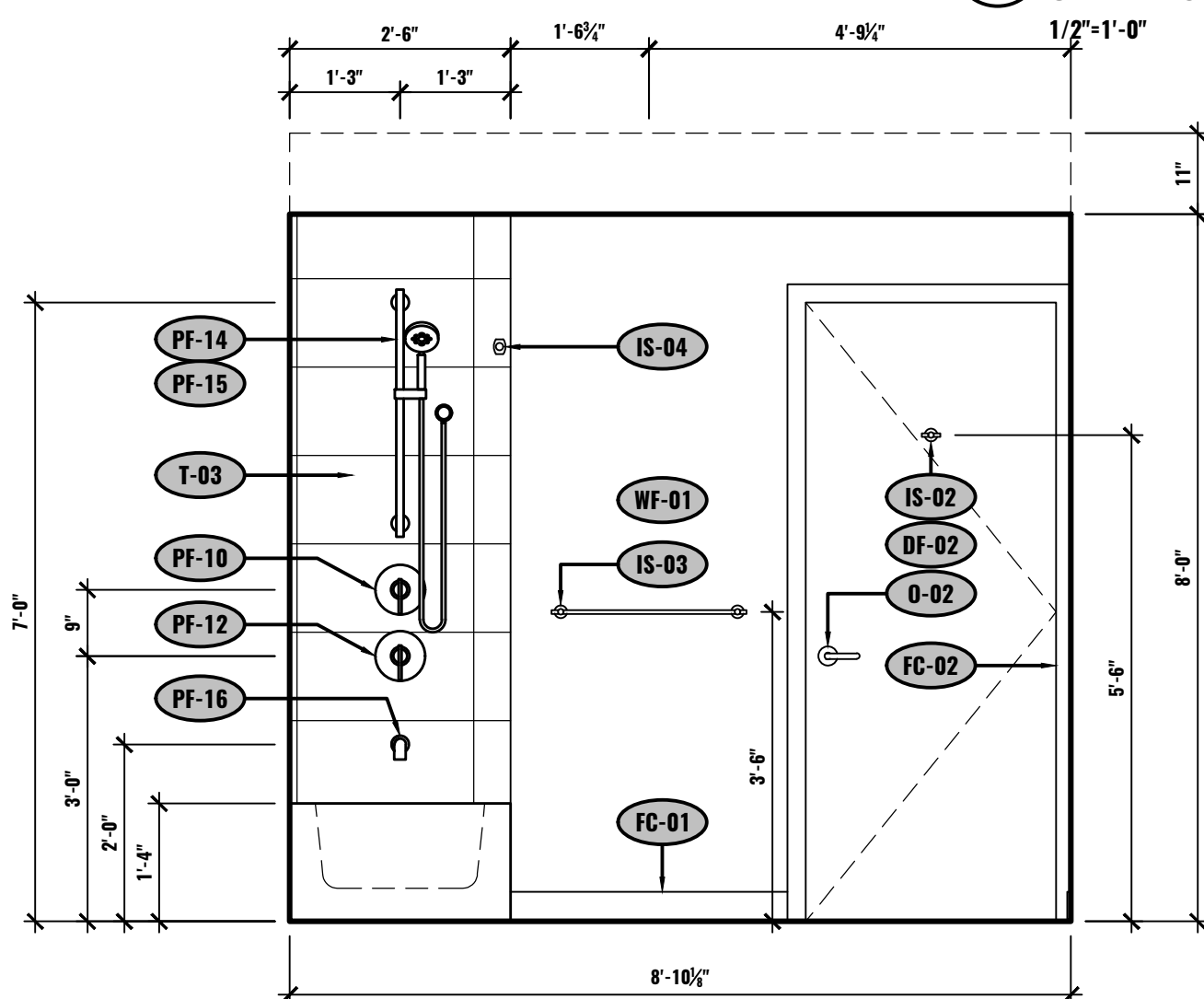
M ELEVATION - BATHROOM UNIT #2-506 1/2"=1'-0"
