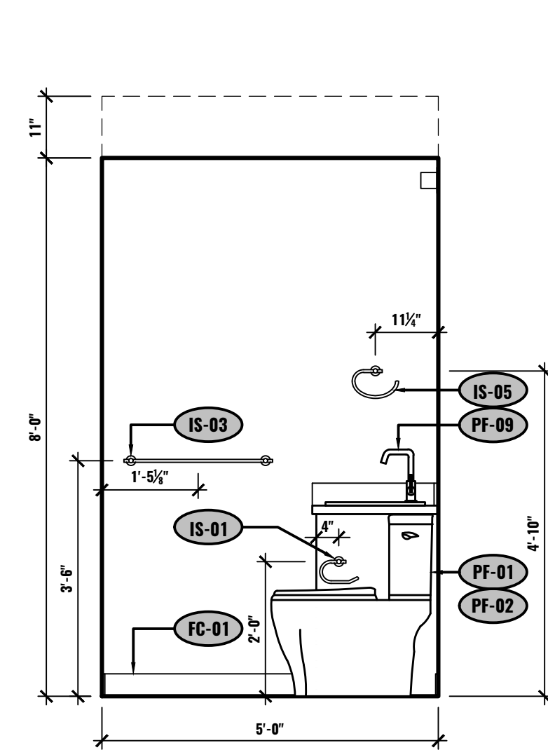
E ELEVATION - BATHROOM UNIT #602 1/2"=1'-0"
