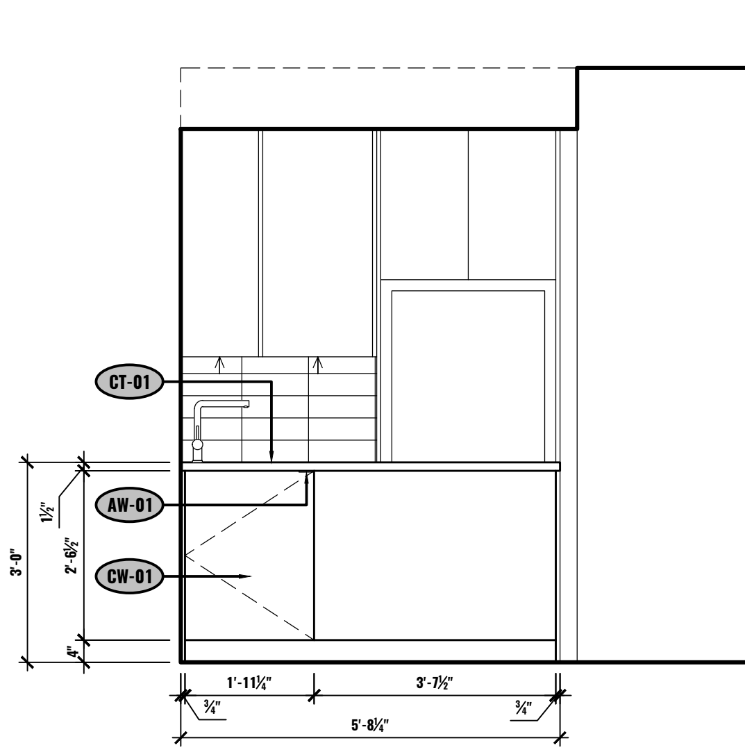
J ELEVATION - KITCHEN UNIT #2-505 1/2"=1'-0"
