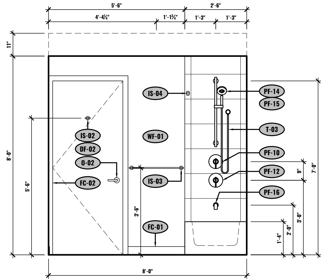
I ELEVATION - BATHROOM UNIT #2-507 1/2"=1'-0"
