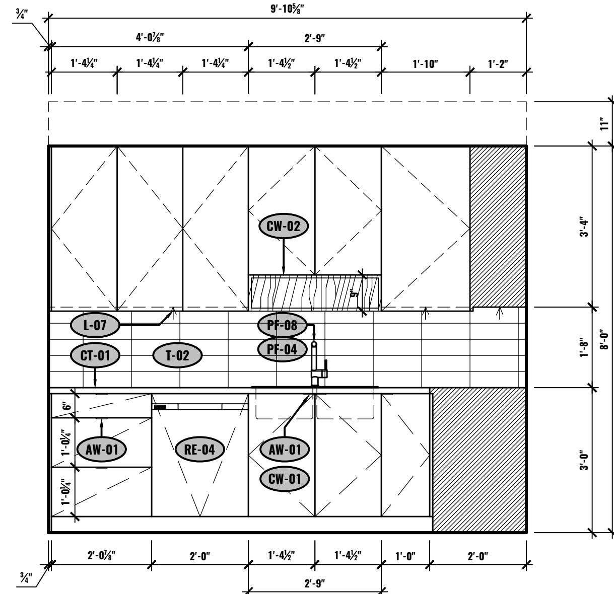
B ELEVATION - KITCHEN UNIT #604 1/2"=1'-0"
