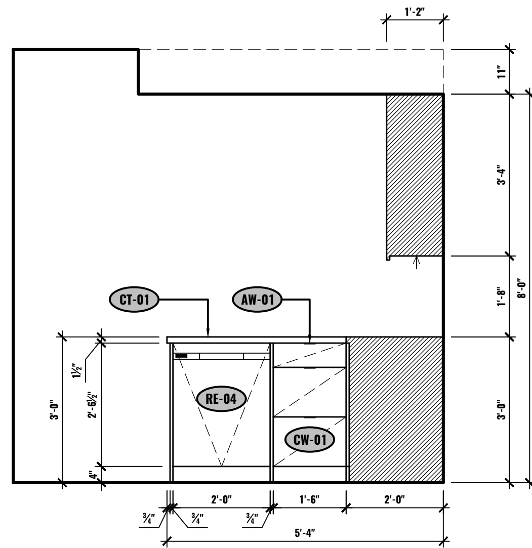
K ELEVATION - KITCHEN UNIT #2-505 1/2"=1'-0"
