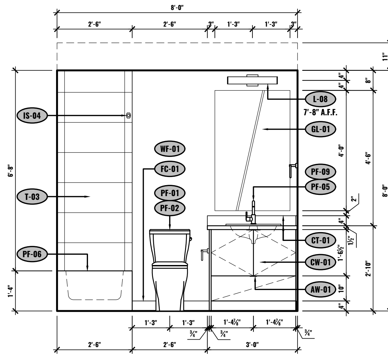
G ELEVATION - BATHROOM UNIT #2-507 1/2"=1'-0"
