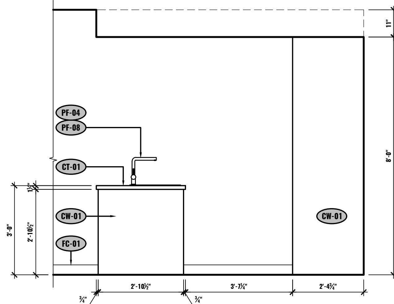
D ELEVATION - KITCHEN UNIT #601 1/2"=1'-0"
