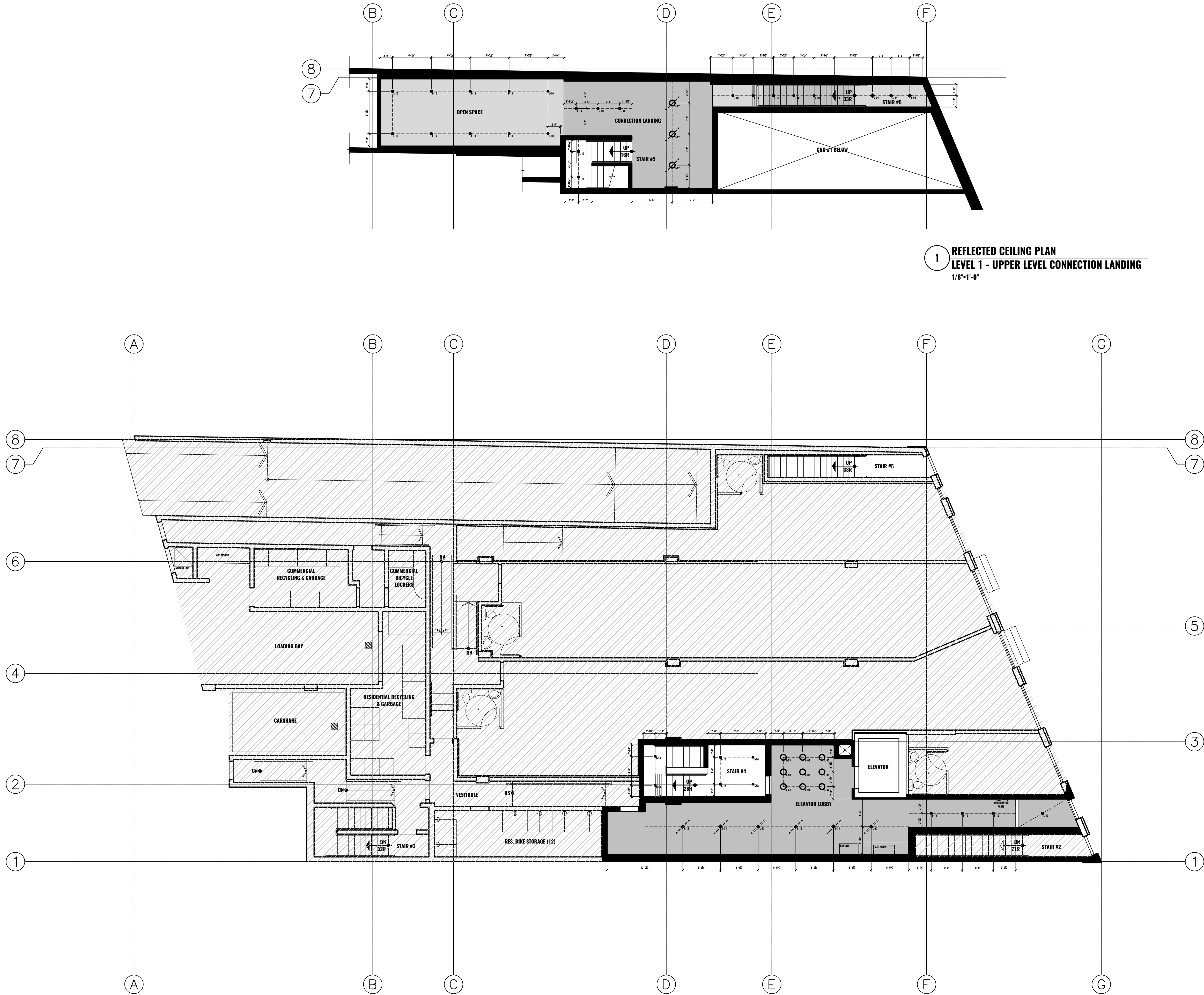
1 REFLECTED CEILING PLAN LEVEL 1 1/8"=1'-0"
