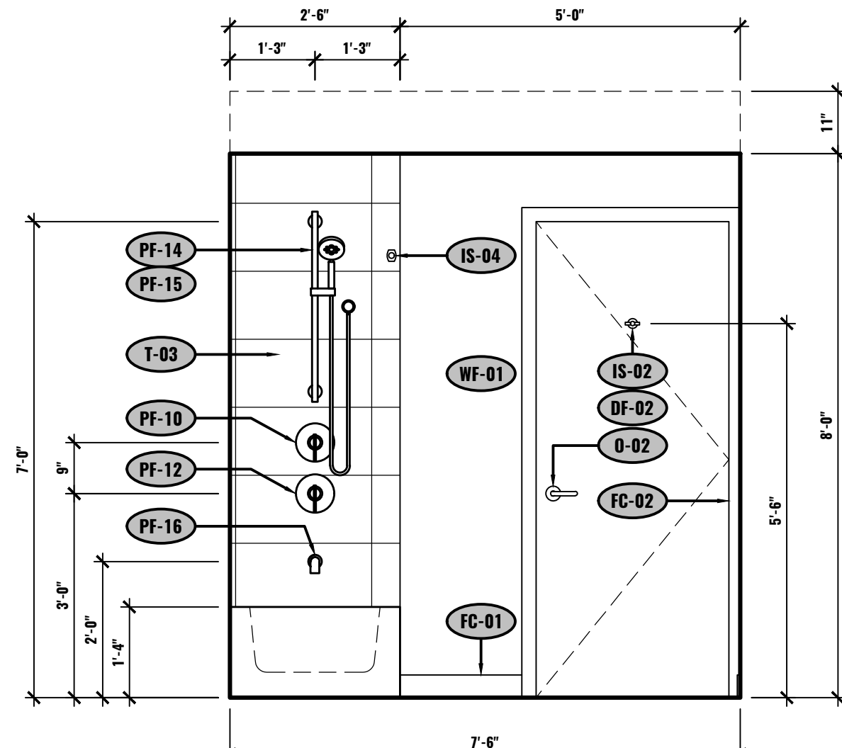
J ELEVATION - BATHROOM UNIT #2-502 1/2"=1'-0"
