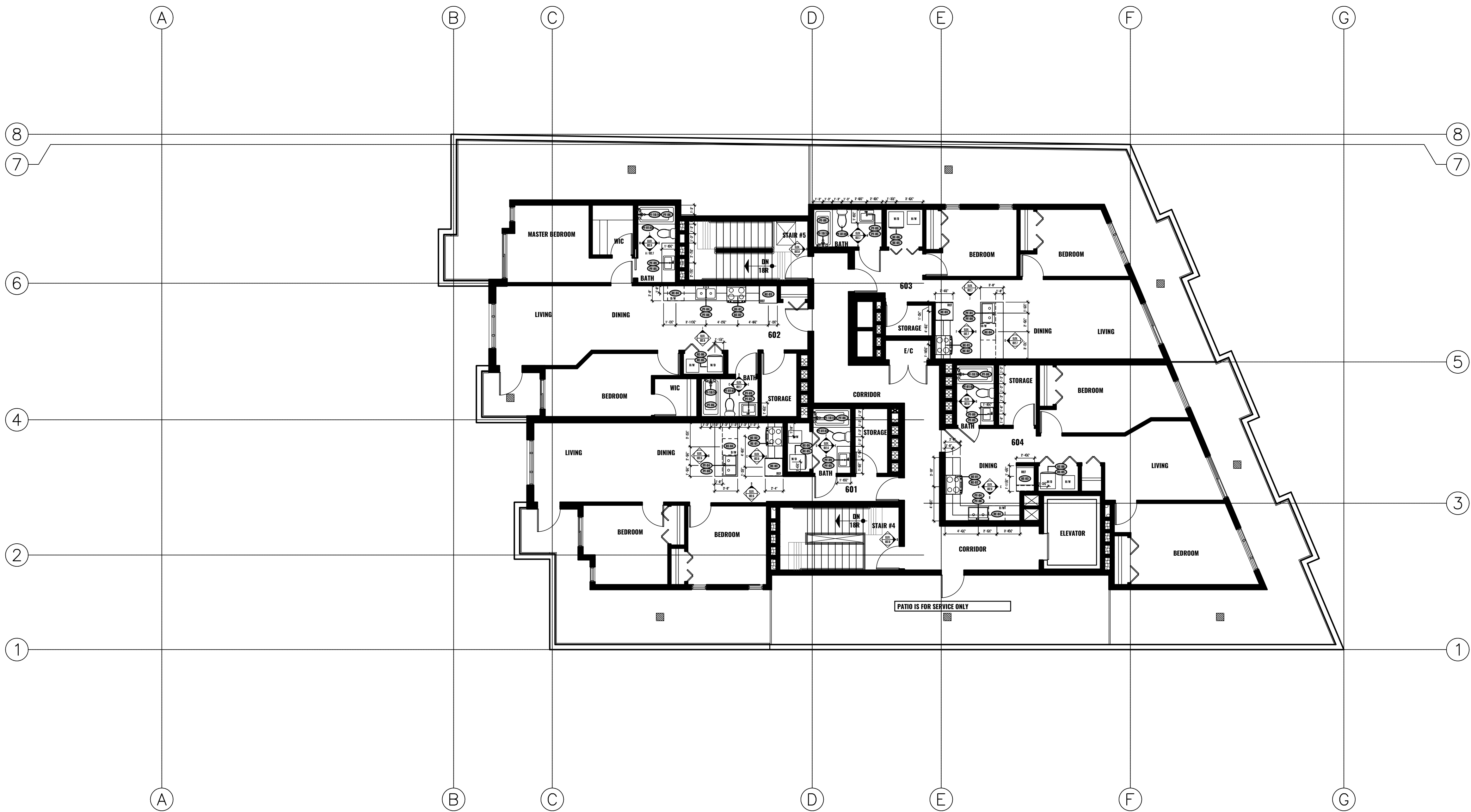
3 CONSTRUCTION PLAN LEVEL 6 1/8"=1'-0"
