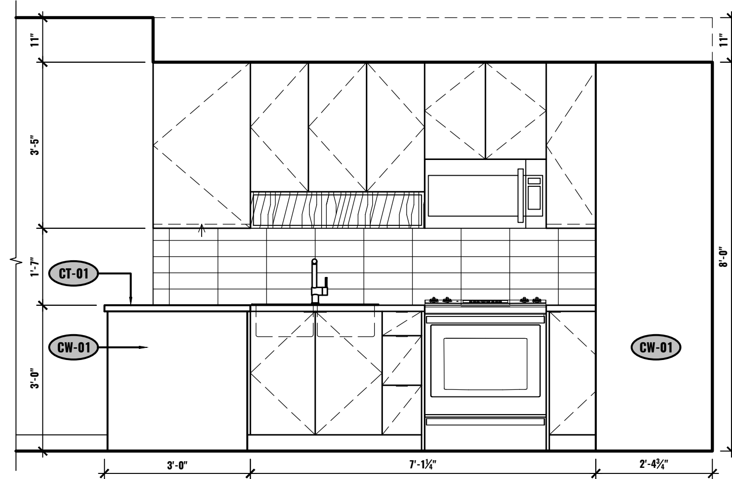
B ELEVATION - KITCHEN UNIT #2-504 1/2"=1'-0"
