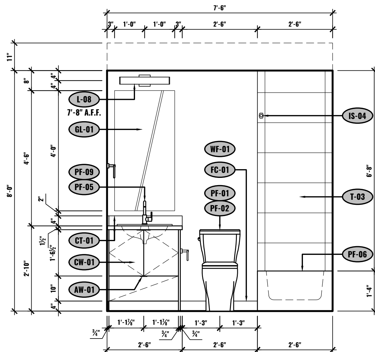
B ELEVATION - BATHROOM UNIT #602 1/2"=1'-0"
