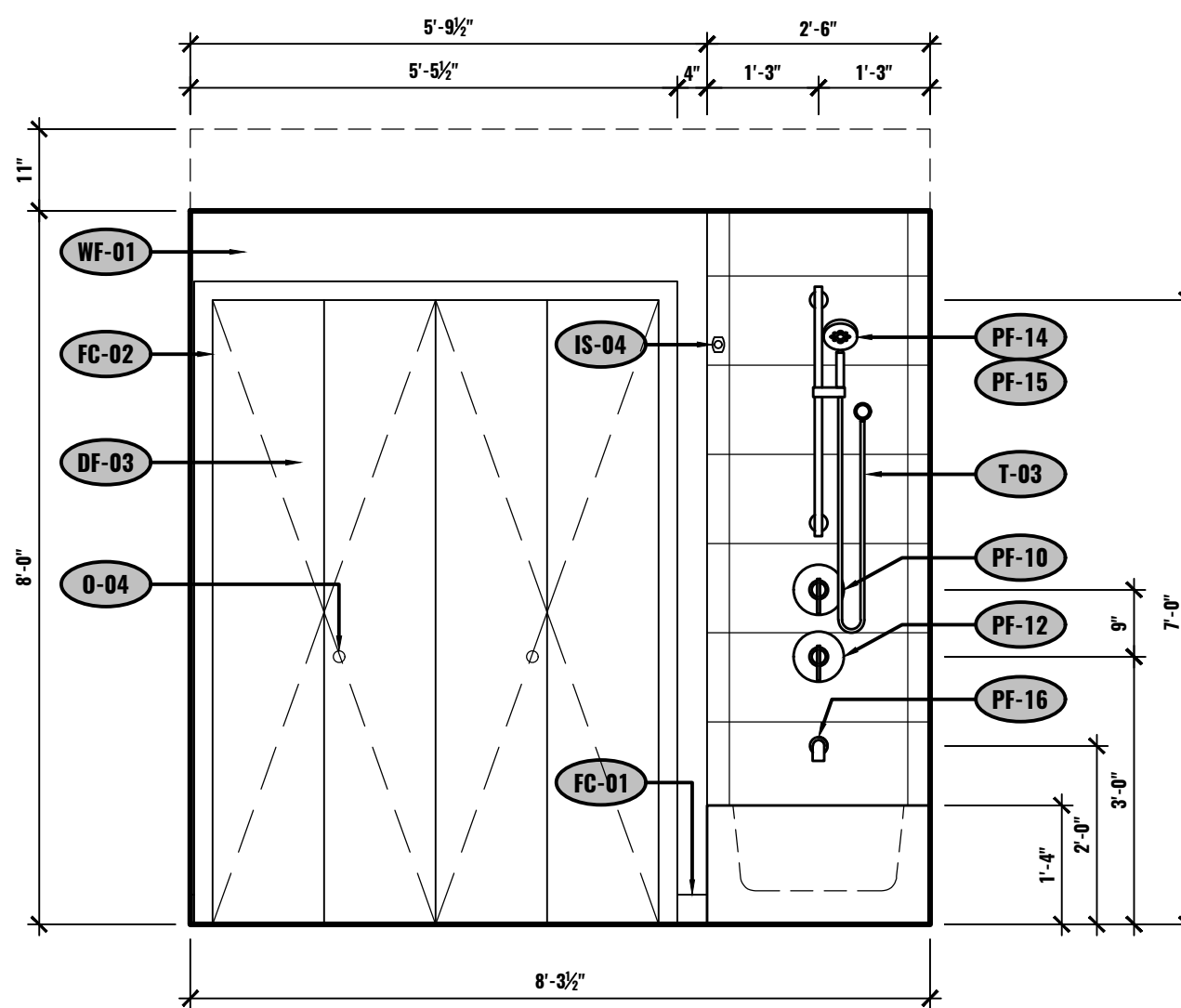
G ELEVATION - BATHROOM UNIT #601 1/2"=1'-0"
