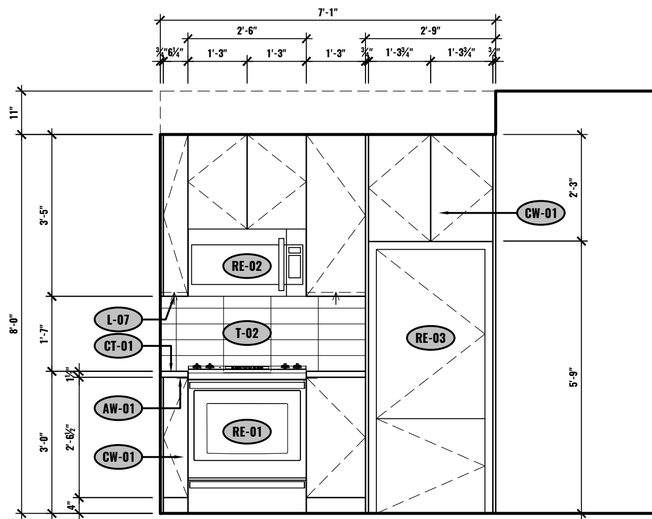
A ELEVATION - KITCHEN UNIT #601 1/2"=1'-0"
