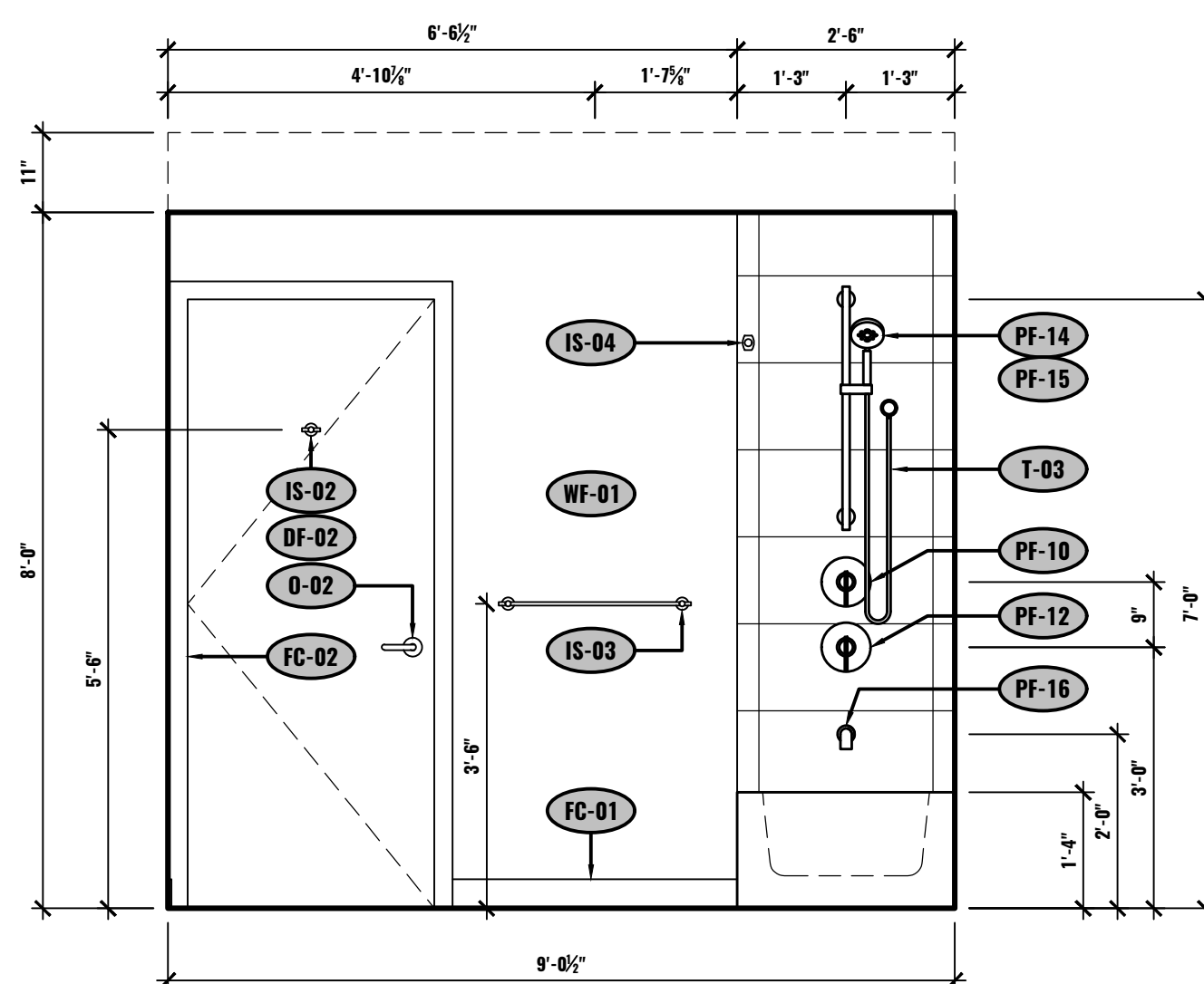
M ELEVATION - BATHROOM UNIT #603 1/2"=1'-0"
