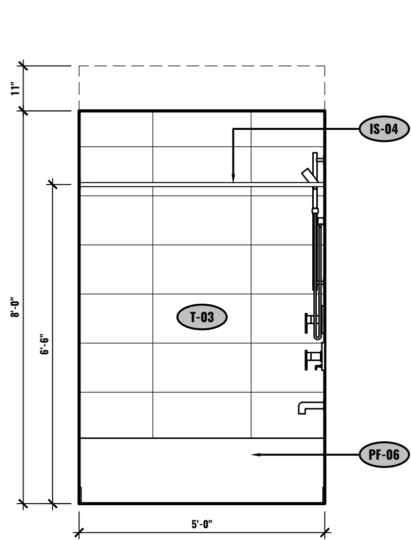
I ELEVATION - BATHROOM UNIT #2-502 1/2"=1'-0"
