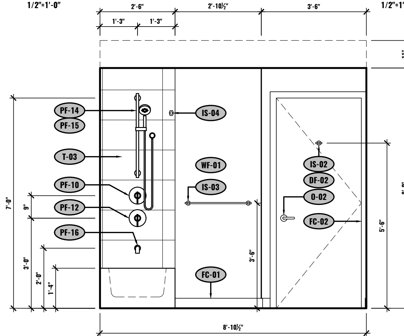
M ELEVATION - BATHROOM UNIT #2-504 1/2"=1'-0"
