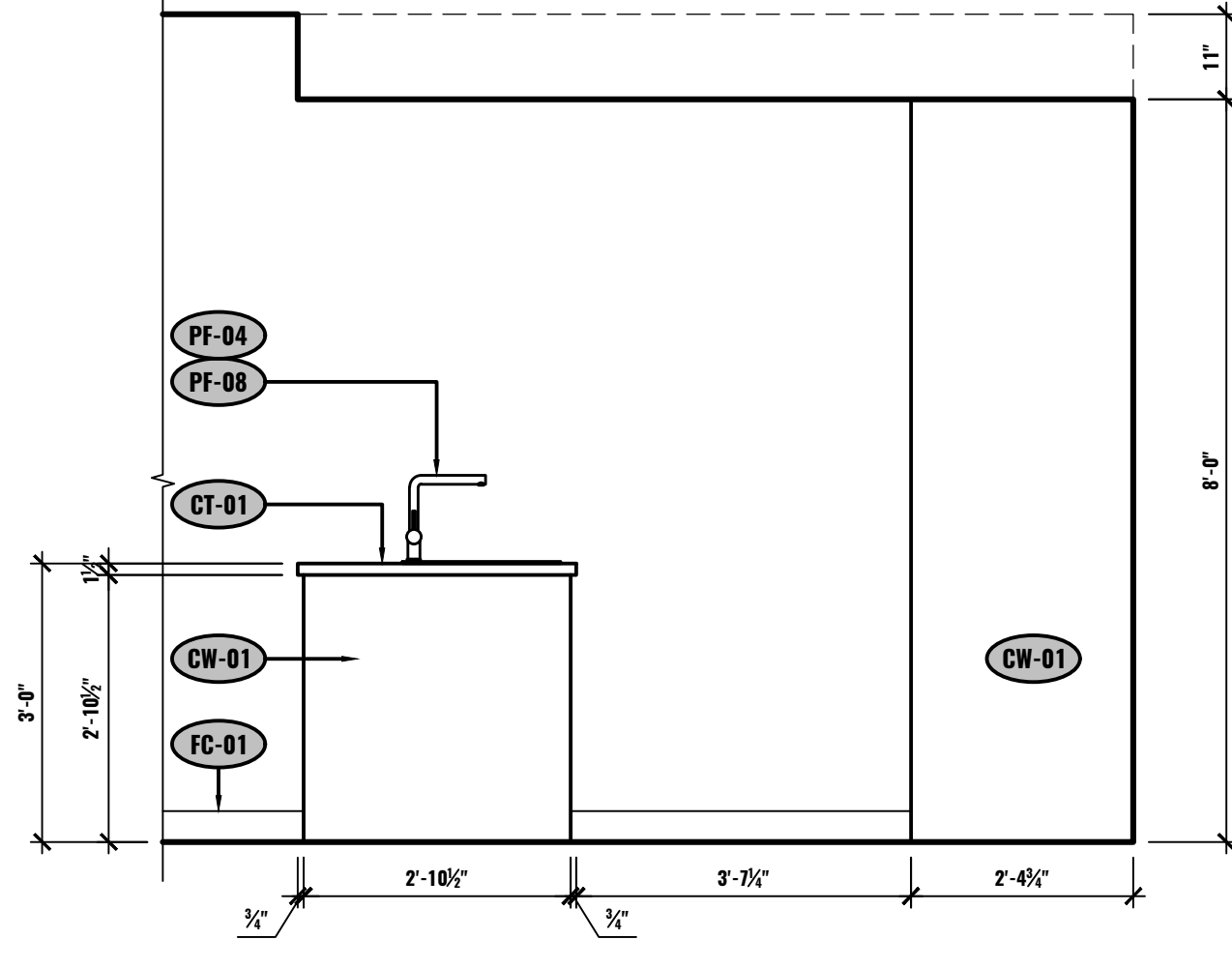
J ELEVATION - KITCHEN UNIT #603 1/2"=1'-0"
