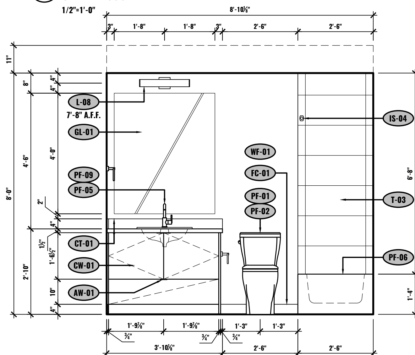
K ELEVATION - BATHROOM UNIT #2-506 1/2"=1'-0"
