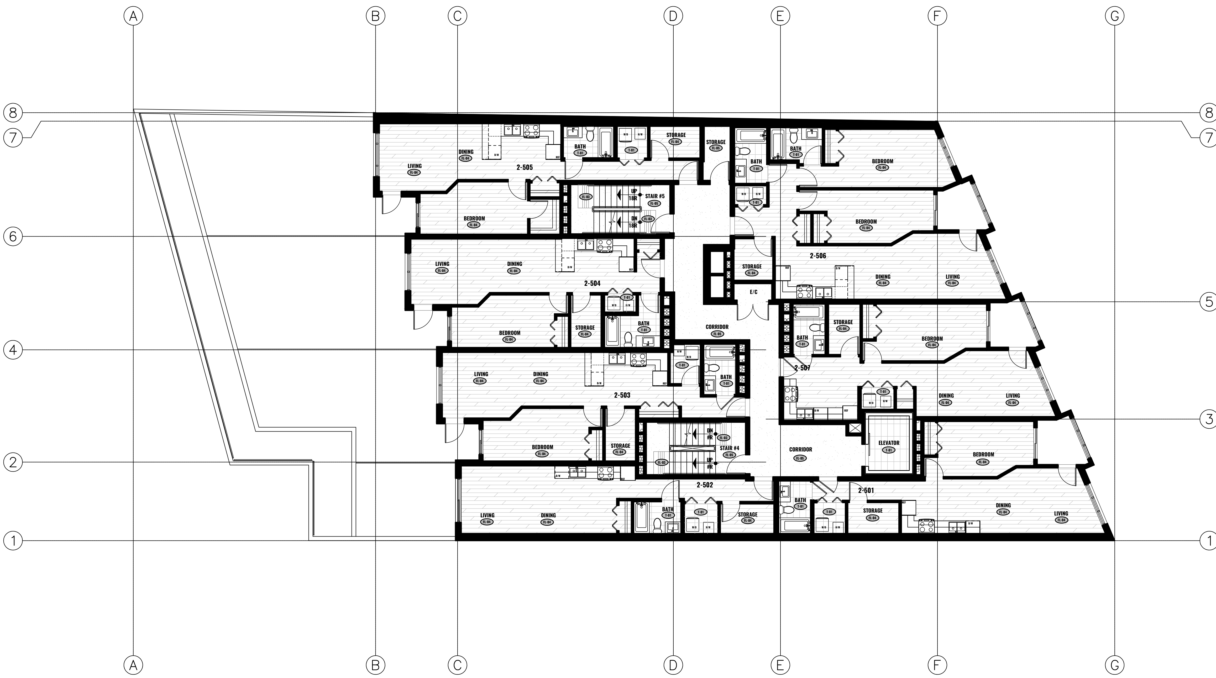
2 FINISHES PLAN LEVELS 2-5 1/8"=1'-0"
