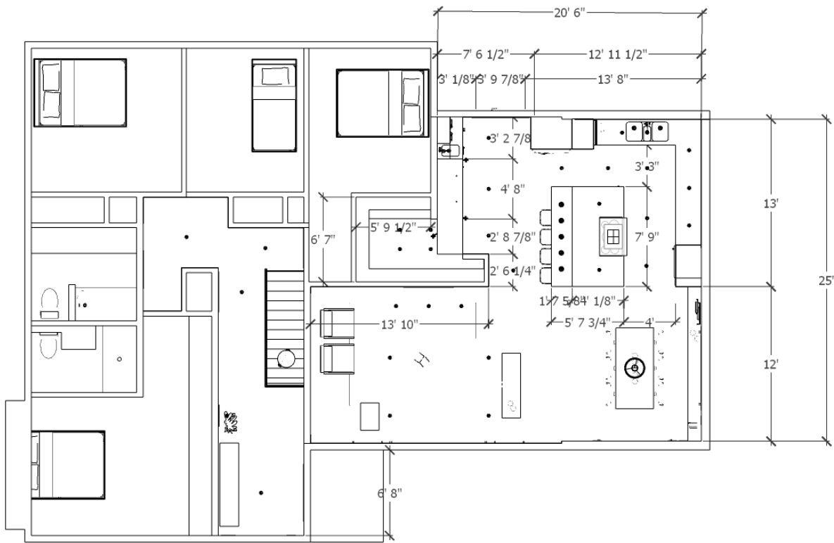
MAIN LEVEL FLOOR PLAN | PROPOSED
