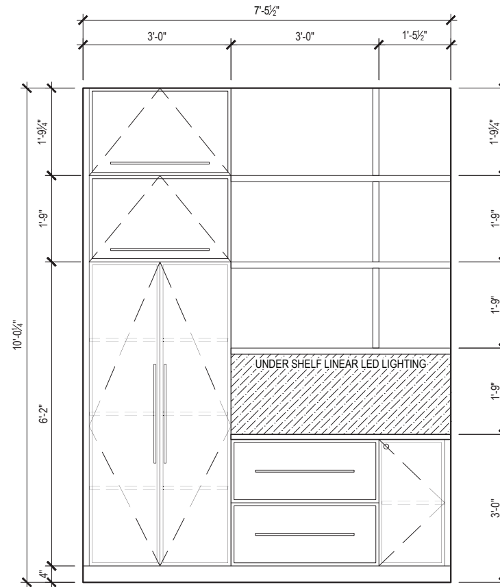
G PANTRY - WEST ELEVATION xxx 3/8" = 1'-0"
