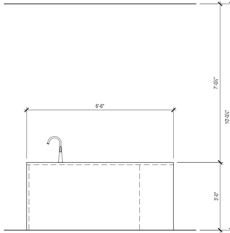
KITCHEN ISLAND - WEST ELEVATION
