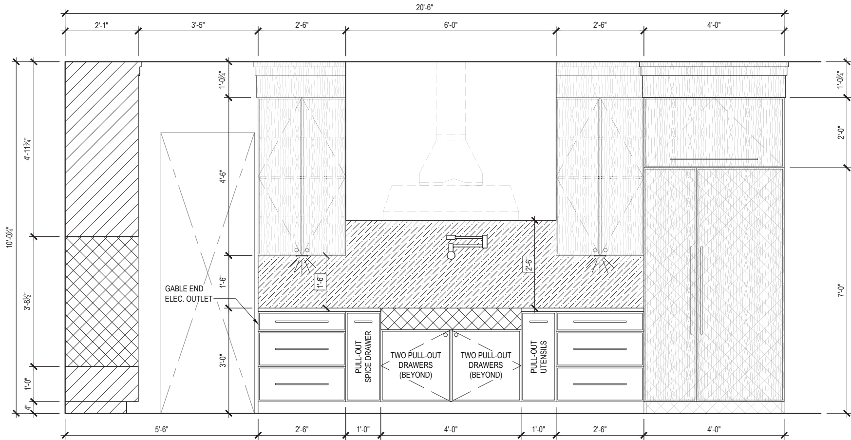
B KITCHEN - SOUTH ELEVATION xxx 3/8" = 1'-0"
