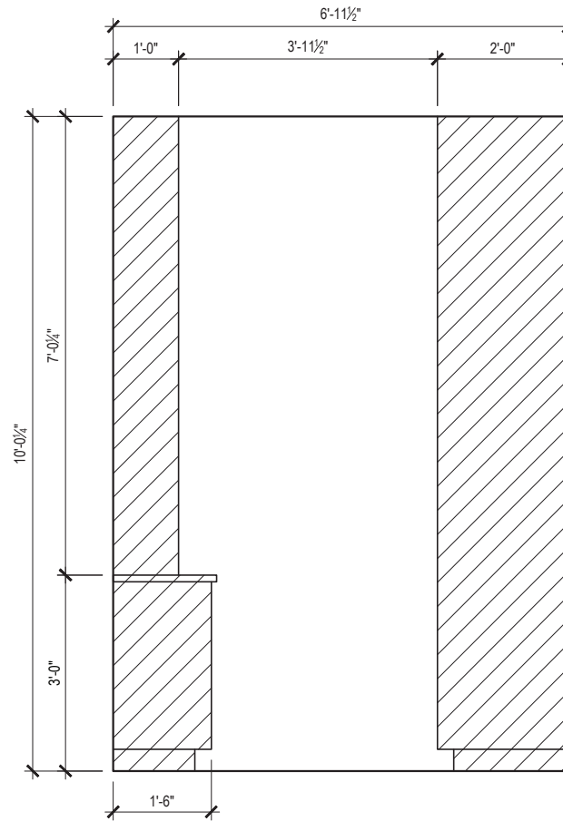
1 PANTRY - SOUTH ELEVATION xxx 3/8" = 1'-0"
