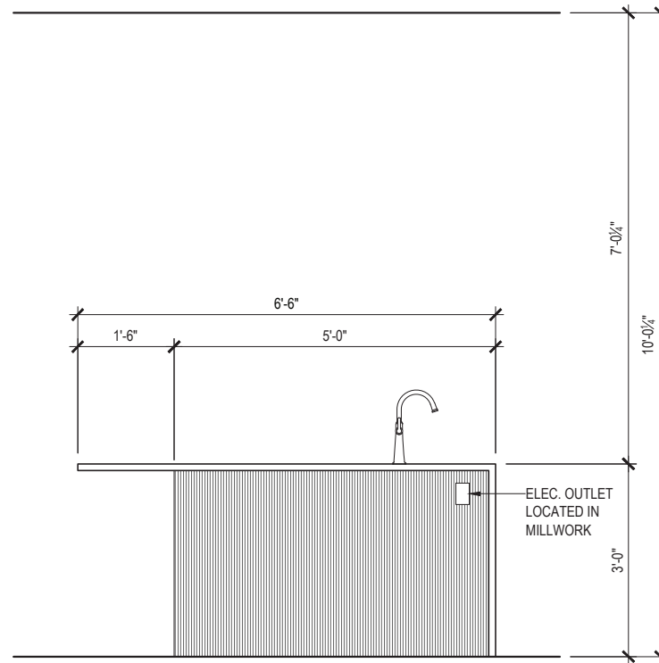
E KITCHEN ISLAND - EAST ELEVATION xxx 3/8" = 1'-0"
