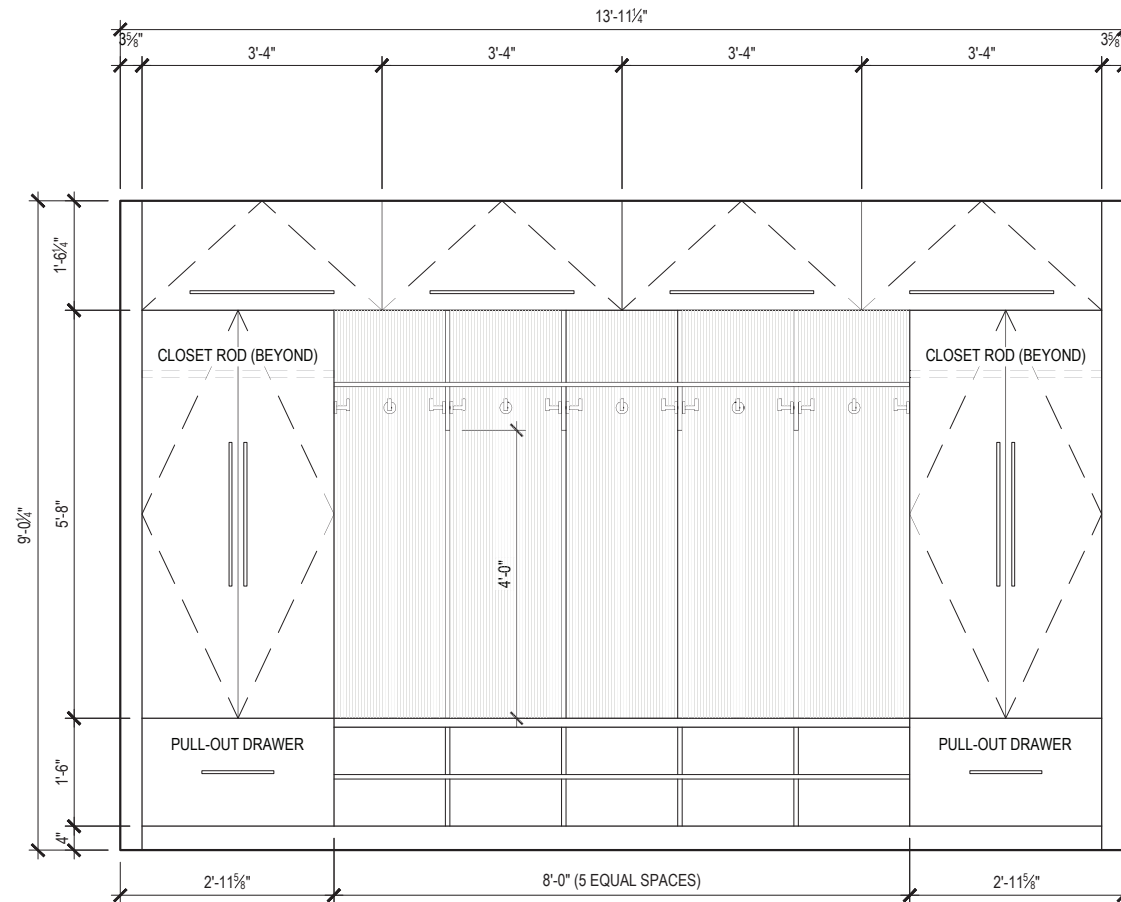
MUDROOM - NORTH ELEVATION M xxx 3/8" = 1'-0"
