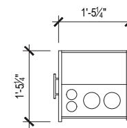
SALON CADDY TOP VIEW
