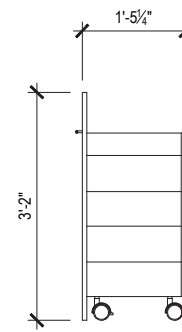
SALON CADDY SIDE VIEW
