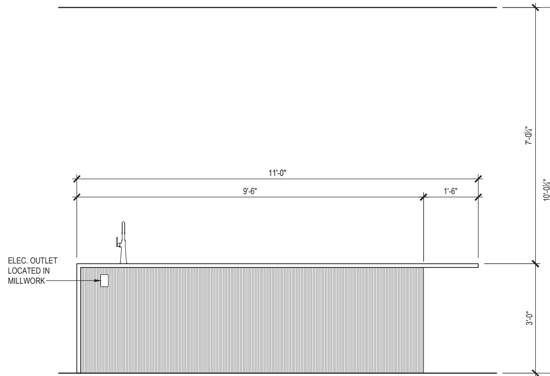
D KITCHEN ISLAND - SOUTH ELEVATION xxx 3/8" = 1'-0"
