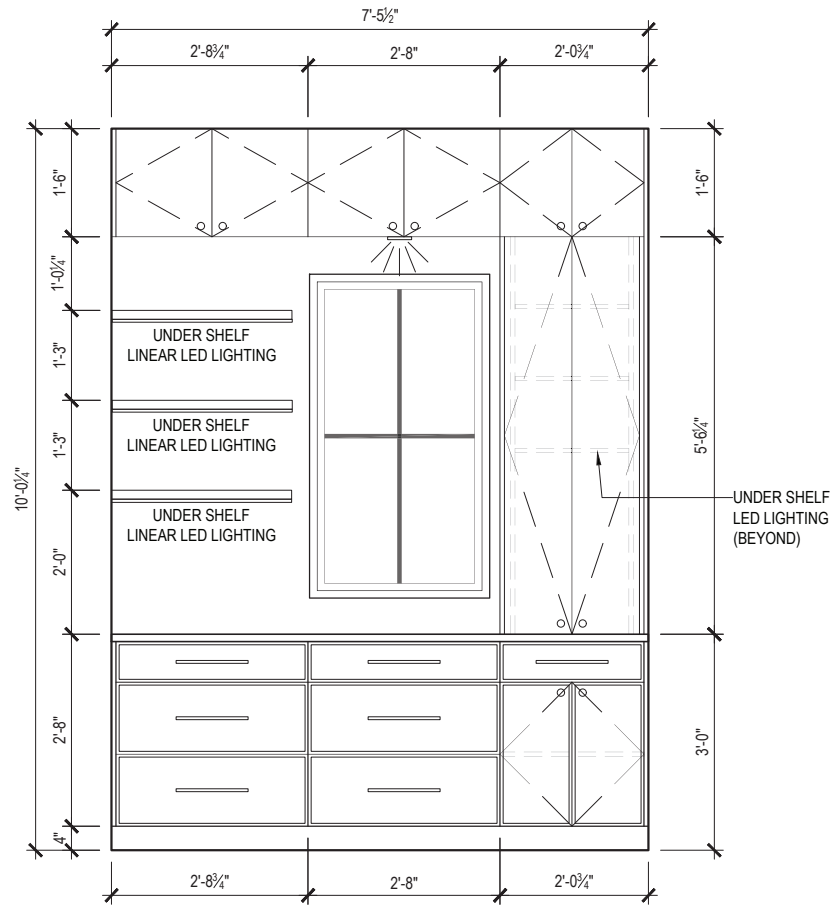
H PANTRY - EAST ELEVATION xxx 3/8" = 1'-0"
