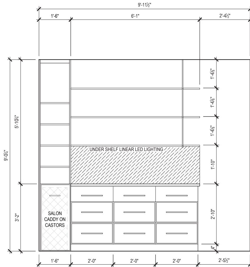
J xxx 3/8" = 1'-0" SALON - SOUTH ELEVATION
