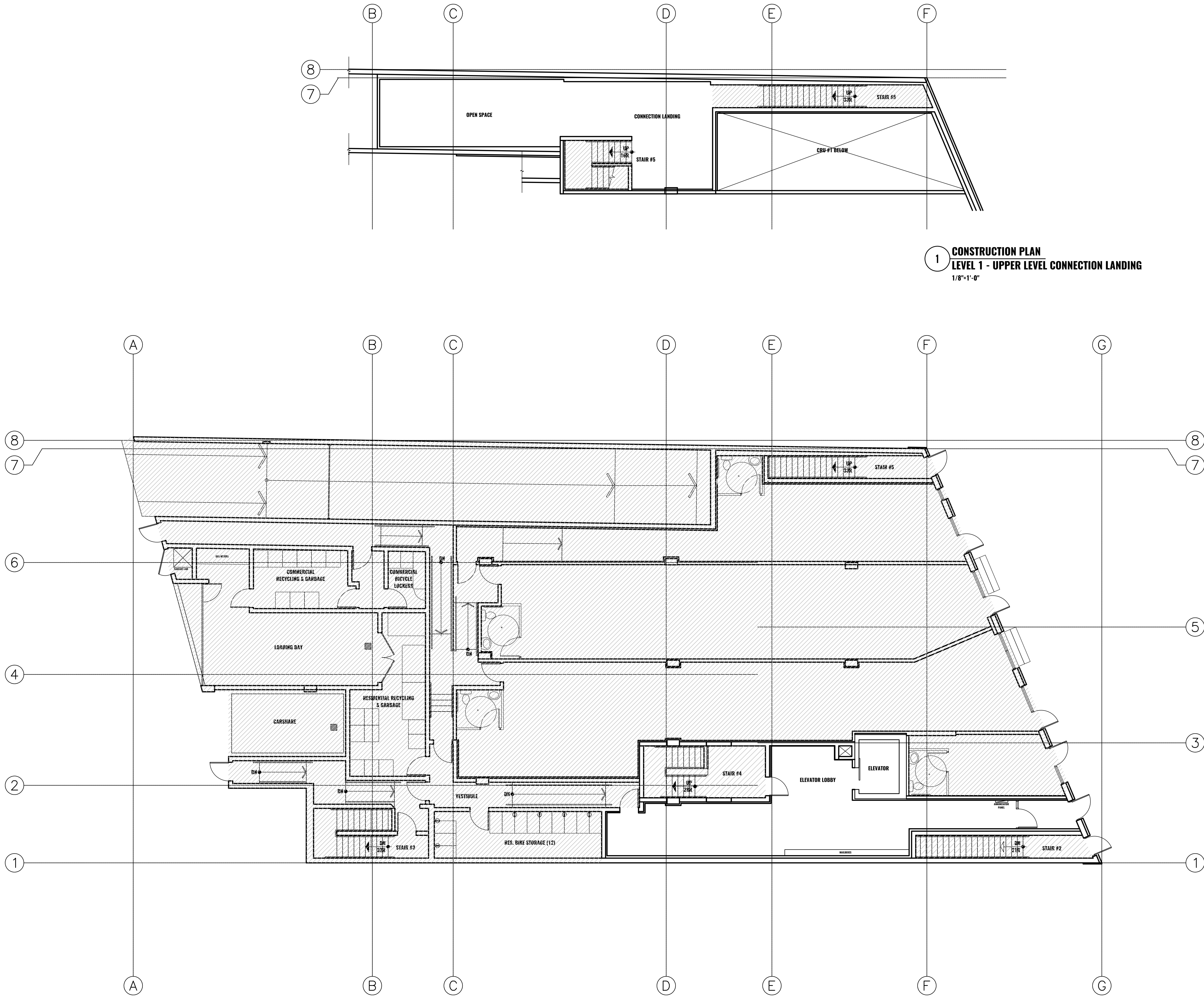
1 CONSTRUCTION PLAN LEVEL 1 1/8"=1'-0"
