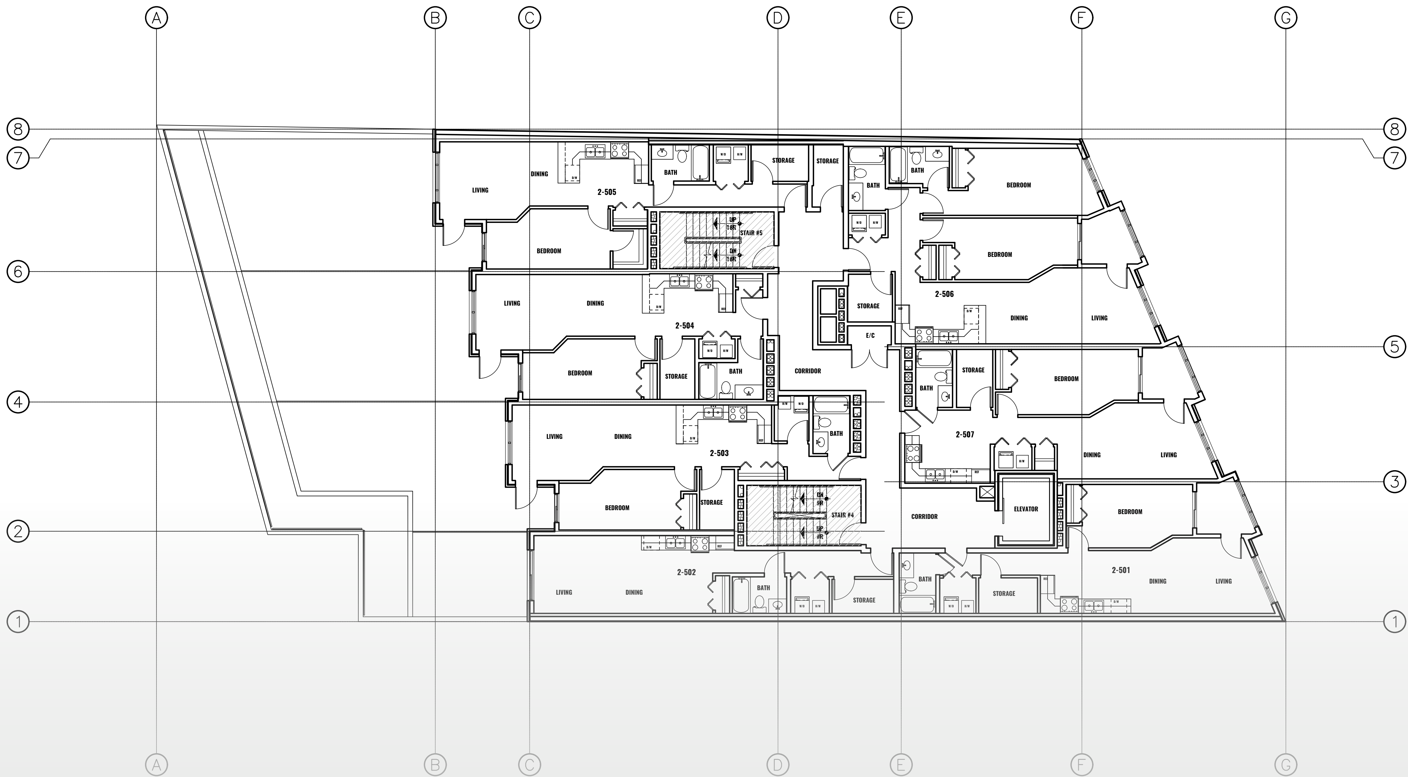
2 CONSTRUCTION PLAN LEVELS 2-5 1/8"=1'-0"
