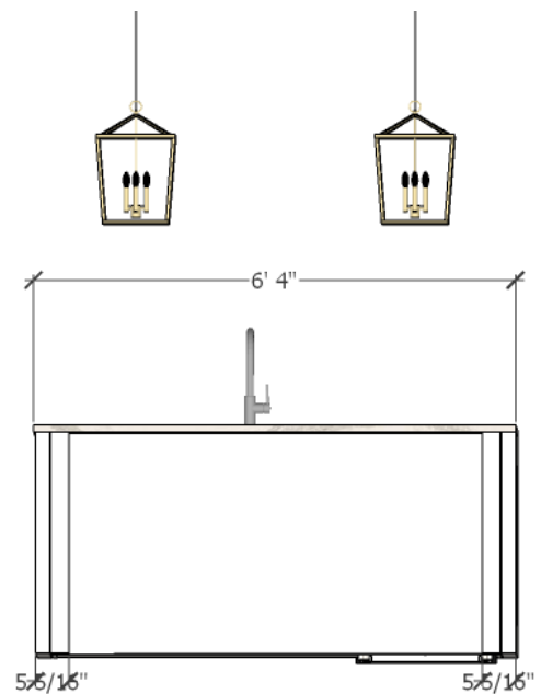
WEST ISLAND ELEVATION KITCHEN CABINET GENERAL LAYOUT DIMENSIONS- UNITS D | B
