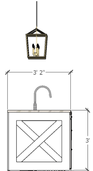
NORTH + SOUTH ISLAND ELEVATIONS
