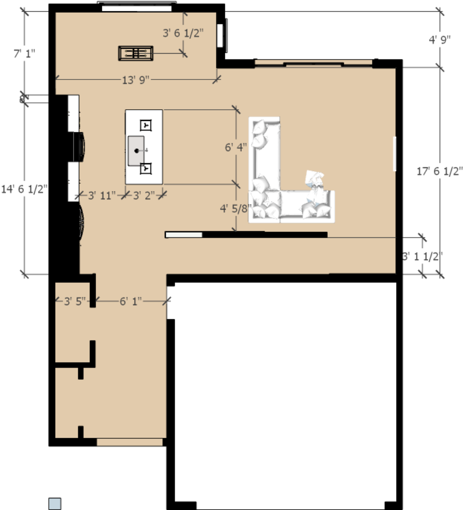
KITCHEN CABINET GENERAL PLAN KITCHEN CABINET GENERAL LAYOUT DIMENSIONS- UNITS D | B
