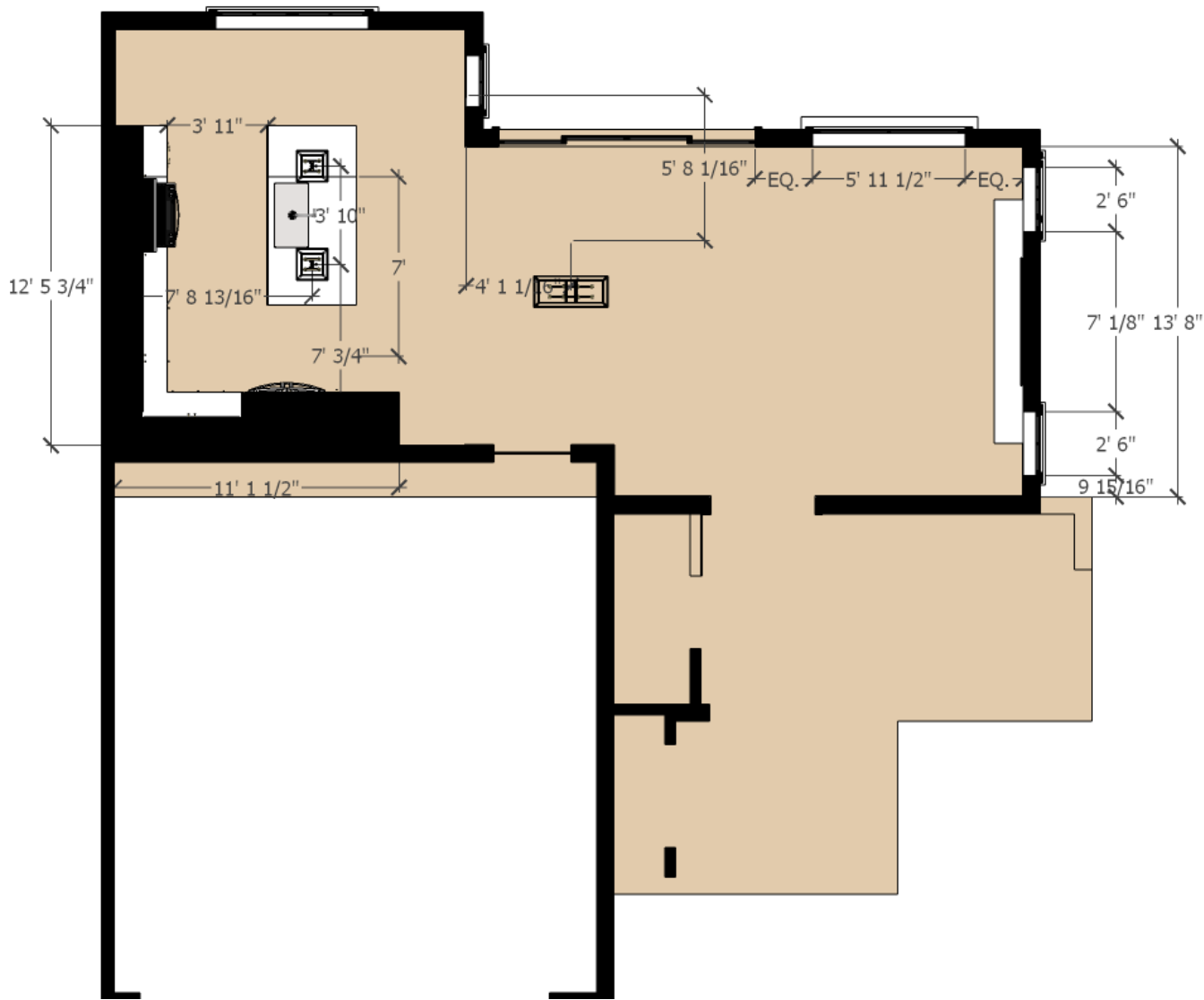
KITCHEN CABINET GENERAL PLAN KITCHEN CABINET GENERAL LAYOUT DIMENSIONS- UNITS C | A
