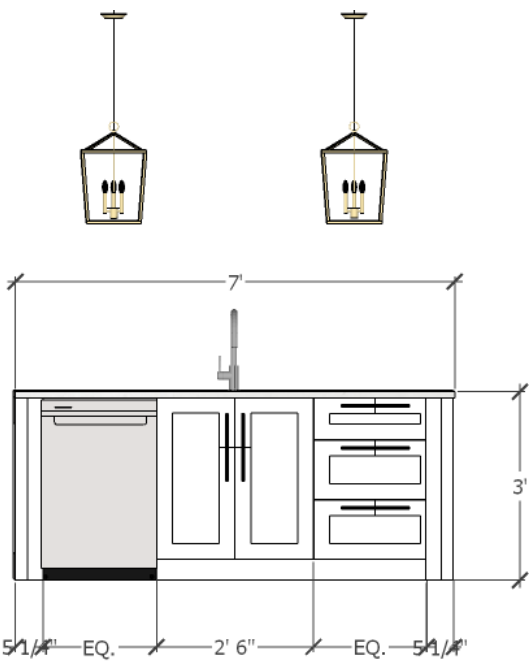
WEST ISLAND ELEVATION
