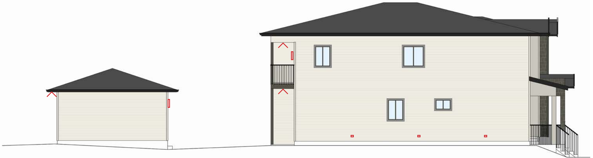
LOT 2 - LEFT (NORTH) ELEVATION
