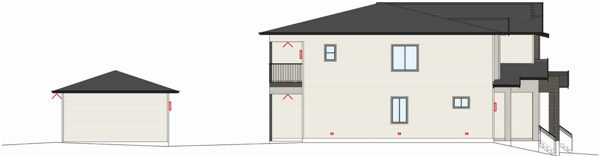
LOT 4 - LEFT (NORTH) ELEVATION
