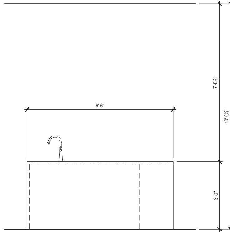
KITCHEN ISLAND - WEST ELEVATION
