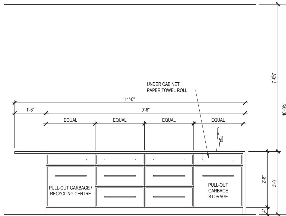
C KITCHEN ISLAND - NORTH ELEVATION xxx 3/8" = 1'-0"
