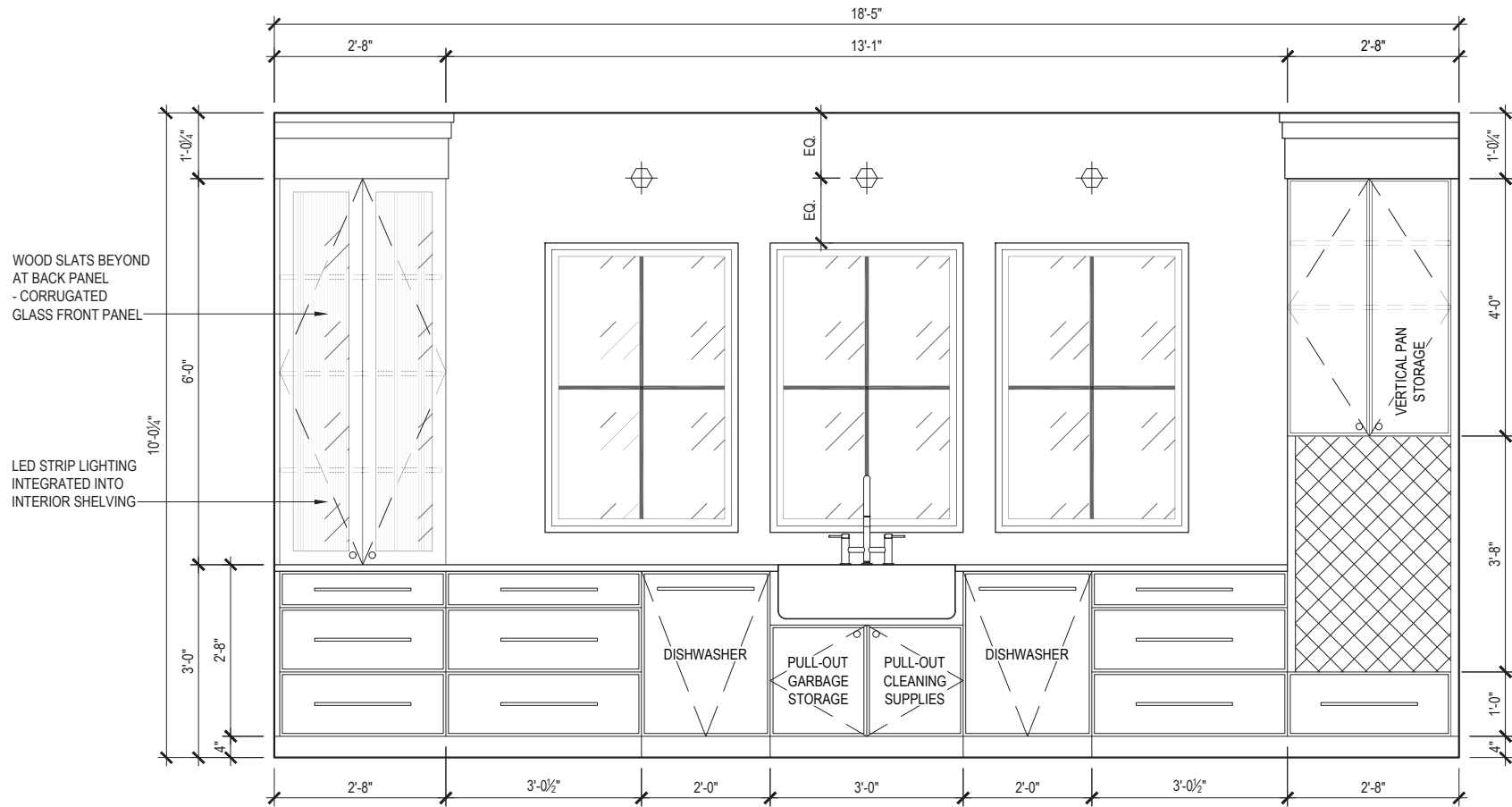
A xxx KITCHEN - EAST ELEVATION 3/8" = 1'-0"
