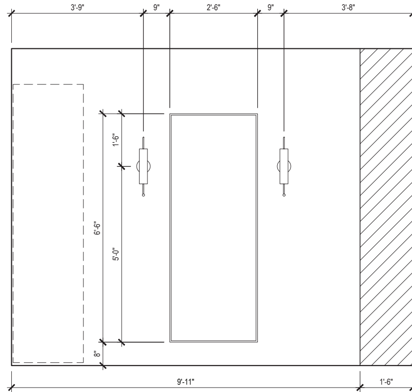
K xxx SALON - EAST ELEVATION 3/8" = 1'-0"
