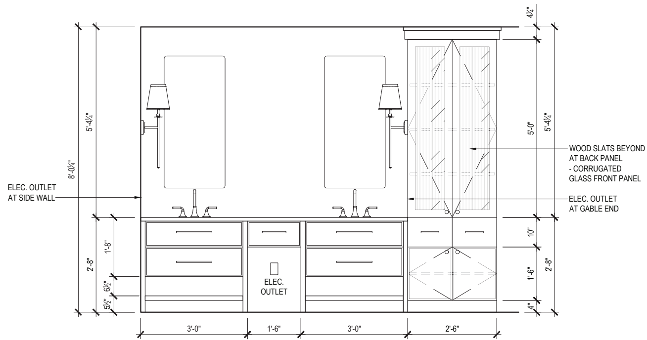
ENSUITE - NORTH ELEVATION L xxx 3/8" = 1'-0"
