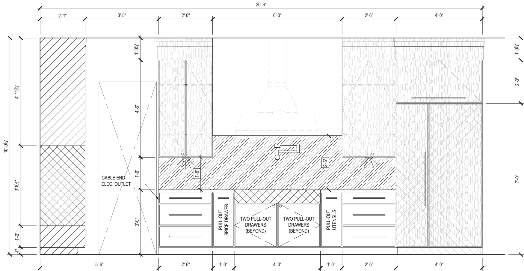
B KITCHEN - SOUTH ELEVATION xxx 3/8" = 1'-0"
