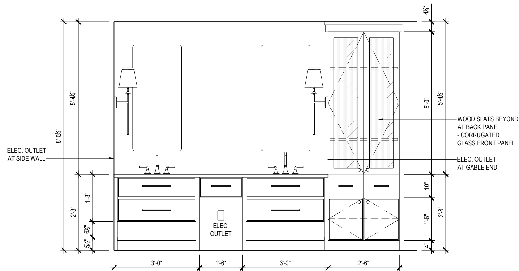
L ENSUITE - NORTH ELEVATION xxx 1/2" = 1'-0"
