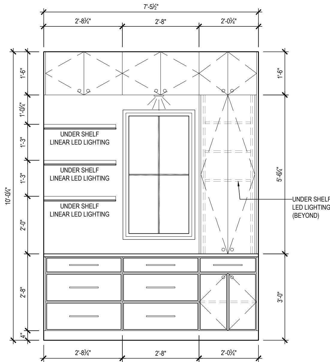
H PANTRY - EAST ELEVATION xxx 1/2" = 1'-0"
