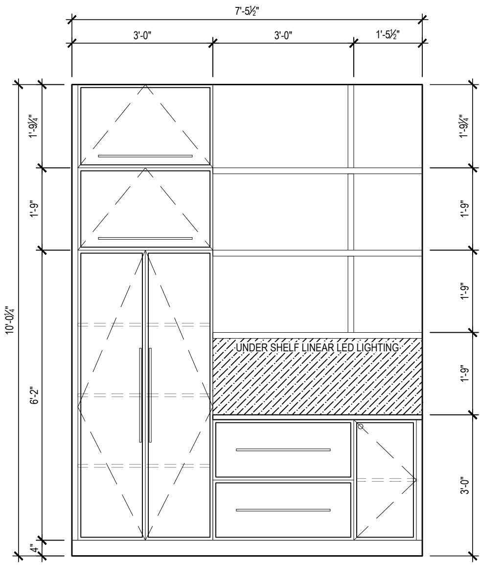
G PANTRY - WEST ELEVATION xxx 1/2" = 1'-0"
