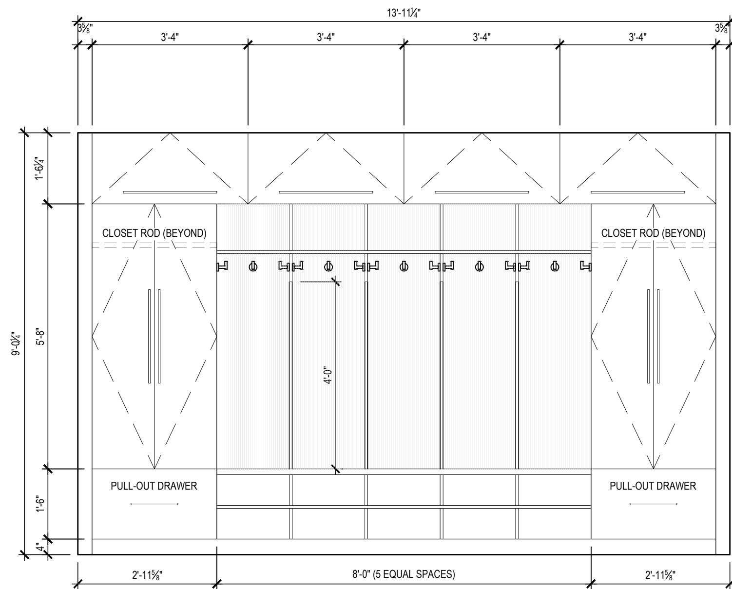
M MUDROOM - NORTH ELEVATION xxx 1/2" = 1'-0"
