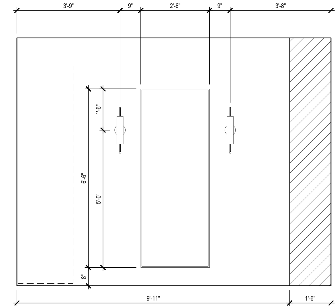
K SALON - EAST ELEVATION xxx 1/2" = 1'-0"
