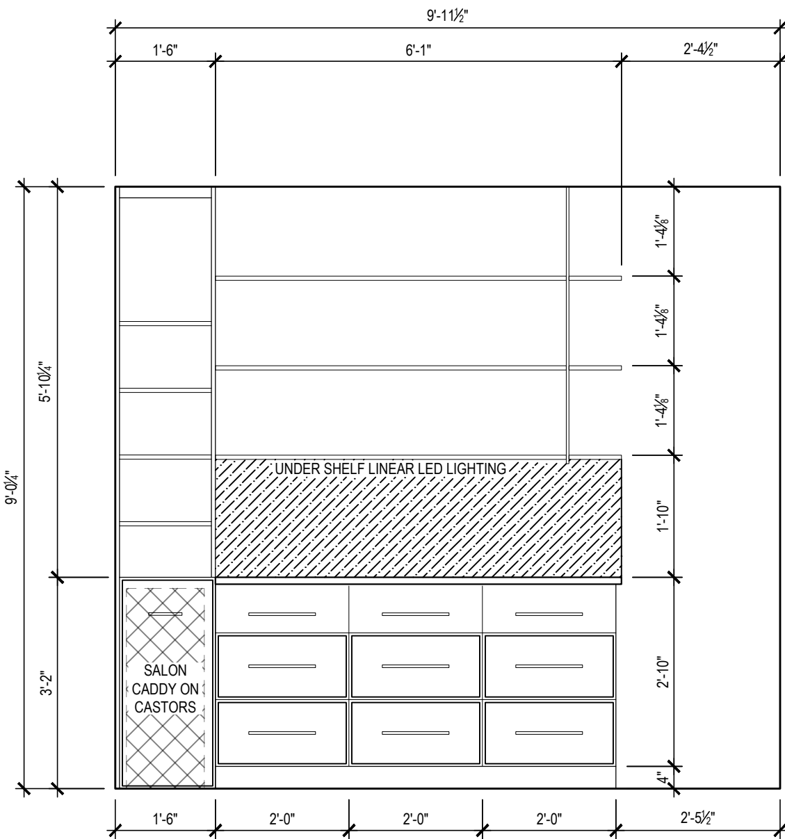
J SALON - SOUTH ELEVATION xxx 1/2" = 1'-0"
