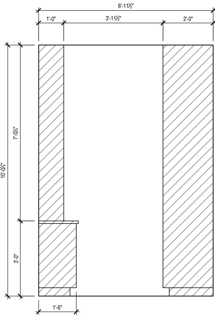
I PANTRY - SOUTH ELEVATION xxx 1/2" = 1'-0"
