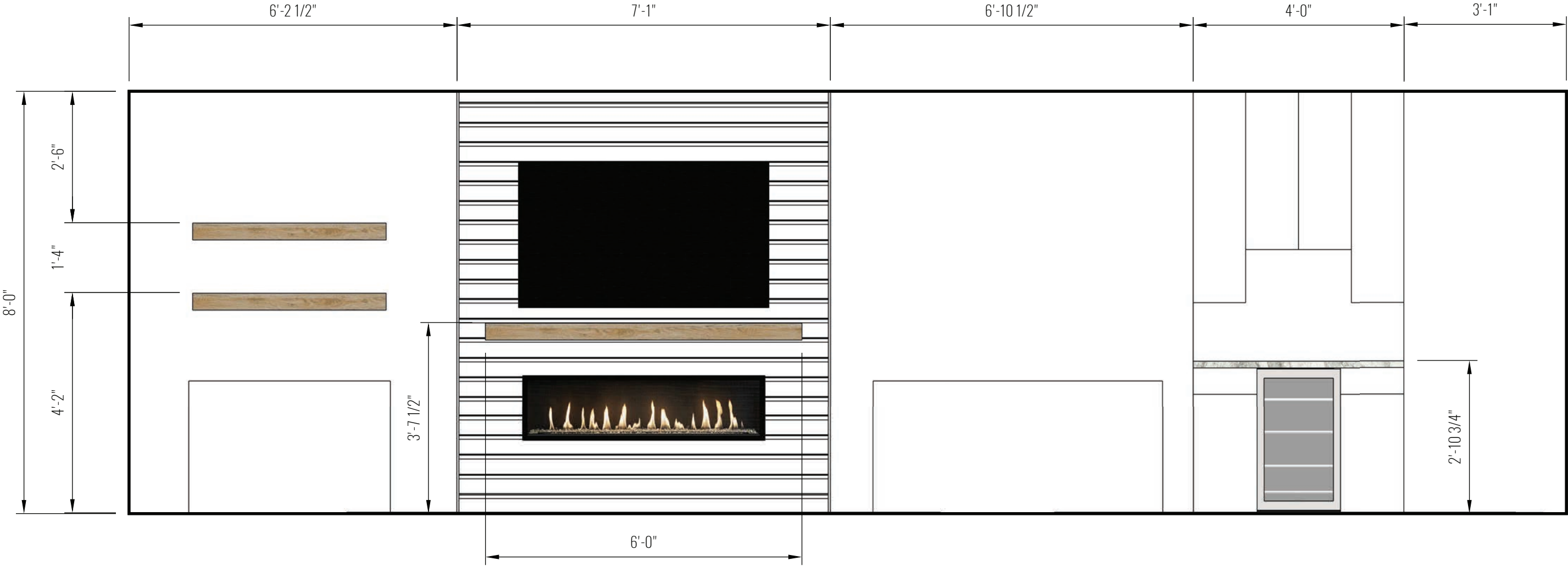
FIREPLACE ELEVATION 1/2" = 1'-0"
