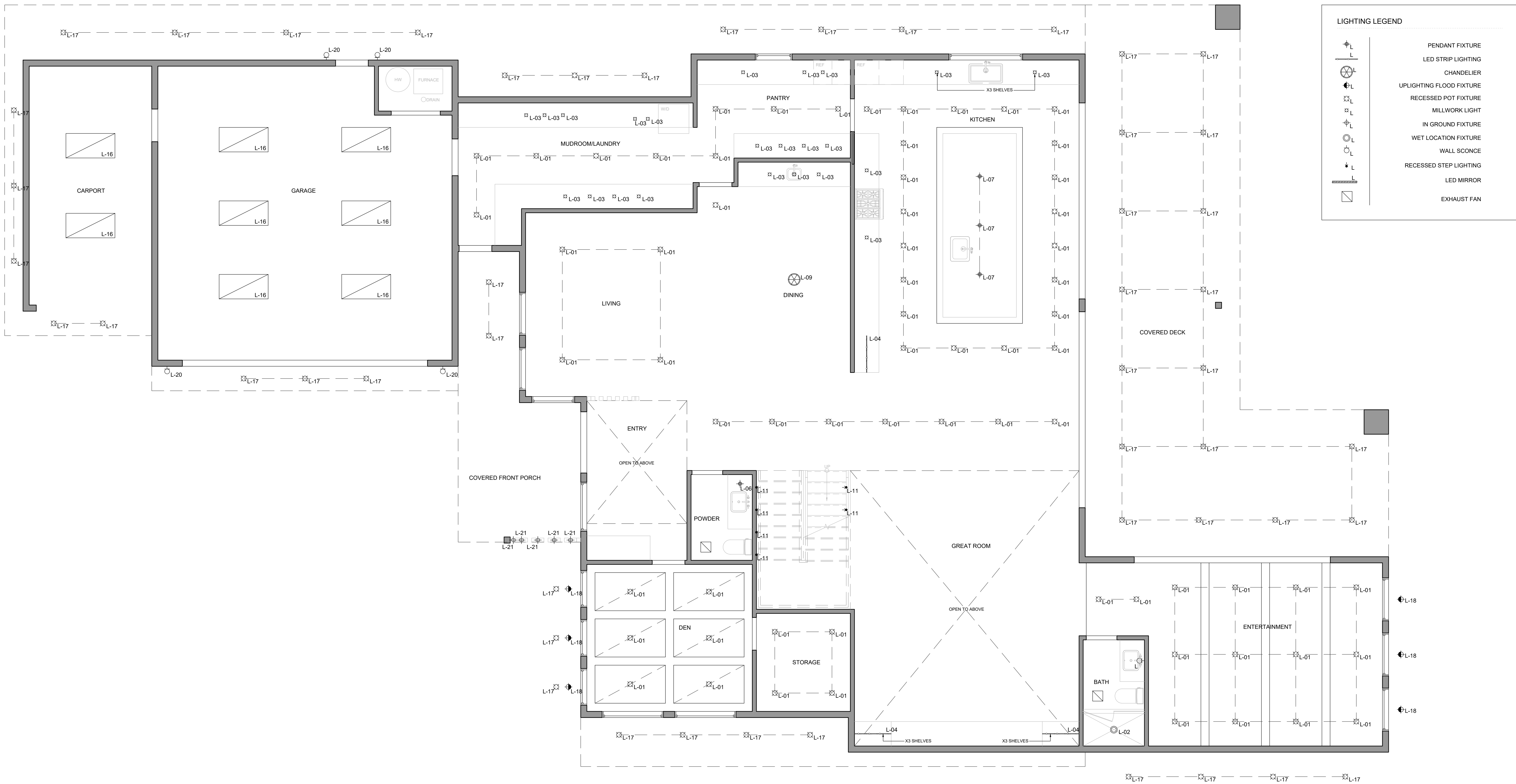
MAIN FLOOR - REFLECTED CEILING PLAN ID1.0.1 SCALE: 1/4" = 1'-0"
