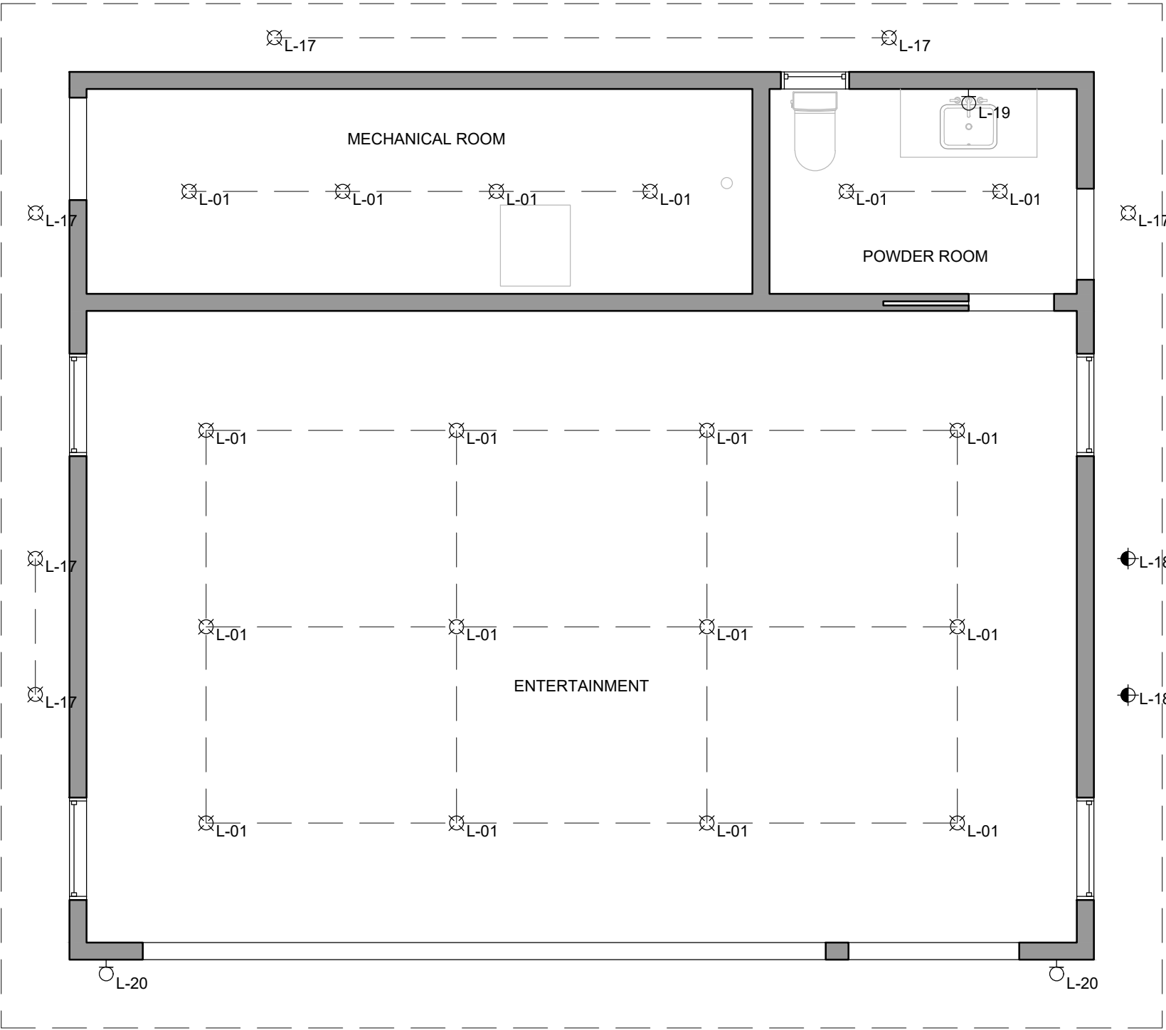
ACCESSORY BUILDING - REFLECTED CEILING PLAN
