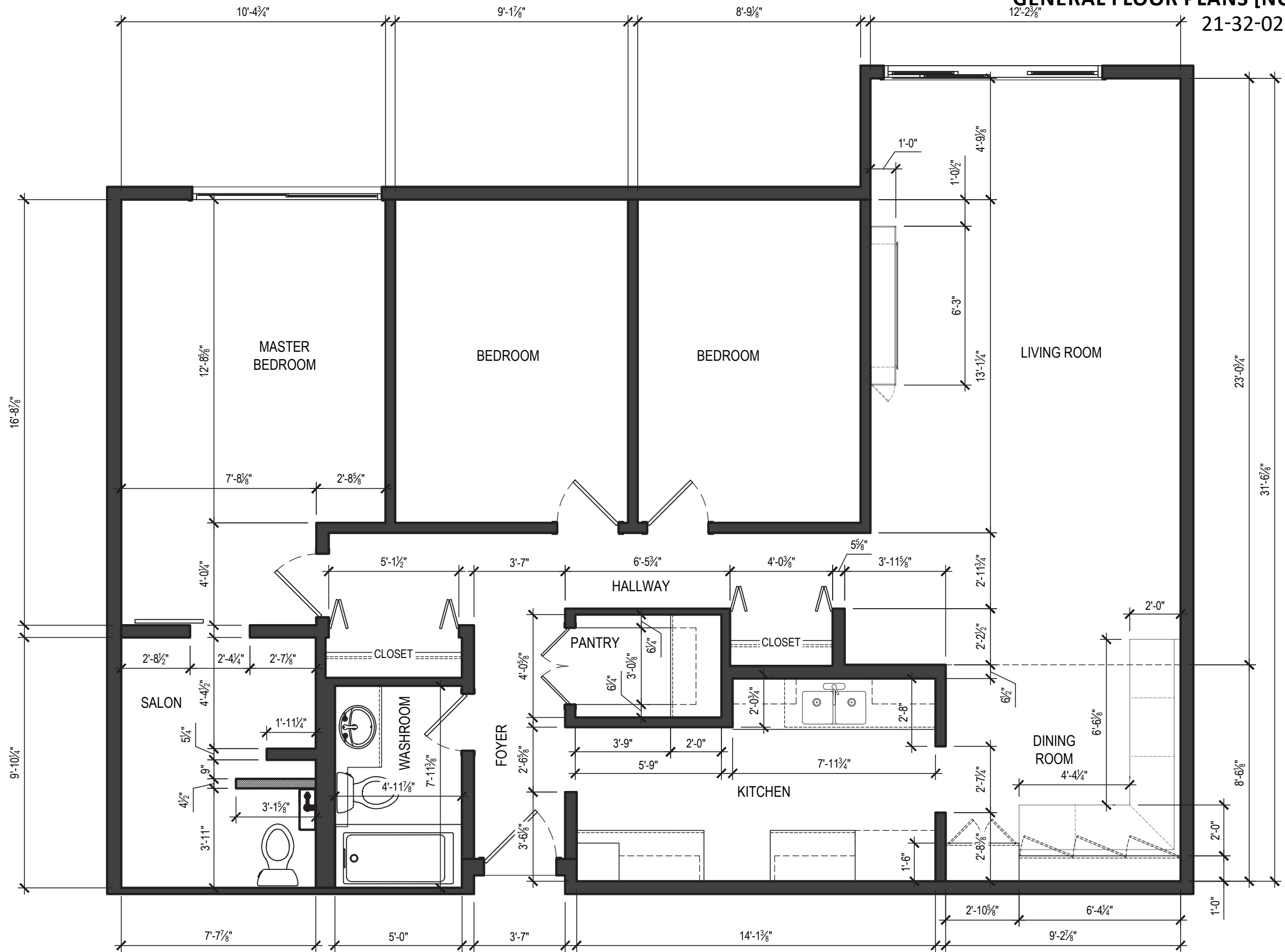
3 FLOOR PLAN (WITH DIMENSIONS) --- 1/4" = 1'-0"
